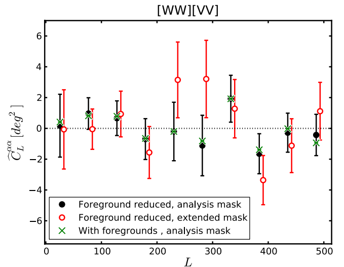
FIG. 7 (color online). Measurement of \hat{C}_L^{\alpha\alpha} from [WW][VV] cross-band correlation, with the corresponding statistical uncertainty obtained from a suite of null-hypothesis foreground-free simulations. Black filled circles are measurements obtained from the foreground-reduced maps after applying the fiducial analysis mask, and they represent our fiducial results of Fig. 3. The colored data points (and the associated error bars) correspond to the two test analyses: the green x 's are obtained from the maps prior to foreground subtraction, but using the fiducial mask, while the red empty circles are measurements obtained from foreground-reduced maps after applying an extended mask (with an additional \sim 35\% of the sky covered around the Galactic plane). The results from the two tests show no apparent bias. For the case of non-foreground-reduced analysis, the difference from the fiducial measurements is negligible compared to the statistical uncertainty; for the extended-mask case, the scatter between the two results is consistent with the difference in sky coverage. This implies that foregrounds and foreground residuals should not have a drastic impact on the estimated measurement uncertainty.
