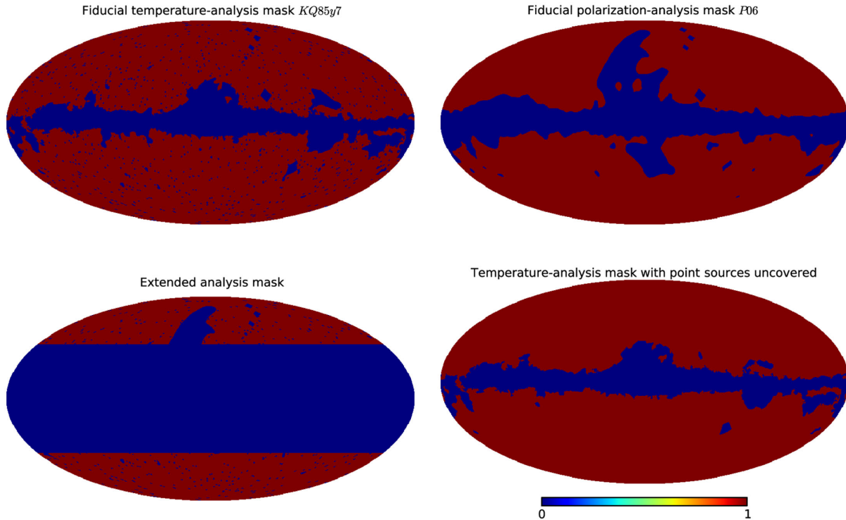
FIG. 12 (color online). Fiducial temperature-analysis mask (with \sim 78\% of the sky admitted), fiducial polarization-analysis mask ( \sim 73\% ), extended mask ( \sim 33\% ), and the temperature-analysis mask with point sources uncovered ( \sim 82\% ). Fraction of the sky admitted of the combined fiducial masks for polarization and temperature is \sim 68\% , which is twice the sky admitted as compared to the extended mask.
