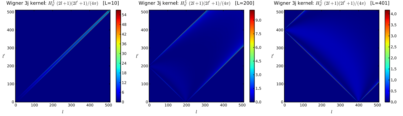
FIG. 9 (color online). The Wigner-3j geometric factors in the summands of Eqs. (8) and (16) for three different values of L . The geometric factor is nonzero only in the region of the ll' space where the triangle inequalities are satisfied. The dominant contribution comes from the triangles in which L \sim l , or L \sim l' , i.e., where either the temperature or the polarization mode has a length scale comparable to the length scale of the rotation-angle mode.
