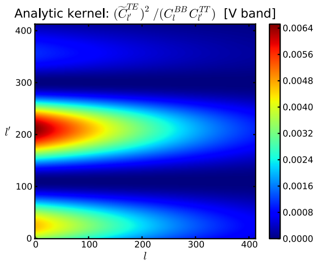
FIG. 10 (color online). The power-spectrum kernel of the summands in Eqs. (8) and (16). The types of triangles that contribute the most to the isotropic bias of C_L^{\hat{\alpha}\hat{\alpha}} are set by the geometric properties of spin-2 Wigner-3j symbols illustrated by the kernel shown in Fig. 9, which is modulated by this kernel to produce summands in the expression for the bias.
