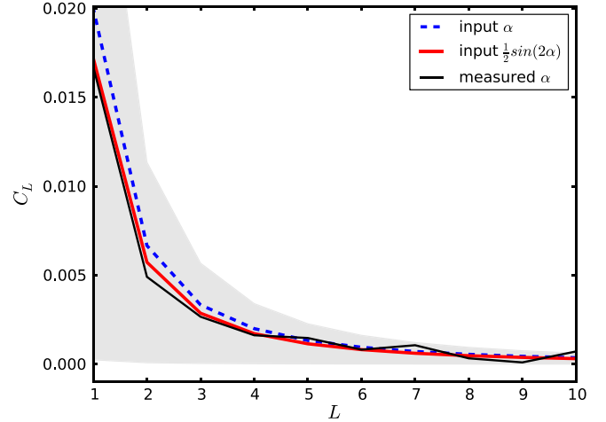
FIG. 1 (color online). The recovery of the CB signal with the analysis method presented in Sec. III is demonstrated using a suite of simulations that include realization of a rotated sky. The dashed blue line is the input signal power spectrum of C_L^{\alpha\alpha} , the thick red line represents the power spectrum of \frac{1}{2} \sin[2\alpha(\hat{\mathbf{n}})] , and the thin black line is the mean recovered power from the simulations; the gray region is a 1\sigma confidence-level interval calculated from the same suite of simulations.
