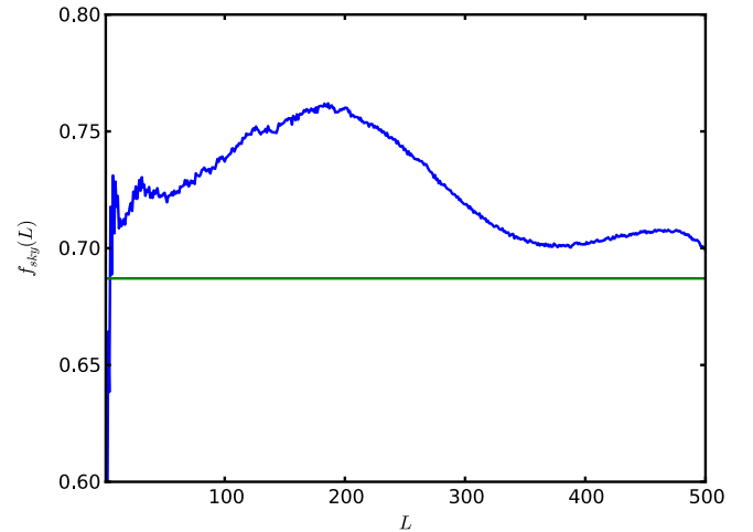
FIG. 11 (color online). The L dependence of the f_{\text{sky}} factor used for the reconstruction of the scale-invariant rotation-angle power spectrum in Secs. IV C and V B. The horizontal (green) line at f_{\text{sky}} = 0.68 represents the fraction of pixels admitted by the mask.
