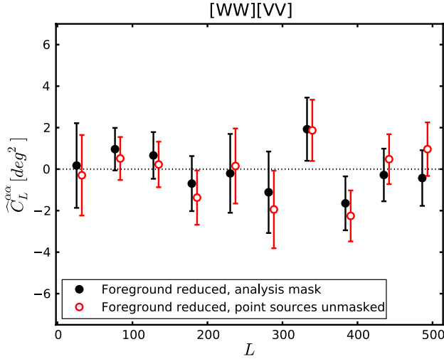
FIG. 6 (color online). Measurement of \hat{C}_L^{\alpha\alpha} from [WW][VV]. Results shown in black are obtained by using the analysis mask that covers all the point sources brighter than \sim 1 Jy, while the results in red (empty circles) are obtained after unmasking all the point sources. There is no apparent bias and the difference in every bin is less than the statistical uncertainty, despite the extreme variation in the source contamination. Scaling arguments in Sec. VC2 imply that the unresolved point sources have a negligible contribution to the estimated measurement uncertainty for the most constraining cross-band correlation.
