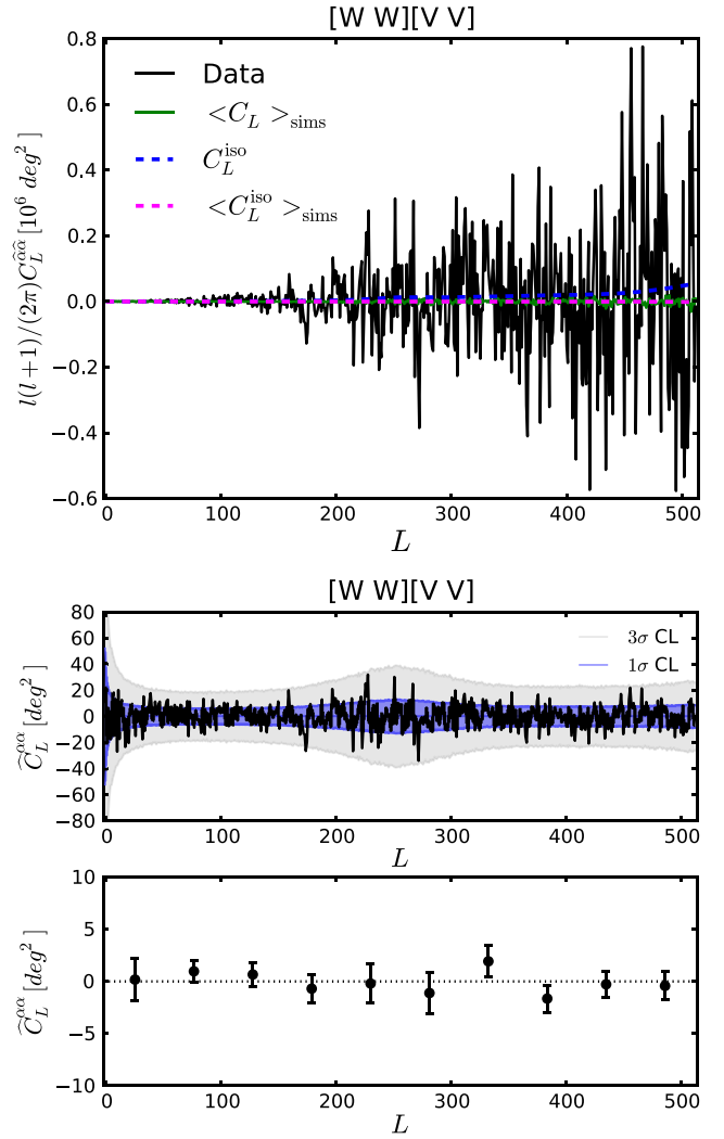
FIG. 3 (color online). Same as Fig. 2, for [f_1 f_2] \times [f_3 f_4] = [WW][VV] .
