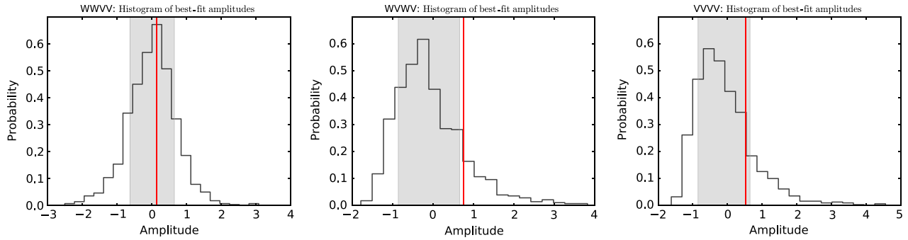
FIG. 5 (color online). Probability distributions of the best-fit amplitude \hat{A} of the scale-invariant rotation power C_L^{\alpha\alpha} recovered from a suite of null-hypothesis realizations are shown for some of the cross-band correlations. The gray areas denote a 68% confidence interval around a mean value; the red vertical line represents the measurement of the best-fit \hat{A} for a given cross-band correlation. We find consistency with zero within 3\sigma for all five measurements.
