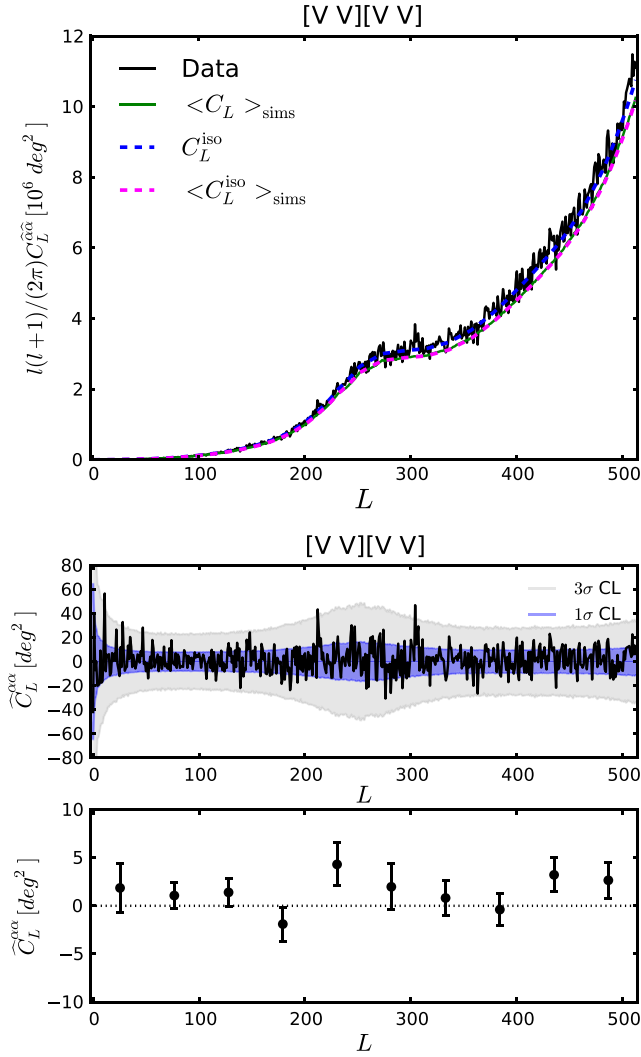
FIG. 2 (color online). Top panel: Measurement of the rotation-angle power spectrum from V band, shown before debiasing, along with the components of the noise bias: Monte Carlo measurement of the null-hypothesis mean \langle \hat{C}_L^{\alpha\alpha} \rangle , isotropic noise bias, and the mean isotropic bias. Middle panel: The same power spectrum after debiasing, with 1\sigma and 3\sigma confidence interval. Bottom panel: Binned version of the middle-panel power spectrum. The results are consistent with zero within 3\sigma .
