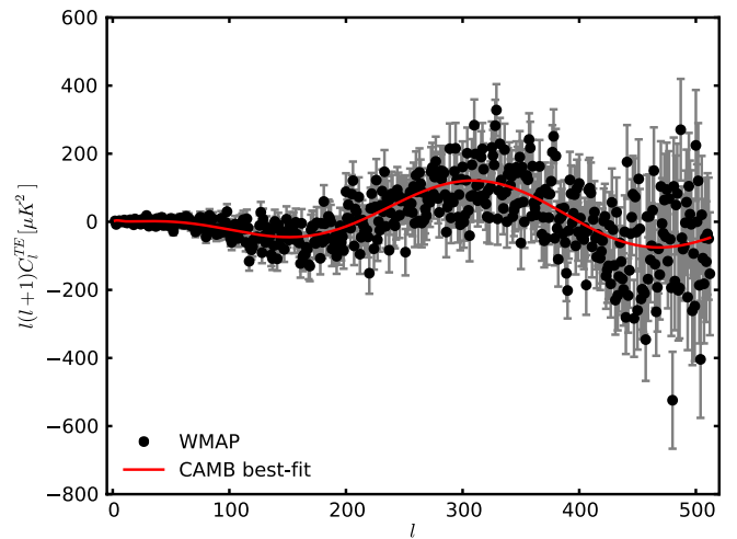
FIG. 8 (color online). TE correlation measured from WMAP-7 data (black) is compared to the primordial power spectrum, generated using CAMB for the best-fit cosmology with no rotation (red, solid); both power spectra are obtained from Ref. [23]. The uncertainty on this measurement (gray) leaves room for a maximal rotation-angle RMS of roughly 9.5^\circ .
