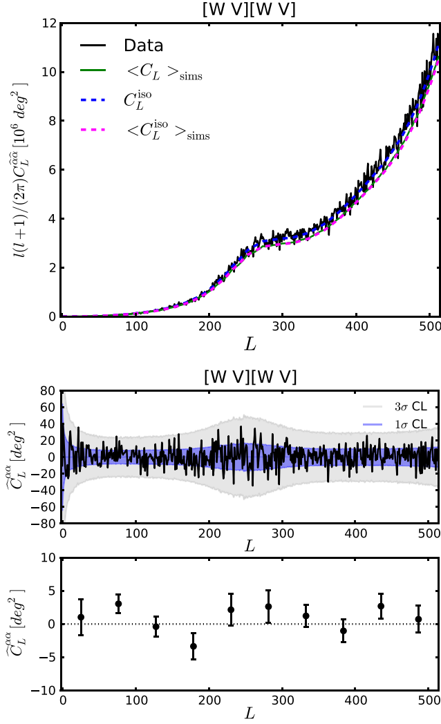
FIG. 4 (color online). Same as Figure 2, for [f_1 f_2][f_3 f_4] = [WV][WV] .
