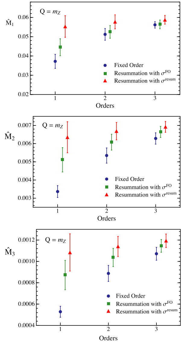
FIG. 2 (color online). Theoretical prediction for the first three moments at the Z pole at various orders in perturbation theory. The blue circles correspond to fixed order perturbation theory (normalized with the total hadronic cross section) at \mathcal{O}(\alpha_s) , \mathcal{O}(\alpha_s^2) and \mathcal{O}(\alpha_s^3) , green squares correspond to resummed predictions at NLL, NNLL, and N 3 LL normalized with the total hadronic cross section, and red triangles correspond to resummation normalized with the norm of the resummed distribution. For these plots we use \alpha_s(m_Z) = 0.114 .
