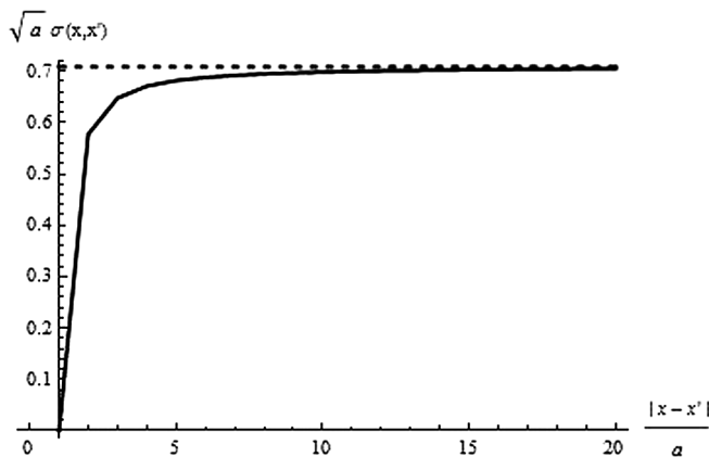
FIG. 1. \sqrt{a}\sigma(x, x') is plotted as a function of Euclidean distance scaled by lattice length.
