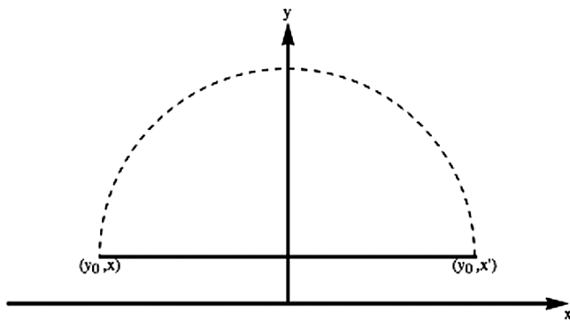
FIG. 4. The trajectory in the xy plane is shown by dotted line.
