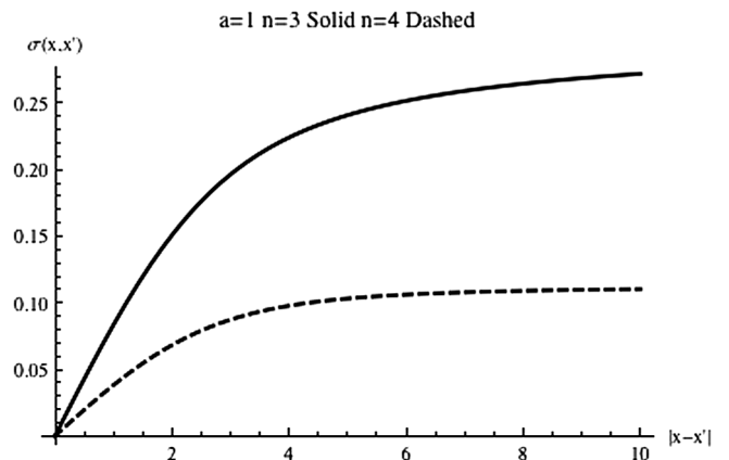
FIG. 2. This plot shows the dependence of \sigma with Euclidean distance in dimensions three and four.
