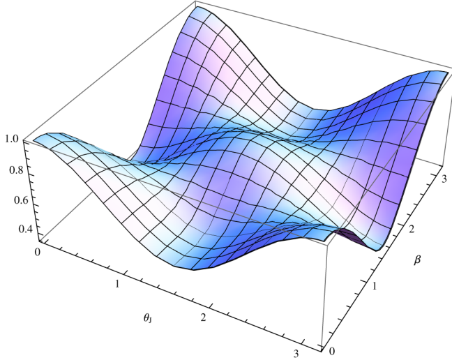
FIG. 10 (color online). Amplitude ratio model: For spinning precessing binaries, the function s(\theta_j, \beta, \psi_j = 0) describing the average amplitude along a given line of sight, assuming a steadily precessing binary with precession cone opening angle \beta . The function s(\theta_j, \beta, \psi_j) [Eq. (31)] is approximately the ratio \rho/\rho_{ns} between the amplitude \rho of a spinning, precessing binary seen in band in a configuration and line of sight specified by (\theta_j, \beta, \psi_j) and the amplitude \rho_{ns} of a nonspinning binary of comparable masses.
