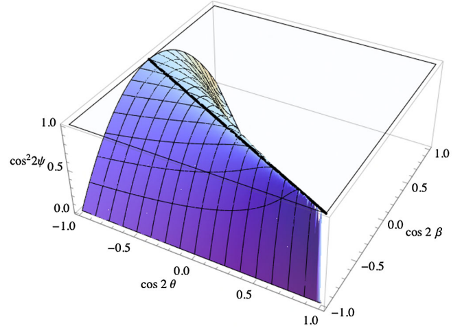
FIG. 7 (color online). Region divisions in coordinate form: The three ways the binary's orbital angular momentum can wind around the two null lines are separated by cases where the cone is tangent to one or the other axis. In this figure we express this dividing surface using explicit coordinates for the 3d configuration space: z = \cos^2 2\psi_J , x = \cos 2\theta_J , y = \cos 2\beta . Points on this surface are simultaneous solutions to Eq. (12), as calculated by Eq. (15). In this figure, the R1 region is the largest, farthest from the viewer; the region R3 is the region above the surface, closest to the viewer; and the region R2 is below the surface.
