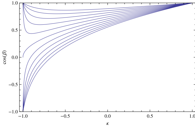
FIG. 2 (color online). Precession opening angle versus spin-orbit misalignment: Relation between \kappa = L \cdot S and \beta = \cos^{-1} L \cdot J for \gamma = |S|/|L| = 0.5, 0.6 \dots 1.5 . Binaries that are angular momentum dominated ( \gamma < 1 ) can have only a small range of precession cone opening angles, bounded by \beta_{\max} = \cos^{-1} \sqrt{1 - \gamma^2} . Binaries that are spin dominated ( \gamma > 1 ) can have all possible precession cone opening angles. For extremely spin dominated binaries \kappa = \cos \beta .
