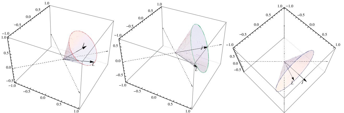
FIG. 6 (color online). Three regions have three types of precession cones: Shown is the precession cone for three fiducial binaries, characterized by the angles (\theta_J, \beta, \psi_J) = (\pi/4, \pi/6, 0) , (\pi/2, \pi/4, \pi/4) , and (\pi/2, \pi/3, 0) . Each figure shows the precession-induced path of \hat{L}(t) (colored circles), the total angular momentum direction (arrow), and an example of an instantaneous L direction (arrow). As these three examples demonstrate, each region corresponds to a different way the precession cone wraps around the two dotted lines. These two lines correspond to orientations of \hat{L} such that the detector would instantaneously see exactly zero amplitude. We will henceforth denote them as “null lines.” These three precession cones are representative examples of the three regions discussed in the text: R1 (left panel), R2 (middle panel), and R3 (right panel)
