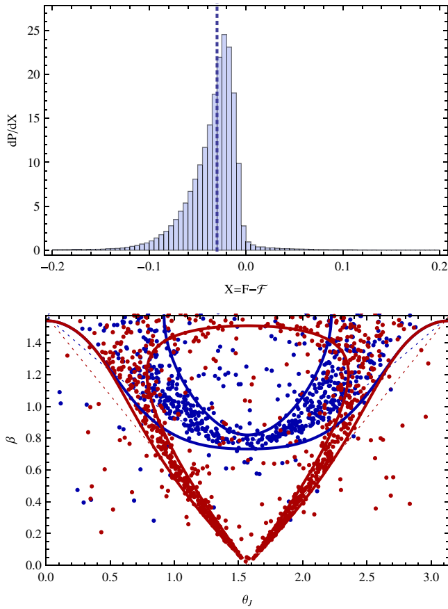
FIG. 13 (color online). Comparison of the analytic prediction of Sec. V C with numerical results II: Monte Carlo. As Fig. 12, except (a) the injected signal can have generic BH-NS-like masses m_1 \in [3, 15]M_\odot , m_2 \in [1, 5]M_\odot , dimensionless spin magnitudes \chi \in [0, 1] , and spin-orbit misalignments \hat{L} \cdot \hat{S} > -0.9 ; (b) to better recover aligned-spin signals, the template family includes Taylor F2 waveforms with \eta > 1/4 , spaced in chirp mass and \eta according to the 2PN hexagonal template bank. Top panel: Our match prediction works for generic sources. [Because the mass and spin distribution used in this analysis favors low \gamma and thus binaries nearly aligned in band, this distribution partially reflects our ability to recover nearly aligned-spin binaries with an extended \eta Taylor F2 bank. That said, subsets of the sample bounded below in \gamma also demonstrate our prediction works well for generic binaries with significant in-band misalignment. Bottom panel: Our expression identifies the dominant physical mechanisms that produce a poor fit between a spinning binary and a candidate nonprecessing waveform. Like Fig. 12, the dotted lines show the separatrixes between regions. The solid lines show the contours predicted from our expression for \mathcal{F} = 0.75 and \psi = 0 (blue) or \psi = \pi/4 (red). For comparison, the points indicate all signal versus bank fitting factors F < 0.66 for \cos 4\psi > 0.975 (blue) or F < 0.7 for \cos 4\psi < -0.975 .
