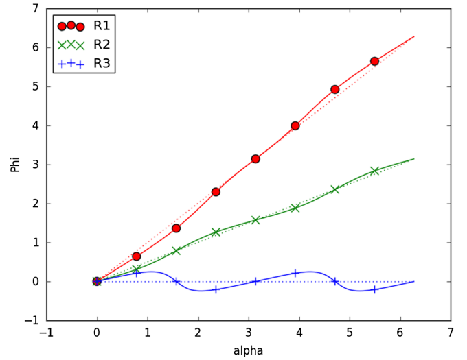
FIG. 8 (color online). Phase evolution versus time: For three selected viewing geometries of a single binary with \beta = 60^\circ , a plot of \Phi - \Phi_S(t) = \arg(z) versus \alpha , the precession phase. This plot shows how much of the precession phase is accumulated in the gravitational-wave signal due to precession [Eq. (21)]. These three phase evolutions are generated from Eqs. (17). The dotted line corresponds to W\alpha , where W corresponds to the rate of secular phase increase appropriate to that line of sight. The three viewing geometries lie in the three regions R1, R2, R3 described in the text.
