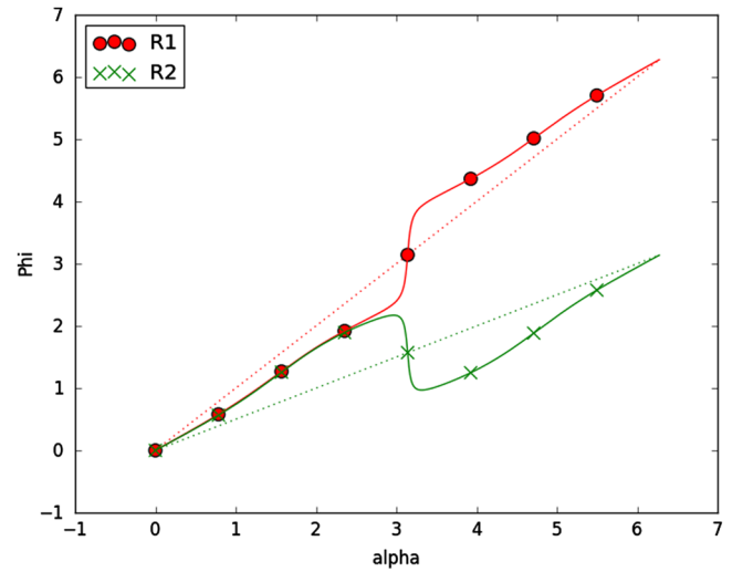
FIG. 14 (color online). Discrete phase change: With a fixed viewing geometry, the geometrical phase difference \arg(z) on either side of a transition surface (here, R1 to R2). As in Fig. 8, an entire precession cycle is shown.
