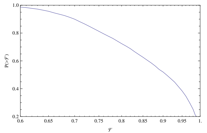
FIG. 11 (color online). Distribution of fitting factors for single-spin BH-NS: Using only the analytic expressions provided in this paper, the predicted fraction P(>\mathcal{F}) of fitting factors greater than \mathcal{F} for a randomly oriented BH-NS binary with m_1 = 10M_\odot , m_2 = 1.4M_\odot , with the dimensionless black hole spin \vec{\chi}_1 randomly oriented and with magnitude uniformly distributed between 0 and 0.98. Compare to the solid line in the bottom right panel of Fig. 9 in Ref. [31], although there the neutron star also has a spin up to 0.3.
