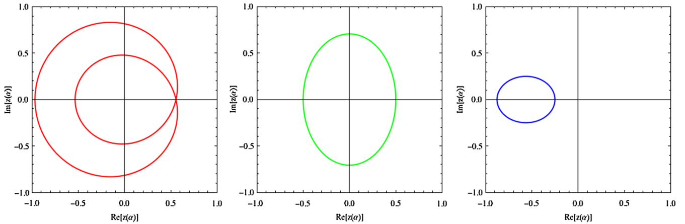
FIG. 9 (color online). Complex amplitude contours: Three examples of the complex amplitude z(\alpha) over a precession cycle, in the constant precession cone approximation. The three configurations shown correspond to the three fiducial precession cones shown in Fig. 6.
