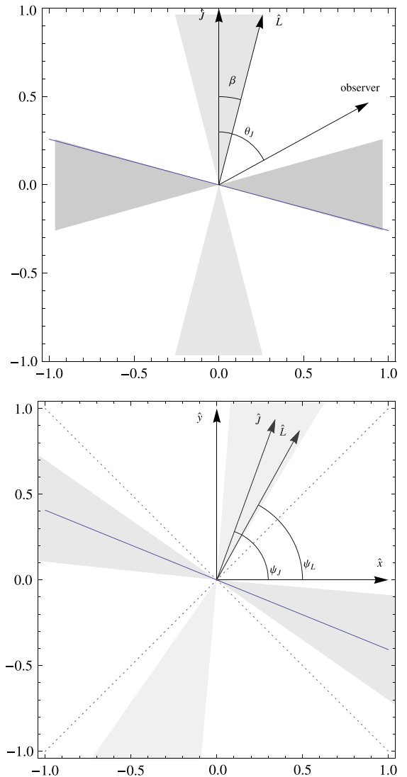
FIG. 5 (color online). Coordinates for steady precession: View from the side (top panel) and along the line of sight (bottom panel) of the geometry of a typical precessing BH-NS orbit, on time scales t long compared with precession but short compared to gravitational-wave decay ( \Omega_p t \gg 1 \gg t/\tau_{gw} ). The light shaded region indicates the cone swept out around the axis by the orbital angular momentum (the direction of strong, circularly polarized gravitational-wave emission from each orbit). In both panels, the thin diagonal line indicates a direction perpendicular to \hat{L} . The dark shaded region indicates the corresponding region swept out by the orbital plane (the direction of weakest, linearly polarized emission); observers along these lines of sight see strong amplitude modulation. The angle \beta between the total angular momentum \vec{J} and \vec{L} is nearly constant on precession time scales. On longer time scales, as \beta increases, the line of sight to the observer is often enclosed in one of the two shaded regions. On the bottom panel, the \hat{x} and \hat{y} axes correspond to the arms of the detector, projected into the plane of the sky. The dotted lines correspond to “null lines,” the directions that, when \hat{L} is parallel to them, produce zero amplitude in our detector; these lines lie in the plane of the sky, perpendicular to our line of sight. (To distinguish \vec{J} and \vec{L} in the plane of the sky, the two panels adopt different reference times.)
