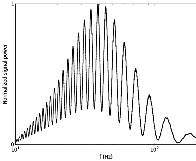
FIG. 4. Several precession cycles contribute comparably to the signal: Power ( |\tilde{h}_\times|^2/S_h(f) ) versus frequency for a spinning binary viewed edge on the \times polarization, computed directly from a Fourier transform of the gravitational-wave signal. In this figure, the binary is a 10 + 1.4M_\odot BH-NS binary with \chi_1 = 1 and \beta^* \approx \pi/3 (solid line). Each pair of peaks corresponds to a single precession cycle. The signal is divided by the high-power zero-detune advanced LIGO noise power spectral density [41].
