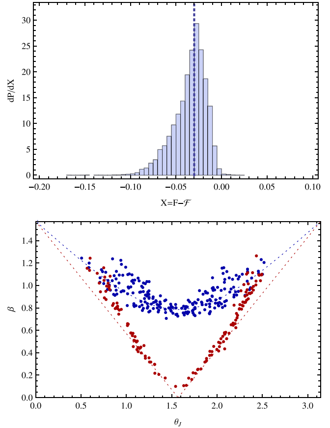
FIG. 12 (color online). Comparison of the analytic prediction of Sec. VC with numerical results I: Single binary masses and spin magnitude Top panel: For 30 000 BH-NS binaries ( 10M_{\odot} + 1.4M_{\odot} with a_1 \in [0, 1] ) with random orientations for \hat{L} \cdot \hat{S} > -1/2 , a comparison between our estimate \mathcal{F} and the fitting factor F calculated by comparing that signal with a standard single-detector template family (Taylor F2 templates with physical parameters; hexagonal template bank chosen for 97% minimal match; early-stage advanced LIGO noise curve such that f_{\text{peak}} \approx 40 Hz [41]). For comparison, the vertical dotted line at -0.03 shows the typical mismatch expected from template bank discreteness. Despite known systematic differences between the signal and template model even for aligned systems, our match prediction works well almost everywhere. To highlight its effectiveness, we have eliminated the small fraction of worst-performing configurations, corresponding to sources recovered with templates with 0.24 < \eta \leq 1/4 . Because of the finite parameter extent of physical Taylor F2 templates, the conventional signal model cannot reproduce large aligned spins. Bottom panel: For the same comparison of template bank against signals as above, the configurations of the worst-fit sources ( F < 0.7 ) with \cos 4\psi > 0.9 (black or blue; J nearly aligned with the detector on the plane of the sky) and \cos 4\psi < -0.9 (dark gray or red; J nearly 45^\circ off the detector arms, in the plane of the sky). For comparison, the black or blue and dark gray or red solid lines are the surfaces \cos 2\beta + \cos^2 \theta = 0 (black or blue) and \cos 2\theta_j + 2 \cos 2\beta (dark gray or red) [Eq. (16)]. These lines are two one-dimensional cuts through the surface separating R1 and R2, where our expression predicts the worst single-detector matches will occur.
