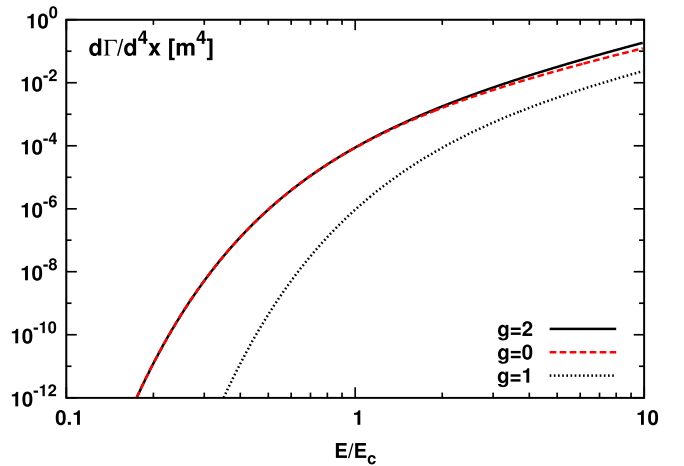
FIG. 1 (color online). The rate per unit volume of decay of the field d\Gamma/d^4x = 2\text{Im}V_{\text{eff}} with \text{Im}V_{\text{eff}} given by Eq. (14). The electric field magnitude is normalized to \mathcal{E}_c = m^2/e the critical field strength, at which T_M \rightarrow m/\pi . For g \neq 2 the rate of field decay is reduced with the largest reduction for g = 1 . Above \mathcal{E}_c we see suppression due to the g factor modifying weights in the sum in Eq. (14).
