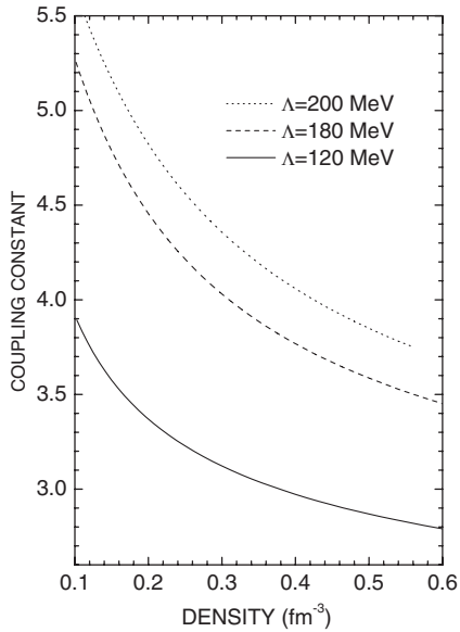
FIG. 2. The running coupling constant g versus the baryon number density at different \Lambda values with the magnetic field B_m = 10^{17} G. The upper lines correspond to larger values of \Lambda .
