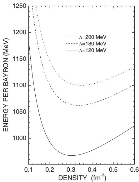
FIG. 3. The energy per baryon E/n_B of stable MSQM versus the number density at different \Lambda values with the corresponding critical magnetic field strength B_m^c .
