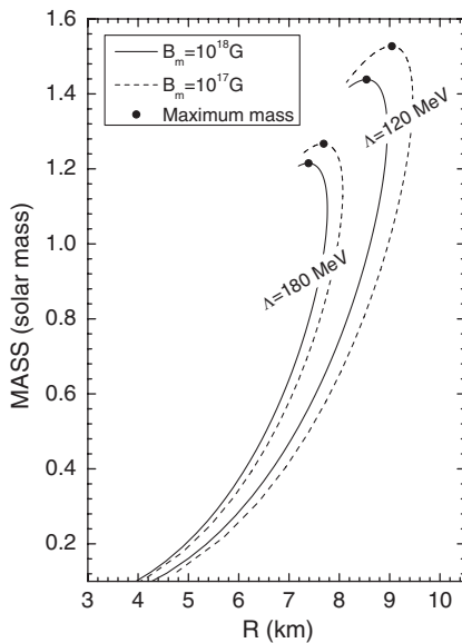
FIG. 7. The mass-radius relation of SQS at different \Lambda values with different magnetic fields B_m = 10^{17} G (dashed lines) and B_m = 10^{18} G (solid lines). The maximum masses on all curves are marked by full dots.
