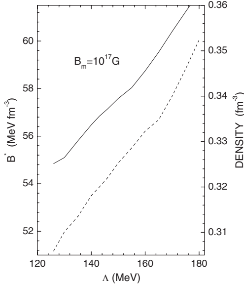
FIG. 6. \Lambda dependence of the bag function B^* (solid line) and baryon number density (dashed line) corresponding to the zero pressure. The \Lambda should be larger than the critical value 126 MeV to produce a nonmonotonic behavior of B^* .
