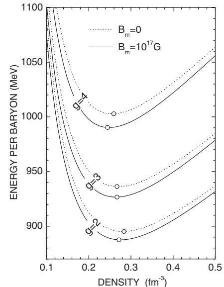
FIG. 1. The energy per baryon versus the density at fixed coupling constant g = 2, 3, 4 for magnetic field strength B_m = 10^{17} G. Compared with the nonmagnetized strange quark matter (the dotted curves with B_m = 0 ), the magnetized case has a lower energy per baryon.
