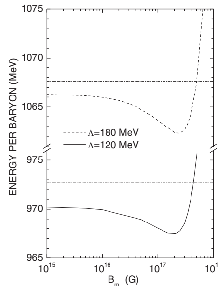
FIG. 4. The energy of magnetized strange quark matter varies with the magnitude of the strong magnetic field for the fixed QCD scale parameter \Lambda = 180 MeV (the upper dashed curve) and \Lambda = 120 MeV (the lower solid curve), respectively. With decreasing the magnetic field strength, the energy per baryon approaches gradually to the value without a magnetic field indicated by a horizontal dashed-dotted line.
