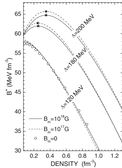
FIG. 5. The effective bag function B^* for MSQM versus the baryon number density at different \Lambda values. B_m = 10^{17} G and B_m = 10^{18} G are marked by dashed lines and solid lines, respectively. Only for larger \Lambda , the B^* has a maximum value B_{\text{max}}^* indicated by asterisks at 2–3 times nuclear saturation density.
