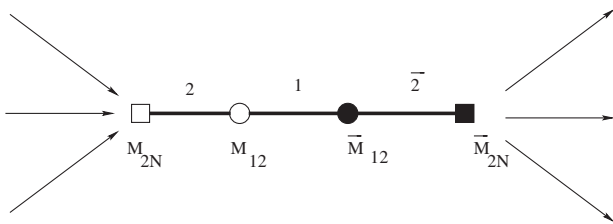
FIG. 2. Example of the dipole meson formed as result of breaking of 2-nd string by pair creation of monopole M_{2N} (shown by boxes) interpolating between 2-nd string and would-be N -th string, which is absent. Arrows denote unconfined flux. Circles denote monopoles M_{KK'} , K, K' = 1, \dots, \nu . Open and closed circles/boxes denote monopoles and antimonopoles, respectively.
