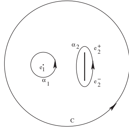
FIG. 4. \alpha -contours in x -plane for the U(2) theory. Solid straight line denotes the cut.
