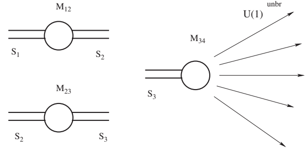
FIG. 3. The monopole confinement in the r = 3 vacuum. The thick double lines denote strings, while the circles denote monopoles. Unconfined U(1) flux is shown by arrows.
