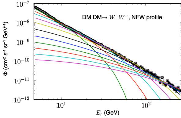
FIG. 16 (color online). Measured intensity (black) and largest allowed intensity (various colors) for WIMP annihilation to W^+W^- for WIMP masses 86, 139, 224, 360, 578, 923, 1495, 2405, 3867, 6219, and 10000 GeV, for the region |b| > 10^\circ plus a 20^\circ \times 20^\circ square at the GC.
