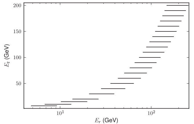
FIG. 9. Spectral line search energy ranges.
