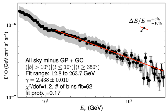
FIG. 8 (color online). E^2 \times \Phi with power-law fit. The gray band shows the systematic error due to uncertainty in the effective area. The arrow shows the shift due to uncertainty in the absolute energy scale. The intensities and energies shown here are tabulated in Table I.
