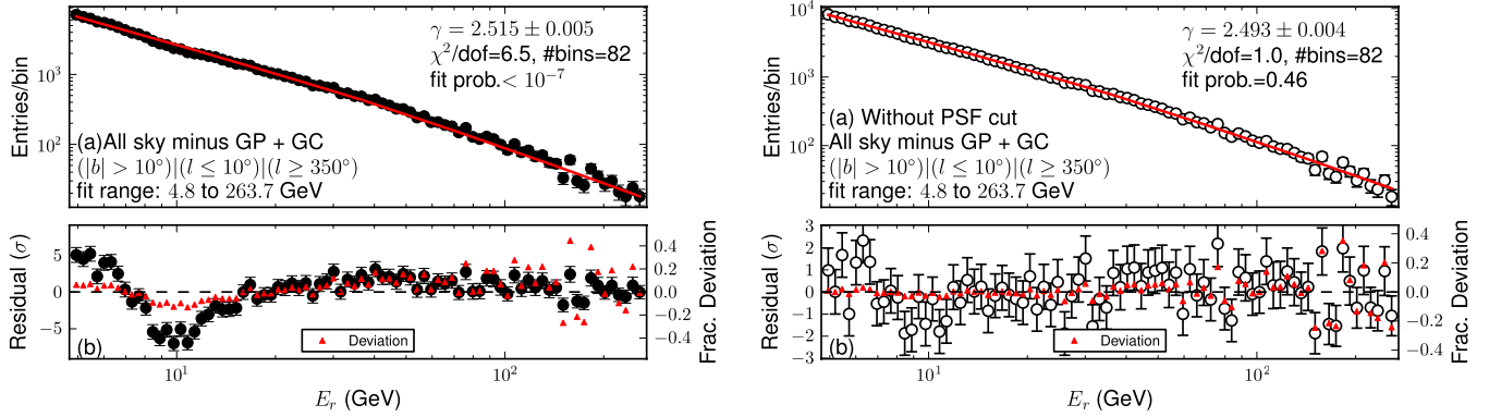
FIG. 7 (color online). The inclusive photon counts spectrum (circles) of the expected signal region. The left spectrum includes photons from the Pass 6 DATACLEAN sample, while the right spectra also includes those photons which failed to pass the “PSF cut,” which induces systematic effects below \sim 13 GeV, as shown in Fig. 6 with control data sets. A power-law fit (top, line), normalized fit residuals (bottom, circles), and the fractional deviation of the data from the power-law fit (bottom, small triangles) are shown as in Fig. 6. We search for dark matter induced gamma-ray lines above \sim 13 GeV using the left data set, and below \sim 13 GeV using the right data set. For dark matter contributions to the inclusive spectrum, we use the left spectrum (for which the systematics from the PSF cut are not important)—see Sec. IV B.
