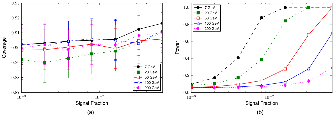
FIG. 10 (color online). Coverage (a) and power (b) for 5000 MC trials for 7, 20, 50, 100, and 200 GeV spectral lines. The error bars are statistical. The background is simulated by a power-law with index \Gamma = 2.5 . In coverage plots, f_j is not restricted to be greater than zero. Restricting to f_j > 0 results in over-coverage at low signal fraction.
