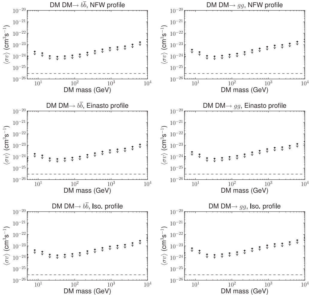
FIG. 17. Cross-section upper limits for dark matter annihilation to b -quarks or gluons from the diffuse gamma-ray background spectrum for the region |b| > 10^\circ plus a 20^\circ \times 20^\circ at the GC, assuming the NFW, Einasto, or isothermal dark matter halo profiles. No photons from astrophysical background sources have been included, making these limits very conservative. The horizontal dashed line is the cross section for a thermally produced WIMP ( 3 \times 10^{-26} \text{ cm}^3 \text{ s}^{-1} ).
