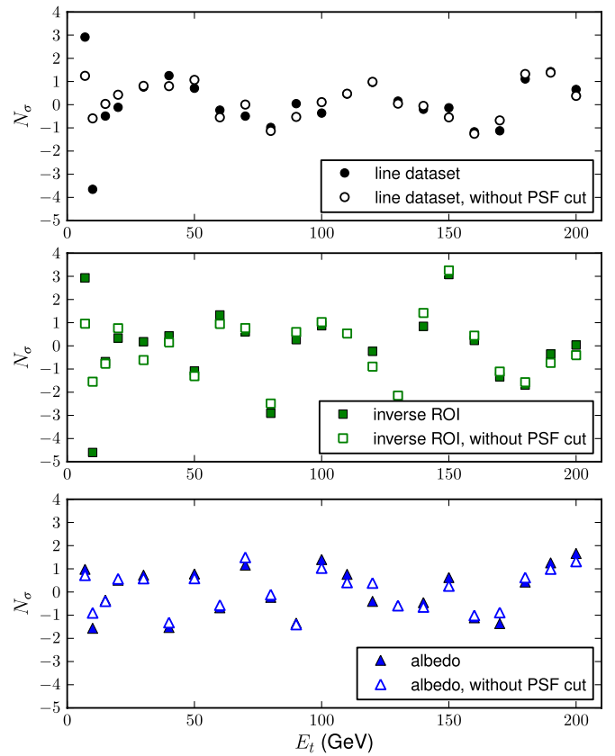
FIG. 12 (color online). Signal significance for the line, inverse ROI, and albedo data sets with and without the PSF cut. A trial factor is not applied to the signal significance. All data sets show an excess at 7 GeV and a deficit at 10 GeV. In the line data set and inverse ROI data sets, the 7 and 10 GeV features have magnitude of significance \geq 3\sigma . Removing the PSF cut decreases the magnitude of their significance, particularly in the line dataset and inverse ROI.
