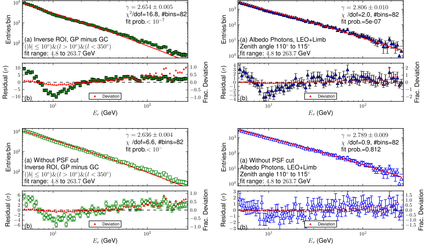
FIG. 6 (color online). The photon counts spectrum for the inverse ROI ( |b| < 10^\circ excluding the 20^\circ \times 20^\circ square at the GC) (solid squares for left top, open squares for left bottom) and for an albedo photon data set (solid triangles for right top, open triangles for right bottom). The top two plots show photons from the “Pass 6 DATA CLEAN” class (see Sec. II), while the bottom two plots in addition include photons that fail to pass the “PSF cut,” which was designed to improve the LAT PSF. In each subfigure, the top plot (a) shows (with a solid line) a fit of the data to a power-law function F(E, \gamma) = E^{-\gamma} times the appropriate exposure \varepsilon(E) (see text); the bottom plot (b) shows the normalized fit residuals and fractional deviation (small triangles) of the data from the fit curve. The top panel shows a prominent bump and dip below about \sim 13 GeV, which is mitigated by removing the PSF cut in the bottom panel, indicating that these features are systematic effects. Note that the vertical scale of the residuals is different for the different panels. The errors bars on the entries/bin are \sqrt{\text{counts}} , while the errors bars on the residuals are \pm 1 sigma to guide the eye.
