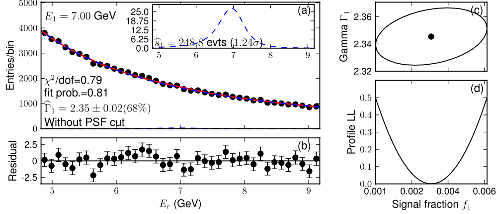
FIG. 13 (color online). Line data-set spectral line fitting results, excluding the PSF cut, for 7 GeV. Removing the PSF cut from the line data set reduces the signal significance from 2.9\sigma to 1.2\sigma , indicating that the feature is caused by a systematic effect. (a) Composite unbinned maximum likelihood fit (signal and background components in blue dashed, combined signal+background in solid red). Signal pdf shown in inset (blue dashed line). (b) Normalized residuals for the composite fit. (c) Standard error ( 1\sigma ) CL error ellipse. (d) Profile of the log-likelihood (LL) for the signal fraction, which is maximized with respect to the spectral index at each point. Note that there are two blue lines in the top left figure, one for the background, which is largely indistinguishable from the red line, and one for a small simulated signal, which is barely distinguishable from the x-axis in this plot, but also shown in the inset.
