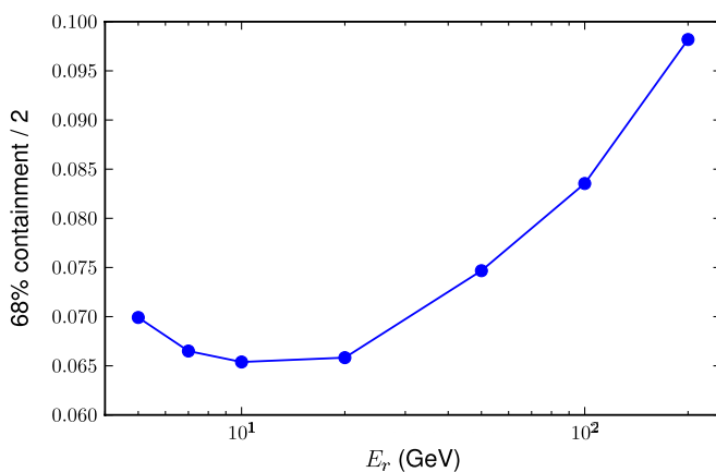
FIG. 4 (color online). MC-derived energy resolution (68% energy dispersion fractional containment divided by 2), integrated over the angular acceptance.
