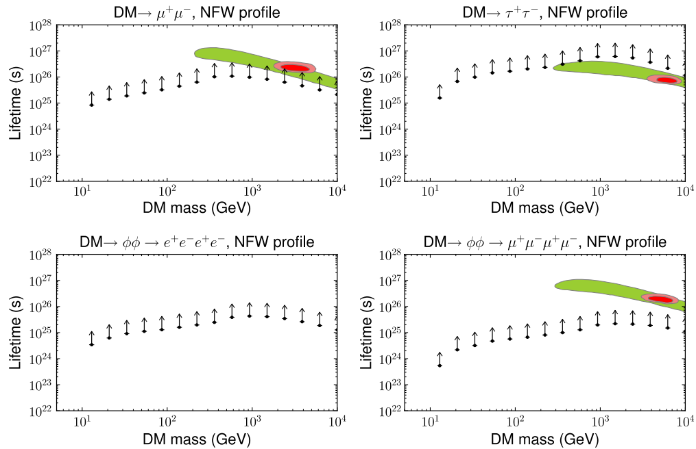
FIG. 22 (color online). As in Fig. 21 but now for dark matter decay to \mu^+\mu^- , \tau^+\tau^- , or \phi\phi , where \phi is a new low-mass force mediator with mass 0.1 GeV (1 GeV), and decays to e^+e^- ( \mu^+\mu^- ) in the figure on the left bottom (right bottom). The green and red shaded regions can explain the PAMELA and Fermi CR data, respectively. They are taken from [59], but we have rescaled their regions by 4/3 to a local density of \rho_\odot = 0.4 \text{ GeV cm}^{-3} from 0.3 \text{ GeV cm}^{-3} used in [59].
