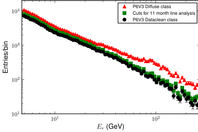
FIG. 2 (color online). Counts spectrum from 4.8 to 2604 GeV in 5% bins for photons in the Pass 6 DIFFUSE class (red triangles), the P6_V3 11-month line analysis photon class (green square), and the Pass 6 DATACLEAN class (black circles) for the ROI |b| > 10^\circ plus a 20^\circ \times 20^\circ square centered at the GC. The dataclean class has the tightest cuts. Additional cuts on the inclination, zenith, LAT rocking angles, and point sources from the LAT 1-year catalog are included.
