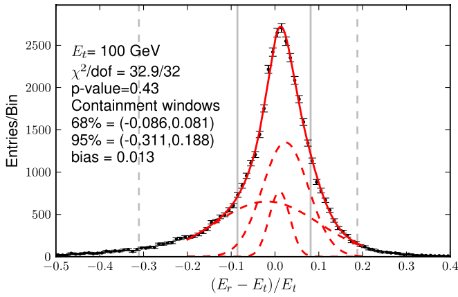
FIG. 3 (color online). Energy dispersion for the 100 GeV MC spectral line. The unbinned maximum likelihood best fit for G(x) is shown with its component Gaussian functions. The 68% and 95% containment windows are given by the solid and dashed vertical lines, respectively, and are based on G(x) . The \chi^2/\text{dof} and p -value for the binned data are included in the figure. The fit of G(x) to the MC data is cut off at |x| > 0.2 (see text).
