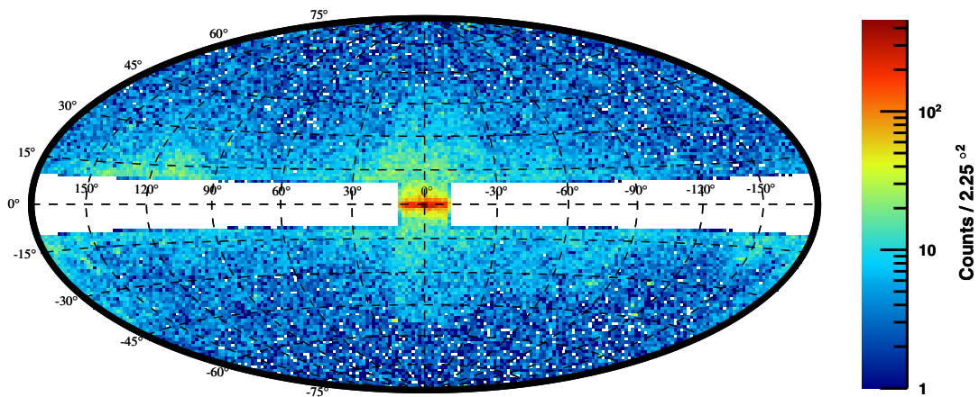
FIG. 1 (color online). The line data set binned in 1.5^\circ \times 1.5^\circ spatial bins, plotted in galactic coordinates using a Hammer-Aitoff projection. Photons with energy from 4.8 to 264 GeV are included. The white areas away from the Galactic plane correspond to the locations of 1FGL point sources and have been masked here. The area in white along the Galactic plane is excluded from this ROI.
