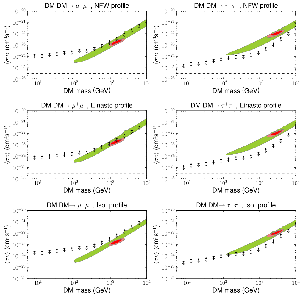
FIG. 19 (color online). As in Figs. 17 and 18, but for dark matter annihilation to \mu^+\mu^- or \tau^+\tau^- .
