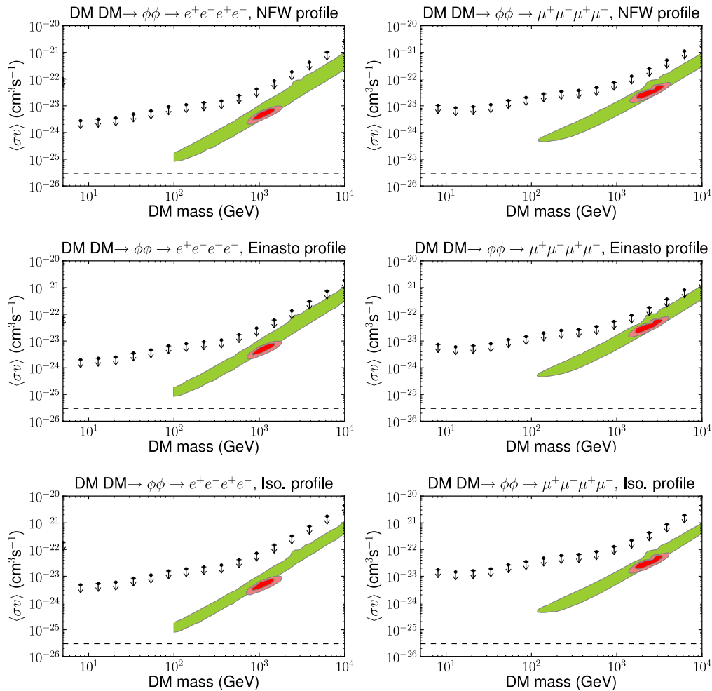
FIG. 20 (color online). As in Figs. 17 and 18, but for dark matter annihilation to \phi\phi , where \phi is a new low-mass force mediator with mass 0.1 \text{ GeV} ( 1 \text{ GeV} ), and decays to e^+e^- ( \mu^+\mu^- ) in the figures on the left (right).
