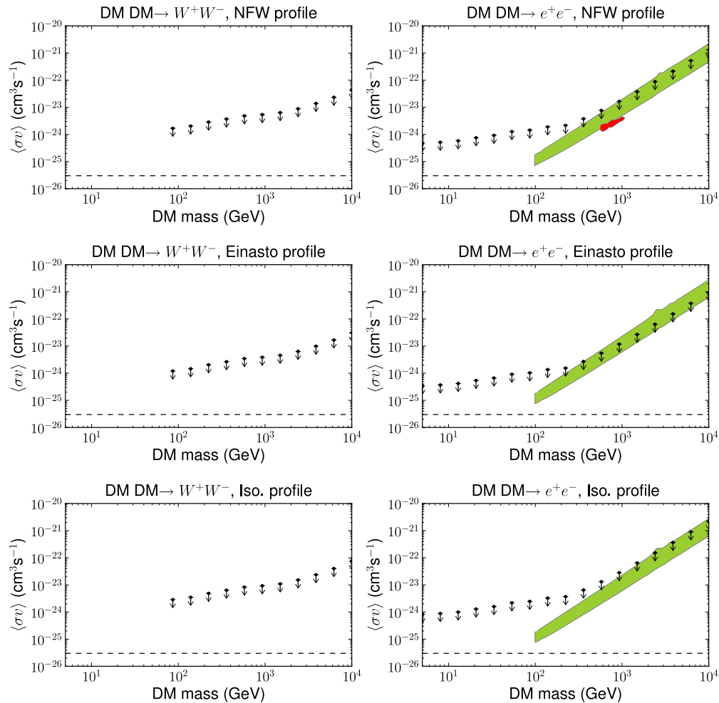
FIG. 18 (color online). As in Fig. 17, but for dark matter annihilation to W -bosons or e^+e^- . The annihilation to e^+e^- only includes prompt photons from final states radiation and none from high-energy leptons inverse Compton scattering off starlight or cosmic microwave background photons. The green and red shaded regions can explain the PAMELA and Fermi CR data, respectively. They are taken from [59], but we have rescaled their regions by (3/4)^2 to a local density of \rho_\odot = 0.4 \text{ GeV cm}^{-3} from 0.3 \text{ GeV cm}^{-3} used in [59].
