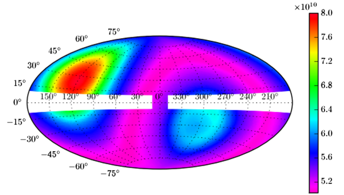
FIG. 5 (color online). Exposure map for 100 GeV in \text{cm}^2 \text{s} in Hammer-Aitoff projection, cut for the ROI |b| > 10^\circ plus a 20^\circ \times 20^\circ square centered at the GC. The map average and square root of the variance is (5.60 \pm 0.61) \times 10^{10} \text{ cm}^2 \text{s} . The exposure is calculated over the line data-set energy range at 5% intervals in log-space for use in the flux construction. The average exposure varies by only \sim 25\% over our energy range.
