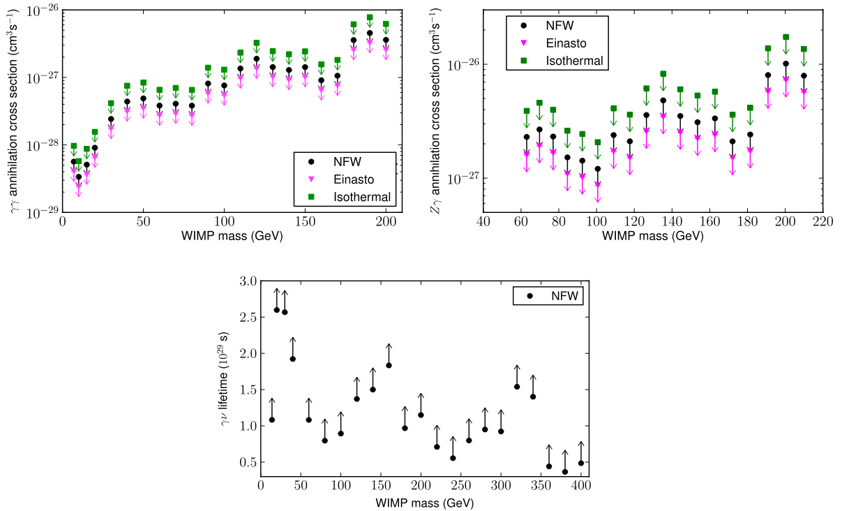
FIG. 15 (color online). Top row: Dark matter annihilation 95% CL cross-section upper limits into \gamma\gamma (left) and Z\gamma (right) for the NFW, Einasto, and isothermal profiles for the region |b| > 10^\circ plus a 20^\circ \times 20^\circ square at the GC. \gamma Z limits below E_\gamma < 30 GeV are not shown; see text for explanation. Bottom row: Dark matter decay 95% CL lifetime lower limits into \gamma\nu for the NFW profile and same ROI. Systematic effects from the photon line flux upper limits are not included.
