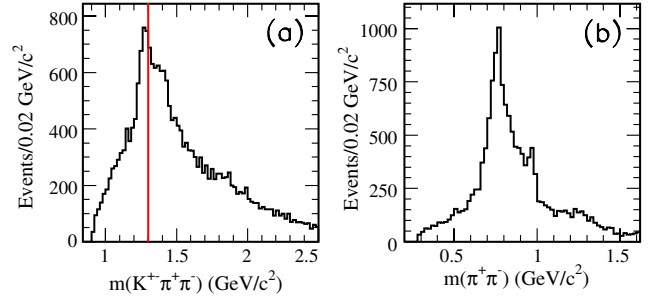
FIG. 7 (color online). (a) The invariant mass of the K^+\pi^+\pi^- combinations with K^*(892)^0K\pi events excluded; (b) the \pi^+\pi^- invariant mass for events from (a) with the K_1(1270) region suppressed by requiring m(K^+\pi^+\pi^-) > 1.3 \text{GeV}/c^2 as shown by vertical line in (a).
