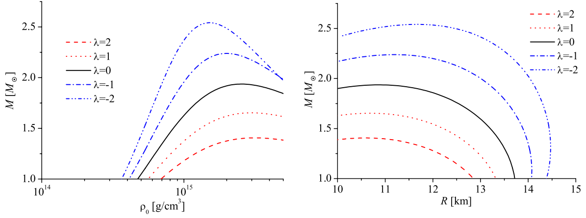
FIG. 3 (color online). The mass of the neutron stars as a function of the central density (left panel) and of the radius (right panel) for several values of the parameter \lambda .
