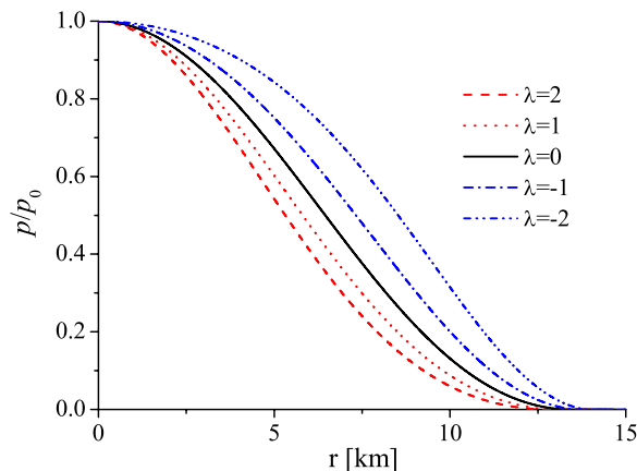
FIG. 2 (color online). The radial p and the anisotropic pressure \sigma as functions of the radial coordinate r , normalized to the value of the radial pressure at the center of the star p_0 . The results are for the same solutions as in Fig. 1.
