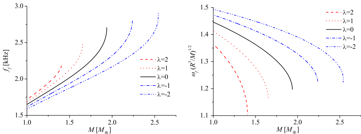
FIG. 5 (color online). The frequency f as a function of the mass M (left panel) and the normalized frequency \omega as a function of M (right panel) for the f mode. The results for several values of the parameter \lambda are shown.
