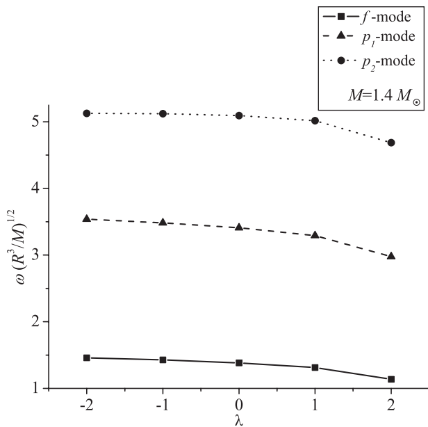
FIG. 7. The normalized frequency \omega as a function of \lambda for fixed value of the mass M = 1.4M_\odot . The results for the f , p_1 and p_2 modes are shown.
