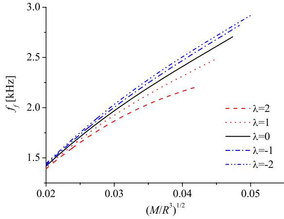
FIG. 4 (color online). The f -mode frequency as a function of the square root of the average density \sqrt{M/R^3} . The results for several values of the parameter \lambda are shown.
