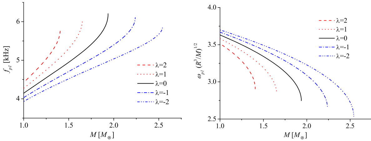
FIG. 6 (color online). The results for the p_1 mode of the same solutions as shown on Fig. 5.
