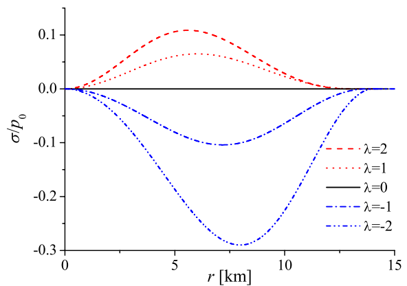
FIG. 2 (color online). The radial p and the anisotropic pressure \sigma as functions of the radial coordinate r , normalized to the value of the radial pressure at the center of the star p_0 . The results are for the same solutions as in Fig. 1.
