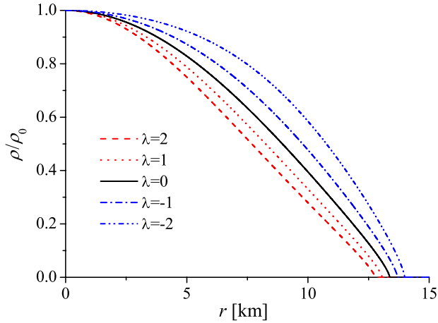
FIG. 1 (color online). The normalized energy density \rho as a function of the radial coordinate r . The results for several neutron star solutions with the same central energy density \rho_0 = 7.455 \times 10^{14} g/cm 3 and different values of the parameter \lambda are shown (this central energy density gives neutron star with mass M = 1.4M_\odot in the case with zero anisotropic pressure, i.e. when \lambda = 0 ).
