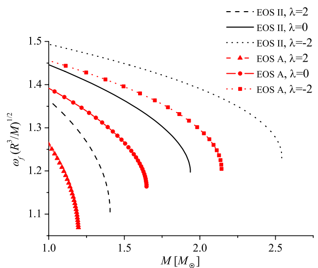
FIG. 8 (color online). The normalized frequency \omega as a function of M for the f mode. The results for different values of \lambda and for two polytropic equations of state of the radial pressure are shown—a soft equation of state EOS A and a stiff equation of state EOS II.
