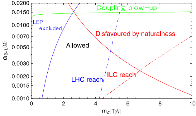
FIG. 1 (color online). The allowed parameter region is drawn [4]. The upper region of the almost straight line (in green) is rejected by a requirement that the B - L gauge coupling does not diverge up to the Planck scale. The upper-right side of the solid line (in red) is disfavored by the naturalness condition of the electroweak scale. The left of the solid line (in blue) has been already excluded by the LEP experiment, v_{B-L} \gtrsim 3 TeV. Recent LHC results for Z' boson search excluded the region m_{Z'} \lesssim 1.5 TeV [10]. The left of the dashed line can be explored in 5\text{-}\sigma significance at the LHC with \sqrt{s} = 14 TeV and an integrated luminosity 100 \text{ fb}^{-1} . The left of the dotted line can be explored at the International Linear Collider (ILC) with \sqrt{s} = 1 TeV, assuming 1% accuracy.
