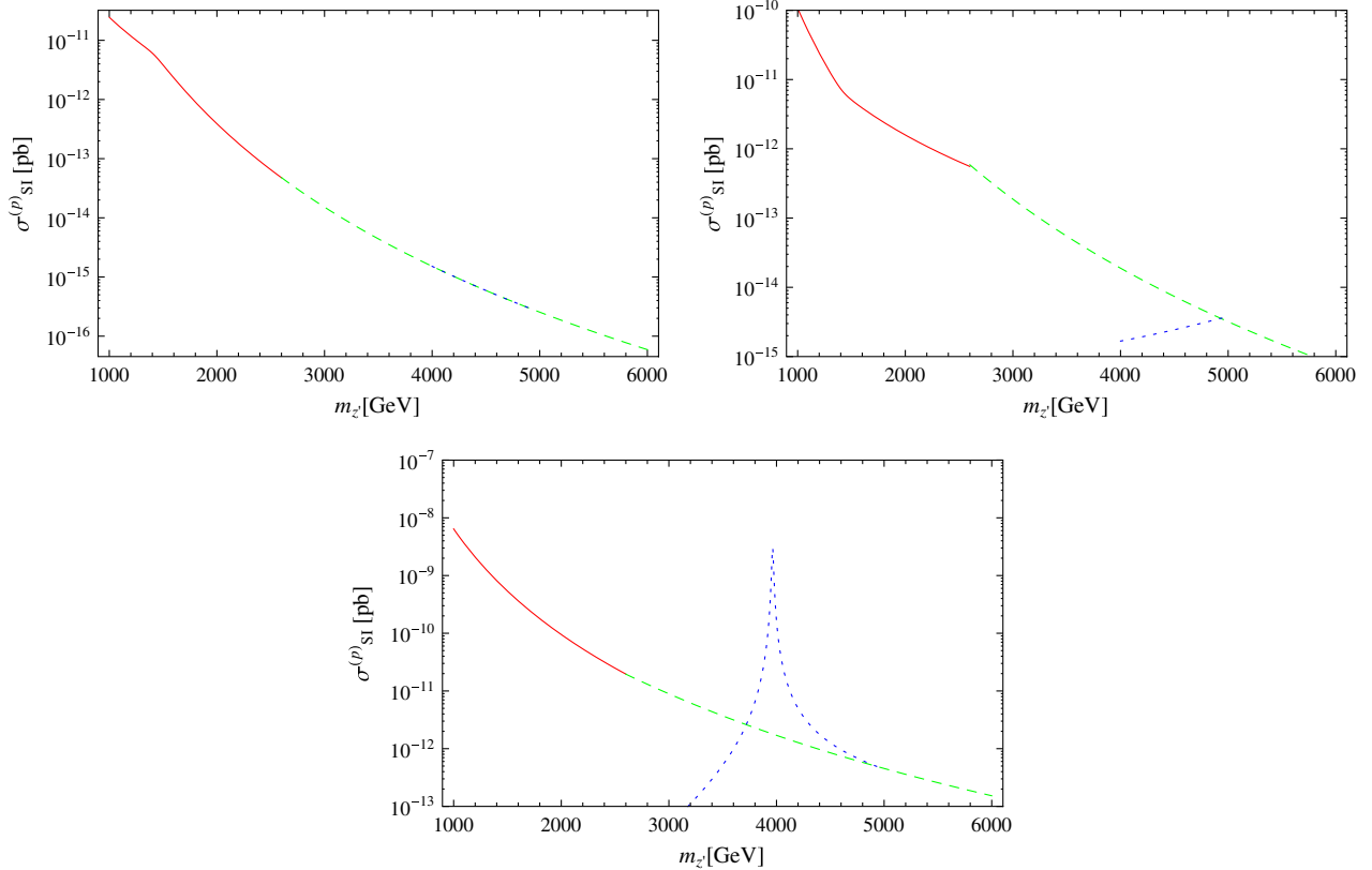
FIG. 4 (color online). The spin-independent cross sections as a function of Z' boson mass. The top-left panel shows the case of m_{\text{DM}} \sim M_H/2 , the top-right panel is for the case of M_{\text{DM}} \sim M_\Phi/2 , and the case for M_{\text{DM}} \sim m_{z'}/2 is shown in the bottom panel. The (red) solid lines, the (green) dashed lines, and the (blue) dotted lines correspond to the LEP line, naturalness line, and LHC line, respectively.
