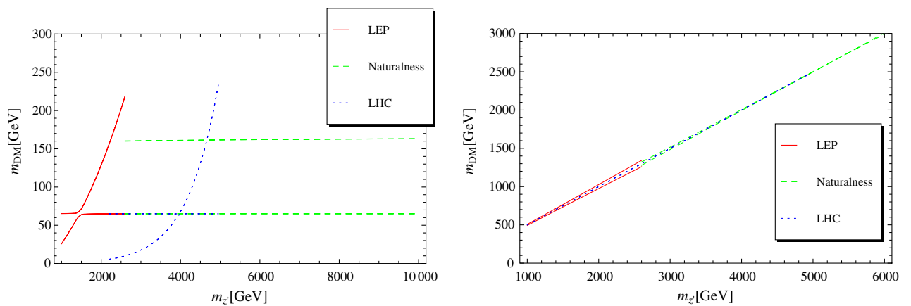
FIG. 3 (color online). The dark matter mass as a function of Z' boson mass. The left panel shows the results when the dark matter mass is close to half of Higgs masses, while the right panel corresponds to the case with the dark matter mass being close to half of the Z' boson mass. The solid, dashed, and dotted lines correspond to the LEP, naturalness, and LHC lines, respectively.
