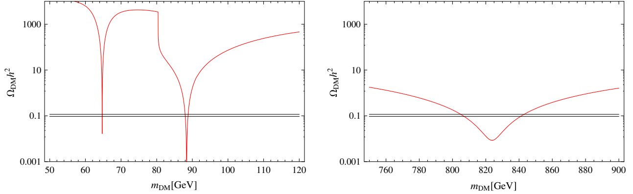
FIG. 2 (color online). The thermal relic density of the right-handed neutrino dark matter as a function of its mass. The left panel corresponds to the Higgs resonance regions while the right panel to the Z' resonance region.
