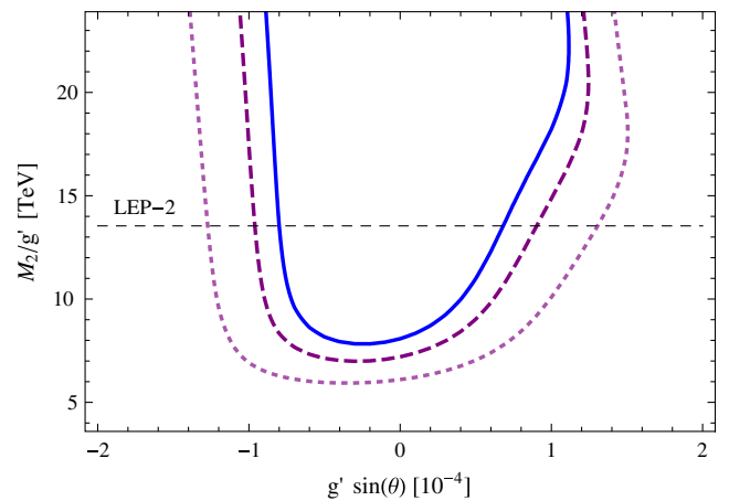
FIG. 2 (color online). \chi^2 contours (90%, 95% and 99% C.L.) in the M_2 - \sin(\theta) plane. The horizontal dashed line is the 95% C.L. lower limit from LEP-2 [29].
