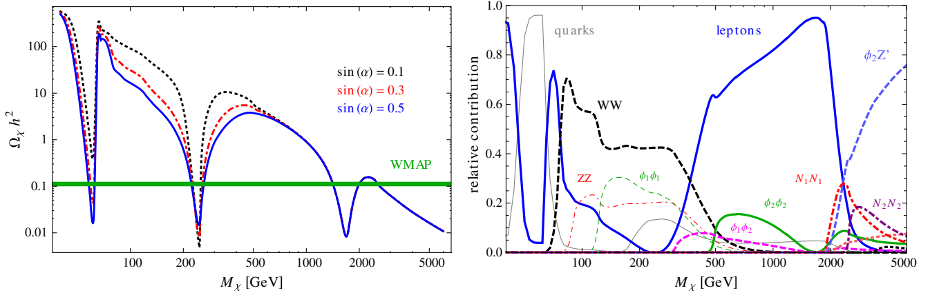
FIG. 3 (color online). Left panel: Relic density of \chi for the parameters m_1 = 125 GeV, m_2 = 500 GeV, v_S = 2.3 TeV, g' = 0.25 , N_1 = 1.9 TeV, N_2 = 2.5 TeV, and \sin\alpha = 0.5 (blue), 0.3 (red) and 0.1 (black). This puts the \phi_1 , \phi_2 and Z' resonances at \sim 60 GeV, 250 GeV and 1.7 TeV, respectively. The green band shows the 3\sigma range measured by WMAP. Right panel: Relative contribution to the relic density by the processes \chi\chi \rightarrow q\bar{q} (sum over all quarks), leptons (including neutrinos), ZZ , etc., for \sin\alpha = 0.3 .
