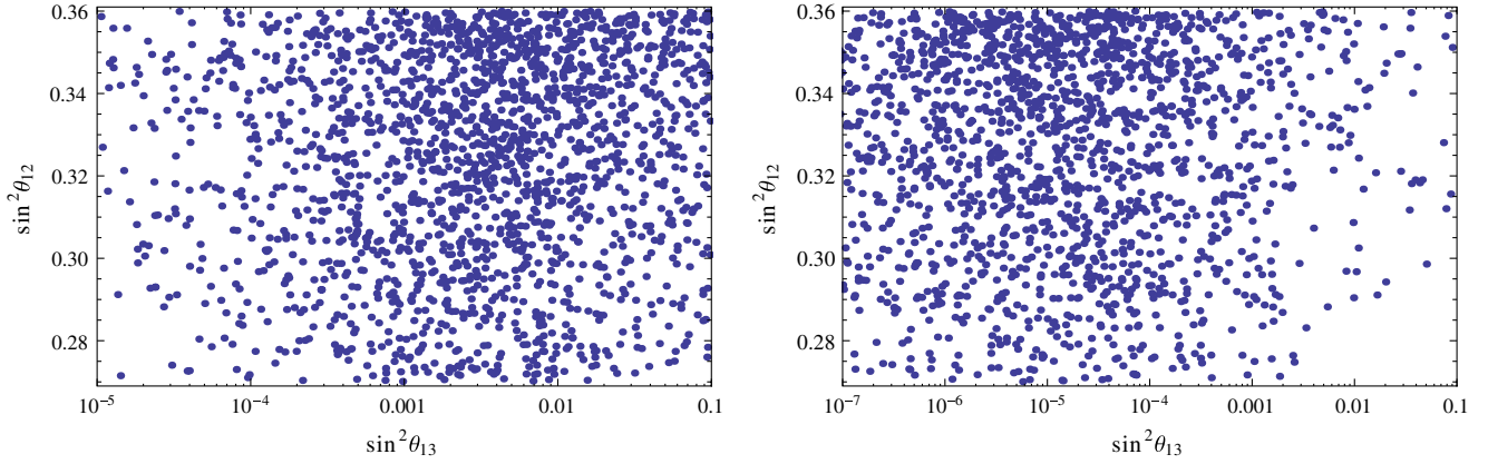
FIG. 1 (color online). Left panel: scatter plots using the broken B + 3\bar{L} low-energy neutrino mass matrix (5) ( \varepsilon = 0.05 ) that leads to NH. Right panel: scatter plots using the neutrino mass matrix (11) ( \varepsilon = 0.1 ) with five right-handed neutrinos and a \mathbb{Z}_2 , which leads to IH. The accepted values of the mixing parameters satisfy the 3\sigma bounds from Ref. [18], except for \theta_{23} , because it can be arbitrarily adjusted by the charged-lepton contribution.
