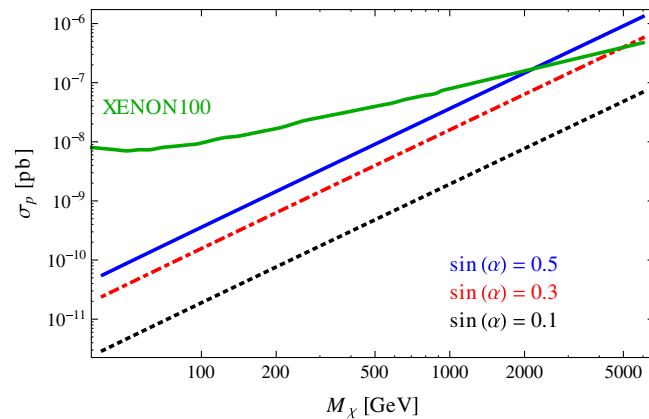
FIG. 4 (color online). Spin-independent cross section of \chi with a proton with the same parameters as Fig. 3, i.e. m_1 = 125 GeV, m_2 = 500 GeV, v_S = 2.3 TeV, g' = 0.25 , N_1 = 1.9 TeV, N_2 = 2.5 TeV, and \sin\alpha = 0.5 (blue line), 0.3 (red, dashed line) and 0.1 (black, dotted line). Also shown is the XENON100 90% C.L. exclusion from Ref. [36].
