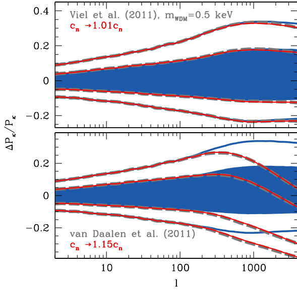
FIG. 9 (color online). Demonstration of our parametrization of WDM (upper panel) and baryonic effects (lower panel) with the Halofit parameter c_n , using the CFHTLS source distribution. Upper panel: Flat \Lambda CDM prediction for the shear power spectrum in blue, shown with predictions for 0.5 keV WDM as in Ref. [49] with grey dashed lines and predictions for c_n \rightarrow 1.01c_n with red solid lines. Lower panel: Flat \Lambda CDM prediction for the shear power spectrum in blue, shown with predictions for baryons (including AGN feedback) as in Ref. [51] with grey dashed lines and predictions for c_n \rightarrow 1.15c_n with red solid lines.
