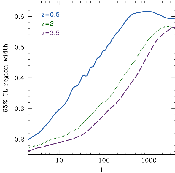
FIG. 4 (color online). Single source plane, 95% CL full-width extent for the shear power spectrum \Delta P_\kappa/P_\kappa (as plotted in the lower panel of Fig. 3) as a function of l , for sources at z = 0.5 (top, blue solid curve), 2 (middle, green dotted curve), and 3.5 (bottom, purple dashed curve).
