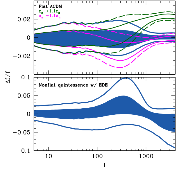
FIG. 10 (color online). The ratio f(l) of the COSMOS and CFHTLS cosmic shear power spectrum predictions for the flat \Lambda CDM (upper panel) and nonflat quintessence with EDE (lower panel) model classes, plotted with respect to the ratio of the ML COSMOS and CFHTLS power spectra. Once again, shaded regions correspond to 68% CL, and the curves bound the 95% CL regions. The upper panel also shows how the flat \Lambda CDM ratio changes when either c_n (upper green contours) or a_n (lower magenta contours) are amplified by 10%, where the altered 68% CL regions are bounded by solid lines and the corresponding altered 95% CL regions are bounded by dashed lines.
