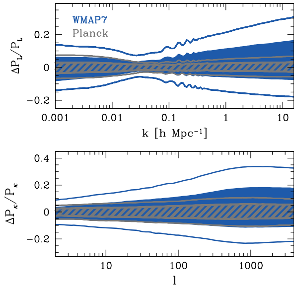
FIG. 7 (color online). Expected improvements from Planck (grey hatched region) over WMAP7 (blue solid region) for flat \Lambda CDM predictions. The upper panel shows the linear matter power spectrum, and the lower panel shows the shear power spectrum for the CFHTLS source redshift distribution, with the 68% and 95% CL regions relative to the ML flat \Lambda CDM model.
