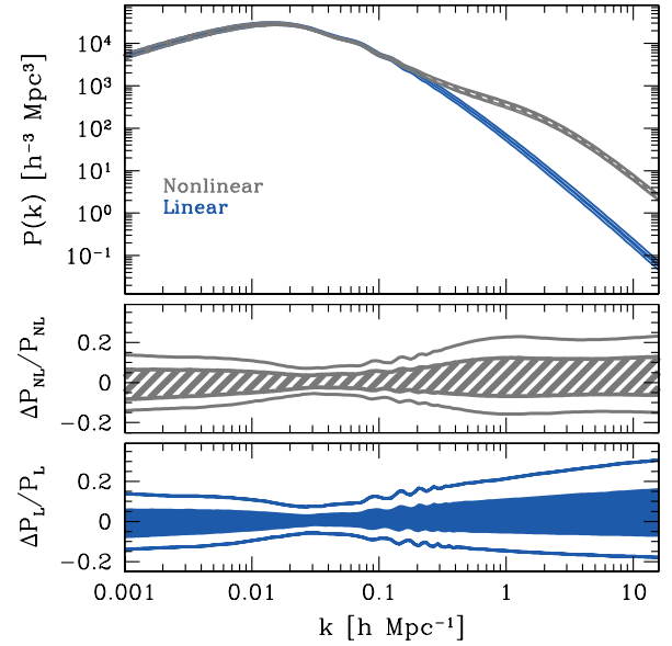
FIG. 2 (color online). Flat \Lambda CDM prediction for the z = 0 matter power spectrum, showing the 68% and 95% CL regions as in Fig. 1. Upper panel: Linear (blue solid region) and nonlinear (grey hatched region) matter power spectra. Middle panel: Fractional confidence range in the nonlinear spectrum around the ML flat \Lambda CDM model. Lower panel: The same for the linear power spectrum. Note k is in units of h \text{ Mpc}^{-1} .
