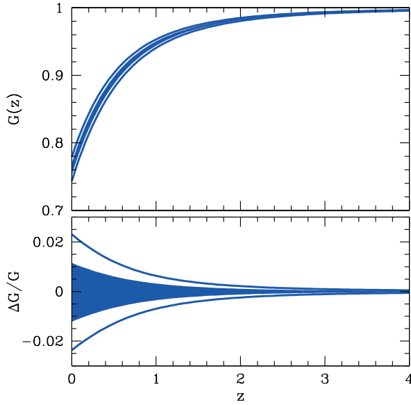
FIG. 1 (color online). Flat \Lambda CDM prediction for the growth factor (upper panel) and its deviation from the ML flat \Lambda CDM model (lower panel). The shaded regions correspond to 68% CL, and the curves bound the 95% CL regions.
