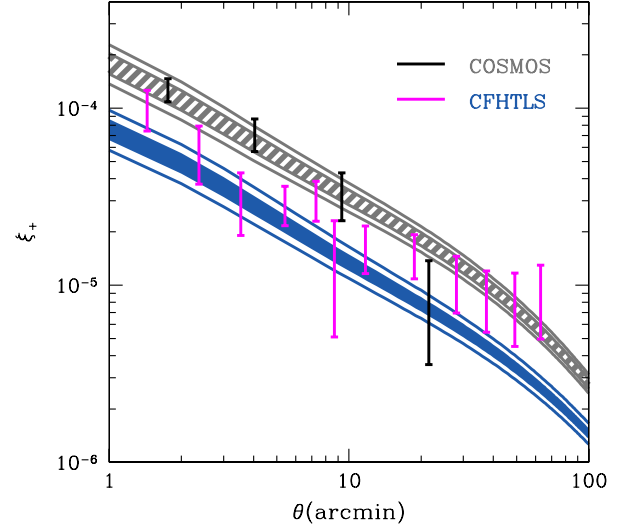
FIG. 5 (color online). Flat \Lambda CDM predictions for \xi_+ , showing the 68% and 95% CL regions as in Fig. 3 for both the COSMOS (grey hatched region) and CFHTLS (blue solid region) source redshift distributions. Also shown are the data points from Refs. [8] (black points) and [43] (magenta points) with 1\sigma error bars. Note that the error bars at different angular separations are correlated.
