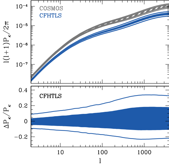
FIG. 3 (color online). Upper panel: Flat \Lambda CDM predictions for the shear power spectrum, showing the 68% and 95% CL regions as in Fig. 1 for COSMOS (upper, grey hatched region) and CFHTLS (lower, blue solid region). Lower panel: CFHTLS shear power spectrum prediction plotted with respect to the ML flat \Lambda CDM model.
