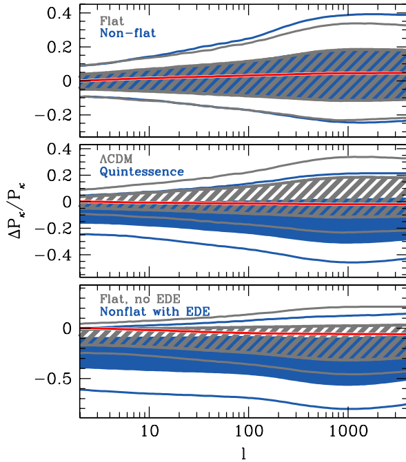
FIG. 6 (color online). Generalizing the model class for shear power spectrum predictions for the CFHTLS source redshift distribution. In all cases, the range is shown relative to the ML flat \Lambda CDM model, with blue regions indicating the wider model class and grey hatched regions the narrower: (upper panel) \Lambda CDM flat vs nonflat predictions; (middle panel) flat \Lambda CDM vs flat quintessence without EDE; (lower panel) flat quintessence without EDE vs nonflat quintessence with EDE (blue solid line). Red lines correspond to the maximum likelihood model of the more general of the two classes compared.
