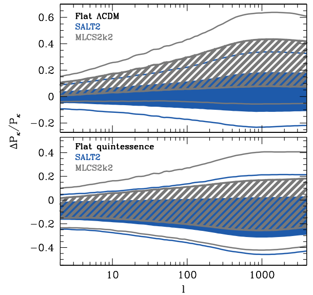
FIG. 11 (color online). Shear power spectrum predictions for the CFHTLS source redshift distribution, where we show the bias resulting from the choice of SN light-curve fitter. Upper panel: Flat \Lambda CDM predictions for SALT2 (blue solid region) and MLCS2k2 (grey hatched region), plotted relative to the ML SALT2 flat \Lambda CDM result. Once again, the shaded regions correspond to 68% CL, and the curves bound the 95% CL regions. Lower panel: Flat quintessence predictions for SALT2 (blue solid region) and MLCS2k2 (grey hatched region), also plotted relative to the ML SALT2 flat \Lambda CDM result.
