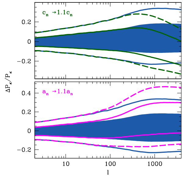
FIG. 8 (color online). Upper panel: Flat \Lambda CDM prediction for the CFHTLS shear power spectrum in blue, shown with the prediction for when the parameter c_n is amplified by 10% (green curves). The altered 68% CL regions are bounded by solid lines, and the corresponding altered 95% CL regions are bounded by dashed lines. Lower panel: Same as above, but now instead the one-halo term amplitude a_n is amplified by 10% (magenta curves).
