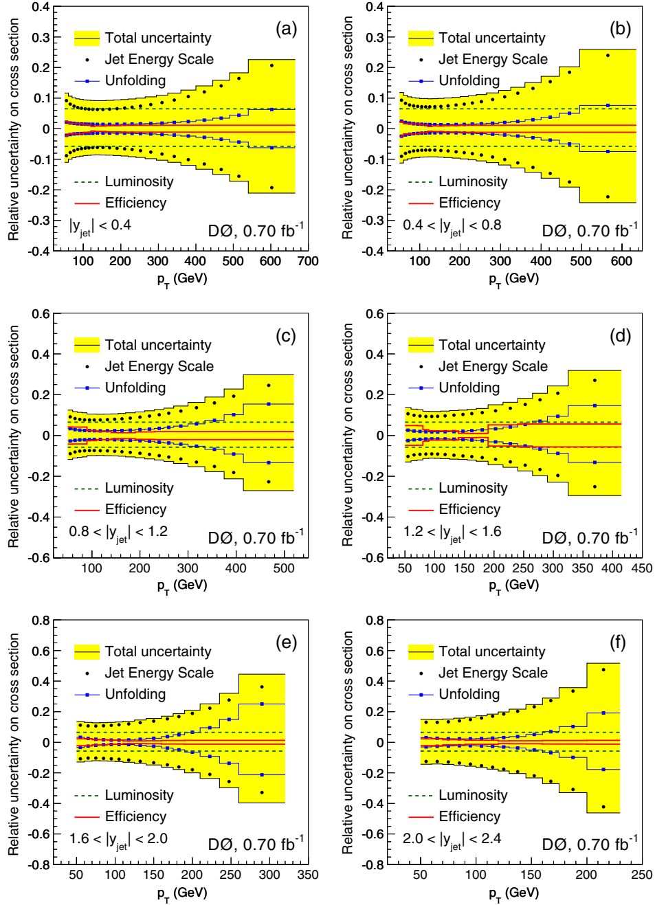
FIG. 45 (color online). (color online) Different components of the systematic uncertainty as a function of jet p_T in the six y bins.
