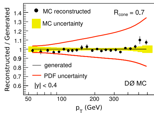
FIG. 37 (color online). (color online) MC closure test of the method used to extract the inclusive jet p_T cross section for the jet |y| < 0.4 bin. The full analysis was repeated treating MC events as data and comparing the result to the input cross section. Good agreement is found within the statistical uncertainties of fits to jet energy scale and resolution, and unfolding present in MC (shaded band), which are much smaller than the systematic uncertainties in data.
