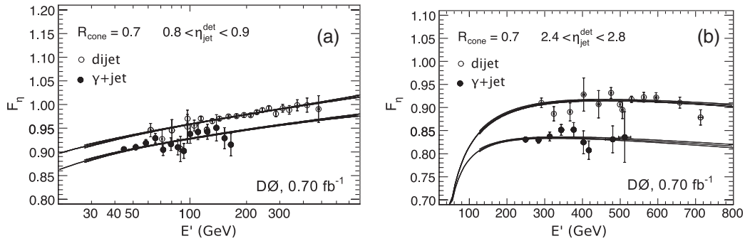
FIG. 10. Fits of F_\eta in \gamma + \text{jet} and dijet data for two different regions in \eta as a function of E' . The central fit values and the uncertainty band are displayed on the figure.
