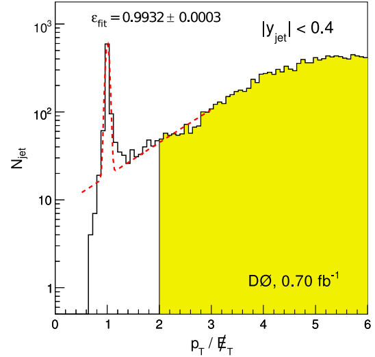
FIG. 26 (color online). (color online) Distribution of p_{T,\text{lead}}/\cancel{E}_T for jet events with leading jet p_T > 200 GeV. A peak from cosmic ray background is visible around 1. The shaded region shows jets passing the p_{T,\text{lead}}/\cancel{E}_T requirement.
