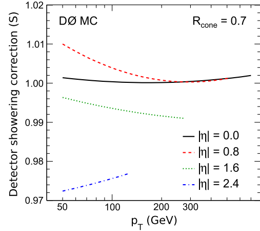
FIG. 15 (color online). (color online) Jet showering corrections shown as a function of jet p_T for different regions of jet pseudorapidity.
