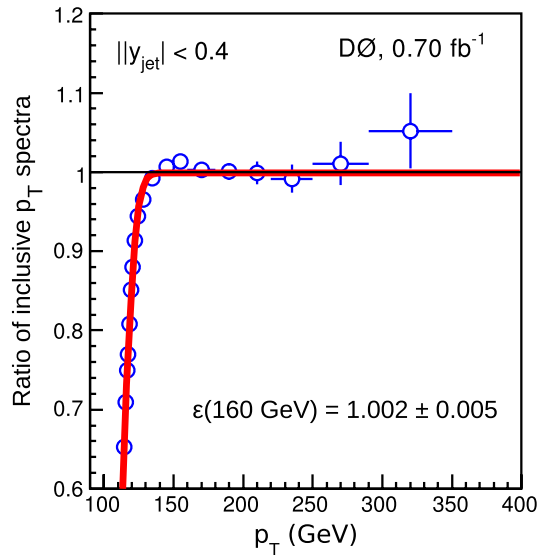
FIG. 24 (color online). (color online) Ratio of two consecutive jet triggers used to obtain the relative jet trigger efficiency for the 95 and 65 GeV single jet triggers. The fit of the turn-on curve determines the 95 GeV jet p_T 99%-threshold to be 130 GeV. A higher threshold of 160 GeV that is consistent with an efficiency \epsilon = 1.00 is used in the final analysis.
