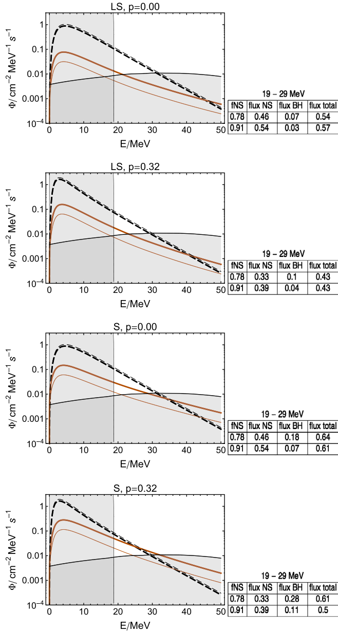
FIG. 8 (color online). The diffuse flux of \nu_e from neutron star-forming collapses (dashed lines) and from failed supernovae (direct black hole-forming, solid lines). We use two different equations of state (the S EoS and the LS EoS), the extreme values for the survival probability ( p = 0, 0.32 ) and two values of the fraction of neutron star-forming collapses: f_{\text{NS}} = 0.78 (thick lines) and f_{\text{NS}} = 0.91 (thin). For each case, we give the integrated flux in the energy interval of interest, in units of \text{cm}^{-2}\text{s}^{-1} .
