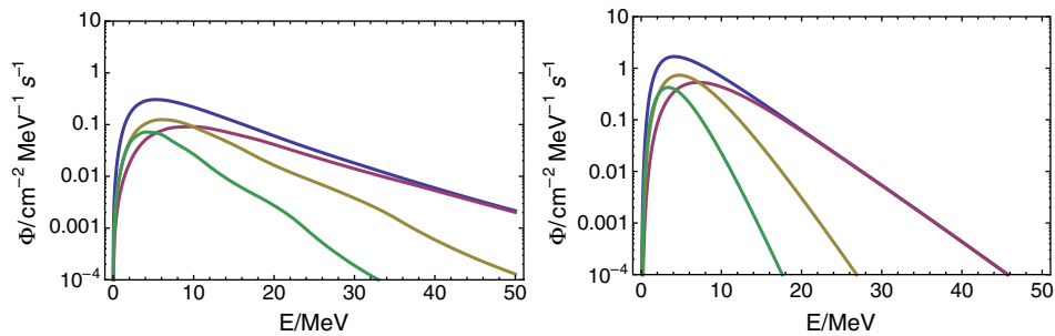
FIG. 2 (color online). The diffuse flux of \bar{\nu}_e from black hole-forming collapses (left panel) and from neutron star-forming collapses (right panel) from different bins of redshift, z . From lower to upper curves at 20 MeV: 2 \leq z < 3 , 1 \leq z < 2 , 0 \leq z < 1 , and the total from all redshifts. We used the S EoS, \bar{p} = 0.68 and f_{\text{NS}} = 0.78 .
