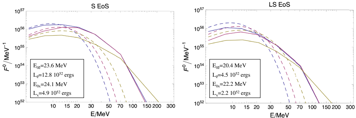
FIG. 1 (color online). Neutrino fluxes at production inside the star for direct black hole-forming collapses (solid, from [13]), and neutron star-forming collapses (dashed, Eq. (2)). In both cases, the curves from upper to lower at 10 MeV correspond to \nu_e, \bar{\nu}_e, \nu_x . For direct black hole-forming collapses the neutrino spectra are shown for the Shen et al. (left panel) and Lattimer-Swesty (right) equations of state. For each, the neutrino luminosities and average energies are given (insets). See text for details.
