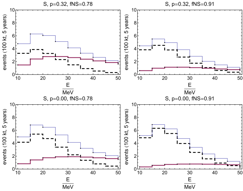
FIG. 9 (color online). The number of \nu_e events in a liquid argon detector with exposure 0.5 \text{ Mt} \cdot \text{yr} , for different sets of parameters. Histograms are shown, using the S EoS, for direct black hole-forming collapses only (solid thick, purple), neutron star-forming collapses only (dashed, black), and total (solid, thin, blue).
