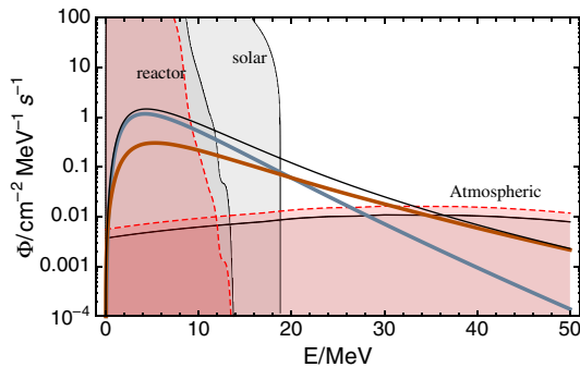
FIG. 4 (color online). Signal and background fluxes. The atmospheric and reactor fluxes are shown for the Kamioka (solid, gray) and Homestake (dashed, red) sites. The atmospheric fluxes of \nu_e and \bar{\nu}_e (from [49]) are very similar, so only one of them is plotted. The calculations of the background fluxes include oscillation effects, which are responsible for the visible modulation of the reactor spectrum. The signal flux plotted refers to the \bar{\nu}_e channel, with the S EoS, p = 0.68 and f_{\text{NS}} = 0.78 . From the lower to upper curves at 40 MeV: the flux from neutron star-forming collapses, the flux from direct black hole-forming collapses and the total flux.
