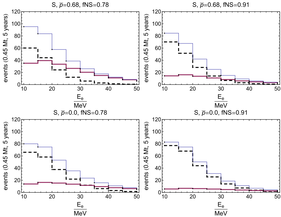
FIG. 6 (color online). The number of inverse beta decay events in a water Cherenkov detector with exposure 2.25 \text{ Mt} \cdot \text{yr} . Histograms are shown, with the S EoS, for direct black hole-forming collapses only (solid thick, purple), neutron star-forming collapses only (dashed, black), and total (solid, thin, blue).
