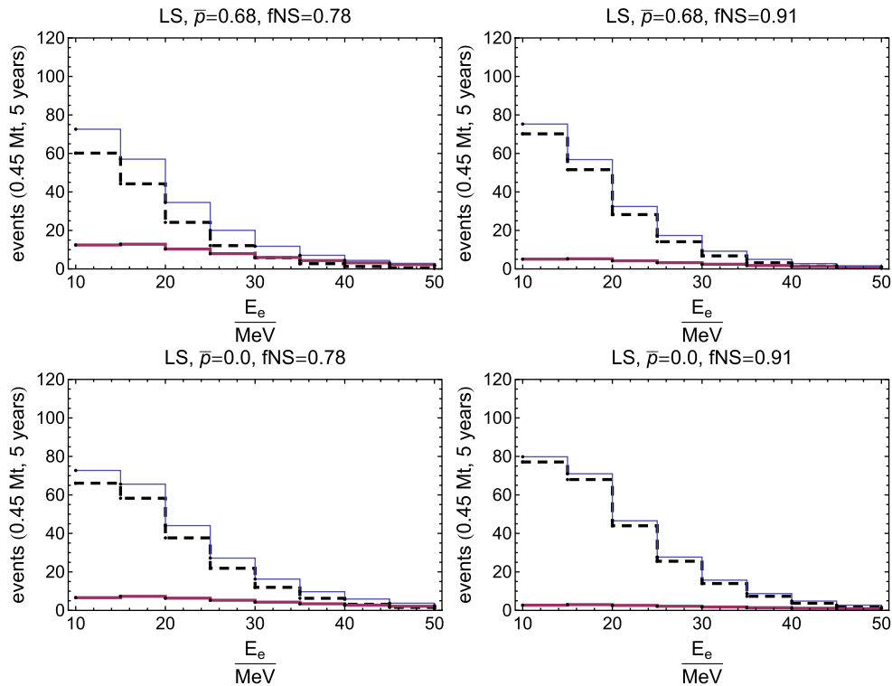
FIG. 7 (color online). The same as Fig. 6, for the LS EoS.
