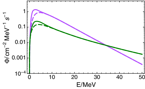
FIG. 3 (color online). \nu_e fluxes from direct black hole-forming collapses (lower curves at 10 MeV) and from neutron star-forming collapses (upper curves) for p = 0 (dashed lines) and for the steplike probability in Eq. (7) (solid). The swap energies are E_c = 12.1, 8.0 MeV for the two fluxes, respectively. We used the S EoS and f_{\text{NS}} = 0.78 .
