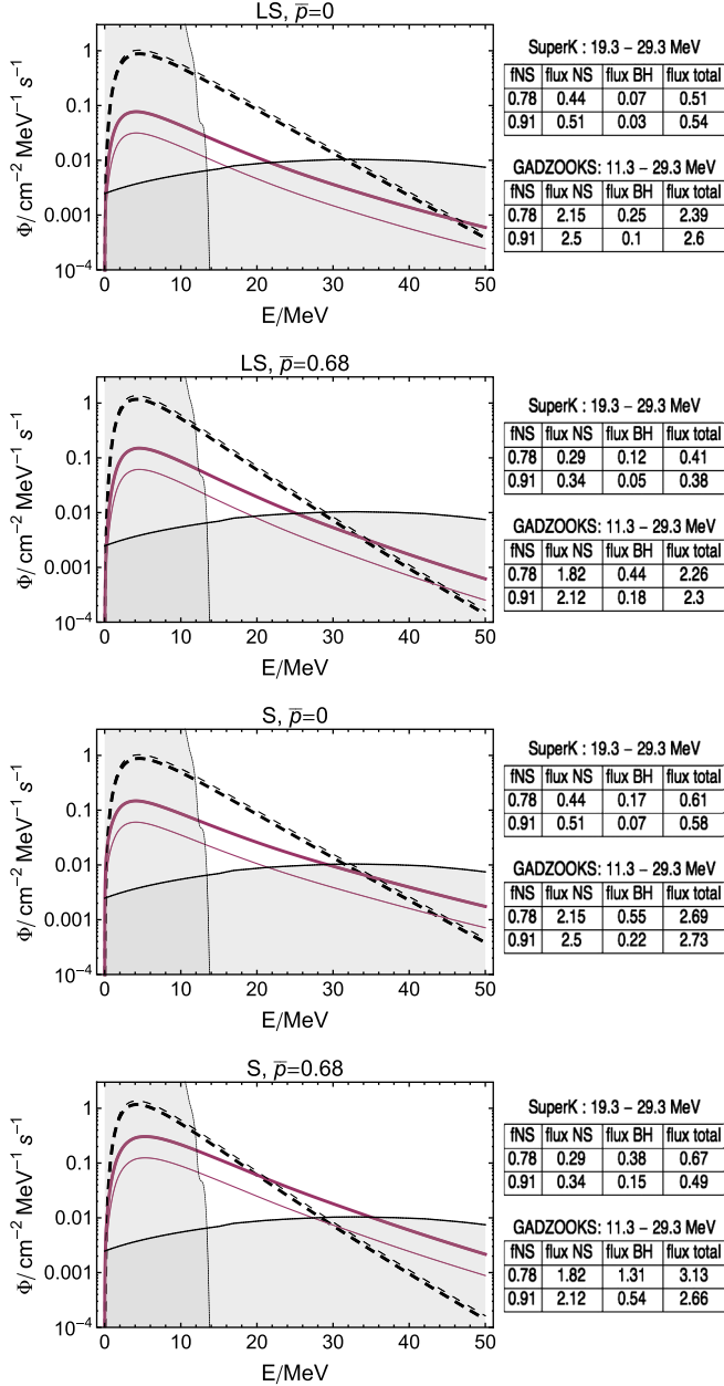
FIG. 5 (color online). The diffuse flux of \bar{\nu}_e from neutron star-forming collapses (dashed lines) and from failed supernovae (direct black hole-forming, solid lines). We use two different equations of state (the S EoS and the LS EoS), the extreme values for the survival probability ( \bar{p} = 0, 0.68 ) and two values of the fraction of neutron star-forming collapses: f_{\text{NS}} = 0.78 (thick curves) and f_{\text{NS}} = 0.91 (thin lines). For each case we give the integrated flux in energy intervals of interest, in units of \text{cm}^{-2} \text{s}^{-1} .
