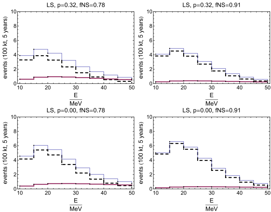
FIG. 10 (color online). The same as Fig. 9 for the LS EoS.
