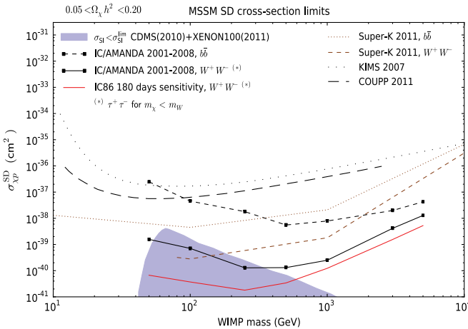
FIG. 6 (color online). Left : Ninety percent confidence level upper limits on the spin-dependent neutralino-proton cross section, \sigma_{\chi p}^{\text{SD}} , as a function of neutralino mass. The results from the analyses presented in this paper are shown as the black dots joined with lines to guide the eye (solid and dashed for the W^+W^- and the b\bar{b} annihilation channels, respectively). The shaded area represents the allowed MSSM parameter space taking into account current accelerator, cosmological and direct dark matter search constraints. The solid red curve shows the expected sensitivity of the completed IceCube detector. Results from Super-K [43], KIMS [44] and COUPP [45] are also shown for comparison. Right : Ninety percent confidence level upper limits on the spin-independent neutralino-proton cross section, \sigma_{\chi p}^{\text{SI}} , as a function of neutralino mass. The results from the analyses presented in this paper are shown as the black dots joined with lines to guide the eye (solid and dashed for the W^+W^- and the b\bar{b} annihilation channels, respectively). The shaded area represents the allowed MSSM parameter space taking into account current accelerator, cosmological and direct dark matter search constraints. The red curve shows the expected sensitivity of the completed IceCube detector. Results from CDMS [36] and XENON [37] are also shown for comparison.
