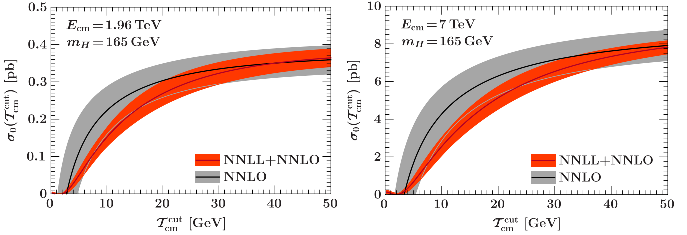
FIG. 4 (color online). Comparison of gg \rightarrow H + 0 jets using \mathcal{T}_{\text{cm}}^{\text{cut}} at fixed NNLO with the resummed results at NNLL + NNLO. For the fixed-order uncertainties in \sigma_0 we use independent inclusive scale variations in \sigma_{\text{total}} and \sigma_{\geq 1} . The uncertainty method for the resummed results is described in the text.
