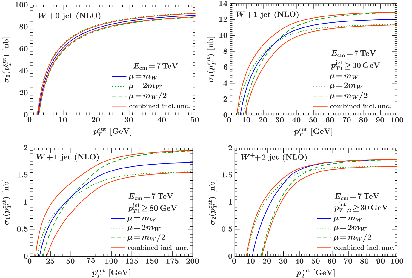
FIG. 3 (color online). Fixed-order perturbative uncertainties for the exclusive pp \rightarrow W + 0, 1, 2 jet cross sections at NLO for the LHC with E_{\text{cm}} = 7 TeV. Central values are shown by blue solid curves, direct exclusive scale variation in the exclusive jet bin by the green dashed and dotted curves, and the result of combining independent inclusive uncertainties to get the jet-bin uncertainty by the outer red solid curves.
