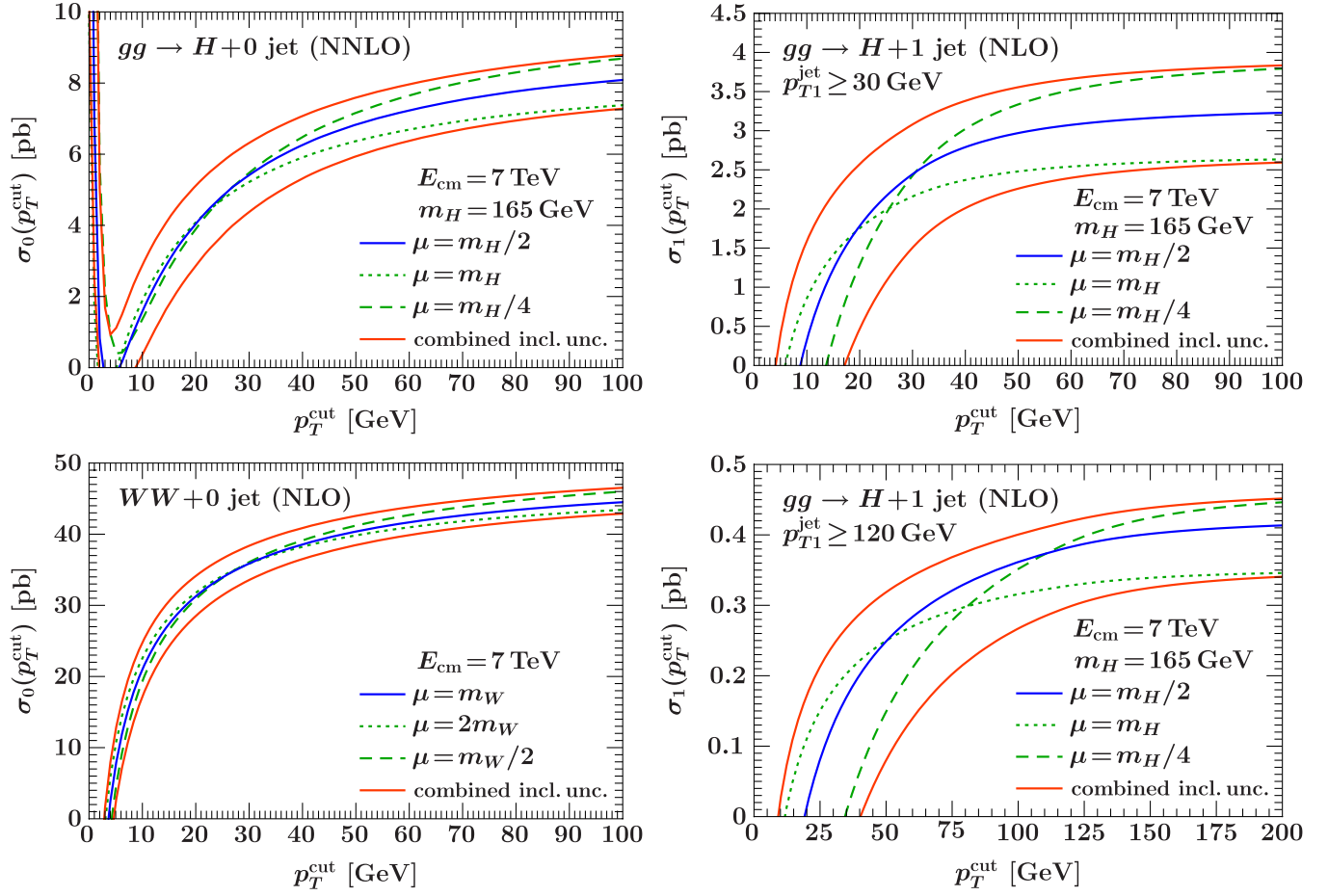
FIG. 1 (color online). Perturbative predictions for H + 0 jets (upper left panel), WW + 0 jets (lower left panel), H + 1 jet with p_{T1}^{\text{jet}} \geq 30 GeV (upper right panel), and H + 1 jet with p_{T1}^{\text{jet}} \geq 120 GeV (lower right panel). Central values are shown by the blue solid curves, direct scale variation in the exclusive jet bin by the green dashed and dotted curves, and the result of combining independent inclusive uncertainties to get the jet-bin uncertainty by the outer red solid curves.
