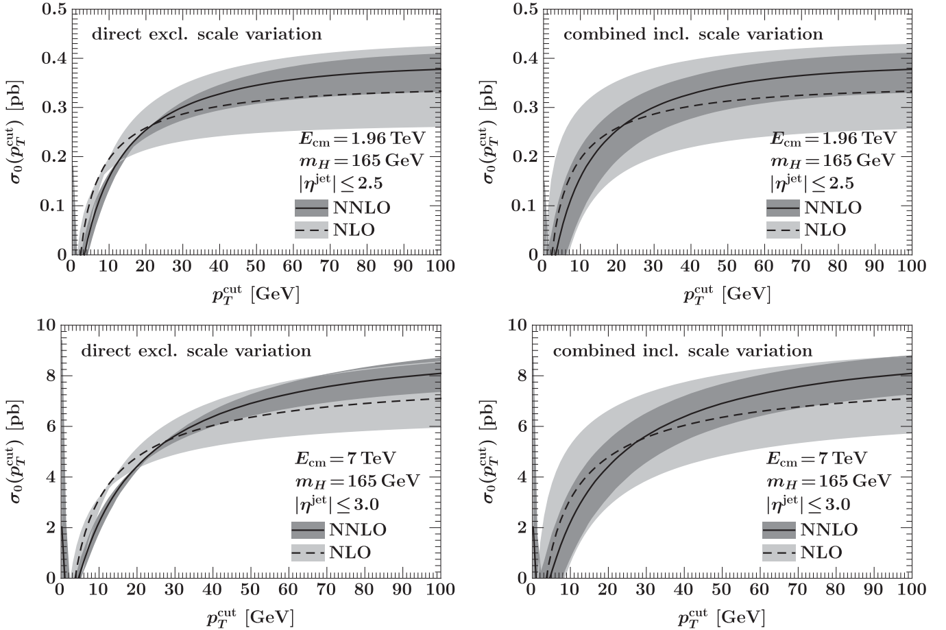
FIG. 2. Fixed-order perturbative uncertainties for gg \rightarrow H + 0 jets at NLO and NNLO. The upper panels are for the Tevatron and the lower panels for the LHC with E_{\text{cm}} = 7 TeV. On the left, the uncertainties are obtained from the direct scale variation in \sigma_0(p_T^{\text{cut}}) between \mu = m_H/4 and \mu = m_H . On the right, the uncertainties are obtained by independently evaluating the scale uncertainties in \sigma_{\text{total}} and \sigma_{\geq 1}(p_T^{\text{cut}}) and combining them in quadrature. (For the LHC case the dark shaded NNLO bands correspond to results in the top left panel of Fig. 1. The direct exclusive scale variation band corresponds to the dashed green lines, and the combined inclusive uncertainty band corresponds to the solid red lines.)
