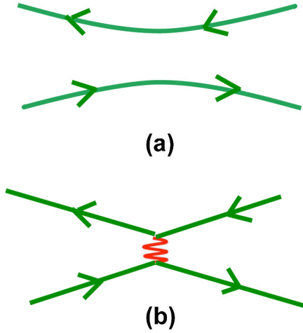
FIG. 4 (color online). (a) The valence diagram for quark-antiquark scattering in a meson. (b) The contribution of t-channel RR exchange to the valence diagram.
