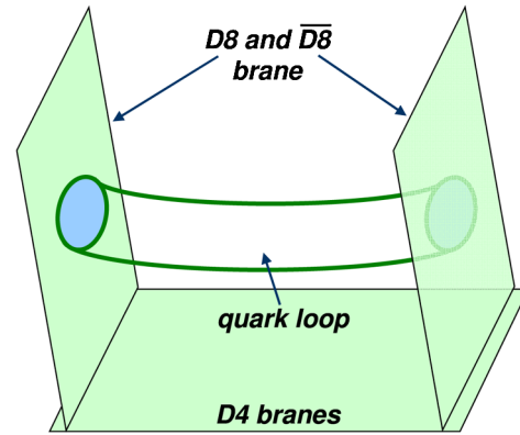
FIG. 6 (color online). String representation of the intermediate state in the valence diagram for quark-antiquark scattering, which takes place by quark strings joining at the color ends. Here the cylinder represents the partition function of the D8 - \overline{D8} intermediate string.
