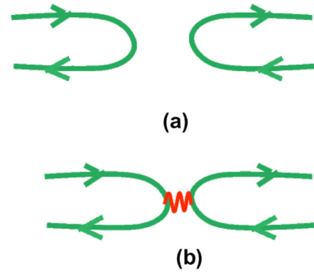
FIG. 3 (color online). (a) The quenched double hairpin correlator which measures the gluonic \eta' mass insertion. The indicated quark propagators are assumed to be summed over all gauge field configurations. (b) The s-channel RR exchange picture for the hairpin correlator. RR exchange results in a local 4-quark contact interaction due to its derivative coupling to the chiral field. These q_\mu factors cancel the massless pole and convert it to a delta-function.
