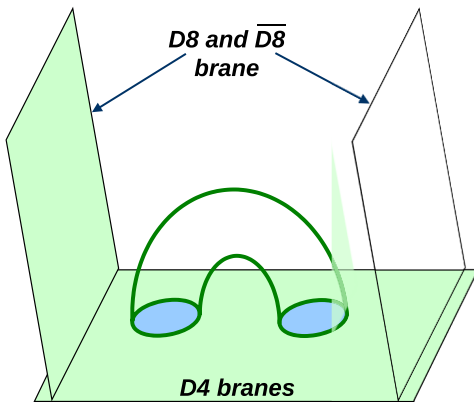
FIG. 5 (color online). String representation of the intermediate state in the double hairpin diagram for quark-antiquark scattering, which takes place by quark strings joining at the flavor ends. Here the cylinder represents the partition function of the D4-D4 intermediate string.
