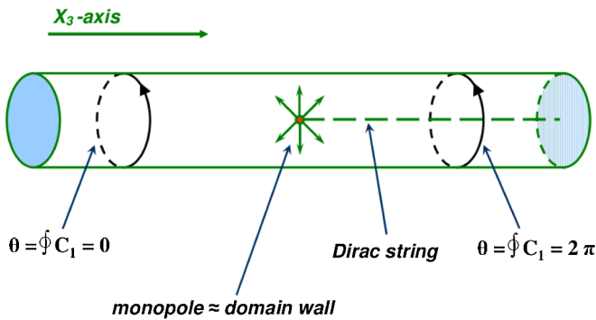
FIG. 2 (color online). View of a D6 brane as a magnetic monopole of the Ramond-Ramond gauge field in the three dimensions transverse to its world volume.
