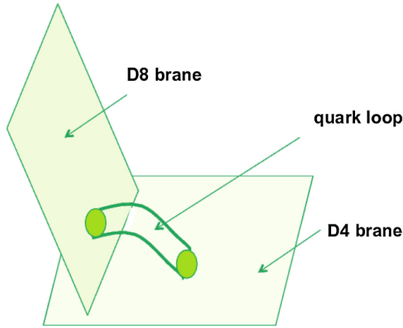
FIG. 1 (color online). An open-string quark loop as a closed-string exchange between D4 and D8 branes.
