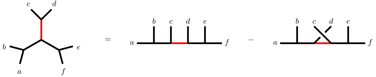
FIG. 4 (color online). Illustration of the kinematic Jacobi relation associated with the indicated edge, as given in Eq. (5.1), which expresses the numerator of the trimerous topology on the left in terms of the difference between the two half-ladders on the right.
