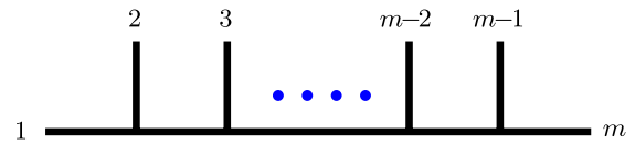
FIG. 1 (color online). Illustration of a generic m -point half-ladder diagram.
