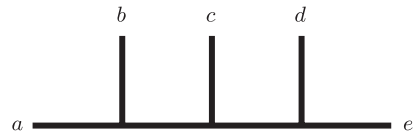
FIG. 3. The five-point half-ladder diagram. All contributions in cubic-graph representations of five-loops involve this topology or are related by antisymmetry around vertices.
