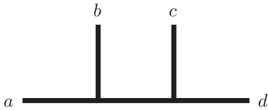
FIG. 2. The four-point cubic diagram. It appears with three distinct labelings of external legs (a, b, c, d) , corresponding to the s -channel diagram: (1, 2, 3, 4) , the t -channel diagram: (2, 3, 4, 1) , and the u -channel diagram: (3, 1, 4, 2) .
