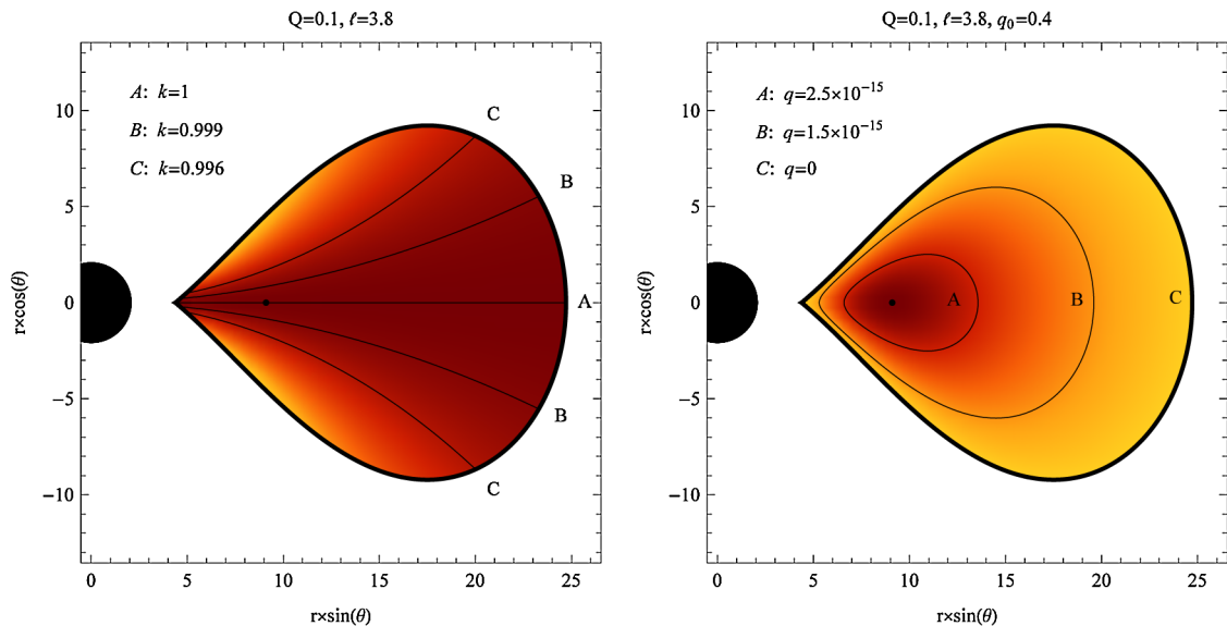
FIG. 5 (color online). Poloidal sections through the isocontours for the correction function k(r, \theta) (left) and the charge density q(r, \theta) (right) for the same positively charged torus as in Fig. 4.
