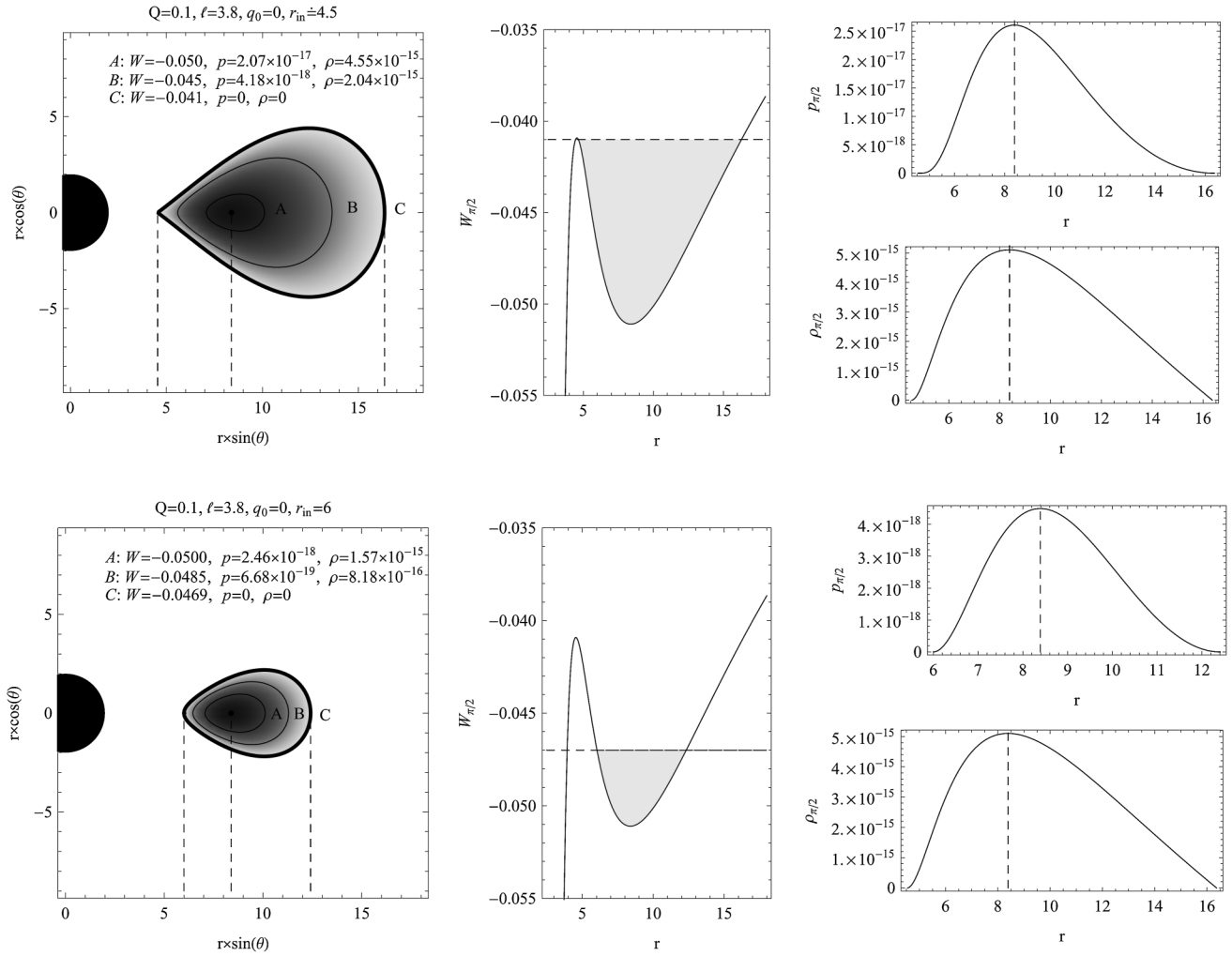
FIG. 3. Profiles of the potential W(r, \theta) , pressure p(r, \theta) and rest-mass density \rho(r, \theta) of uncharged tori, shown in terms of poloidal sections through the equipotential, isobaric and isodensity surfaces, respectively, and their equatorial behavior W_{\pi/2}(r) , p_{\pi/2}(r) and \rho_{\pi/2}(r) , for a Reissner-Nordström spacetime with Q = 0.1 . Two examples are shown with different values for the radius at the inner edge of the torus: r_{in} = r_{cusp} = 4.544 in the upper figures and r_{in} = 6 in the lower ones. The centers (pressure maxima) of both tori are located at r_{cent} = 8.388 . The shapes of the equipotential, isobaric and isodensity surfaces coincide, with the values of the different quantities on them being related by Eq. (24) and the equation of state (22). We show poloidal sections through three such surfaces (A, B and C). The thick curve (surface C) marks the zero-pressure (and zero-density) surface which bounds the torus. The shaded regions above the profiles of W_{\pi/2}(r) indicate the physically relevant parts of the profiles, delimited by the inner and outer edges of the tori. The specific angular momentum \ell = 3.8 for both tori, and the polytropic parameters are \Gamma = 2 and \kappa = 10^{12} in each case.
