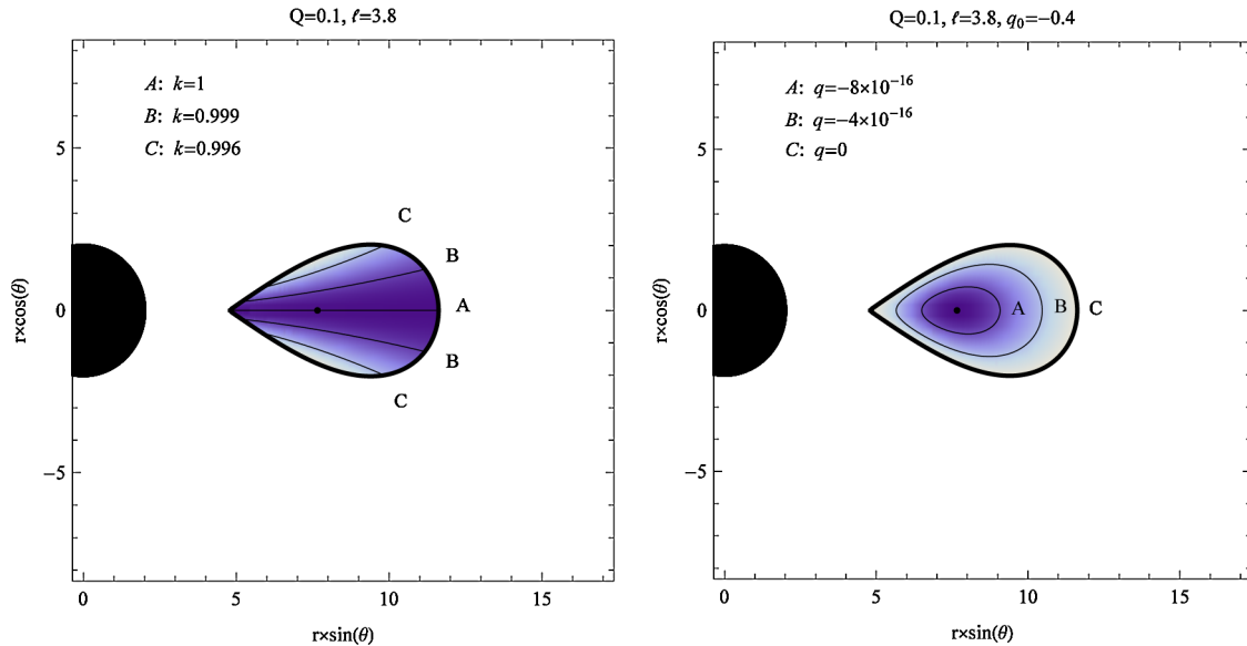
FIG. 7 (color online). Poloidal sections through the isocontours for the correction function k(r, \theta) (left) and the charge density q(r, \theta) (right) for the same negatively charged torus as in Fig. 6.
