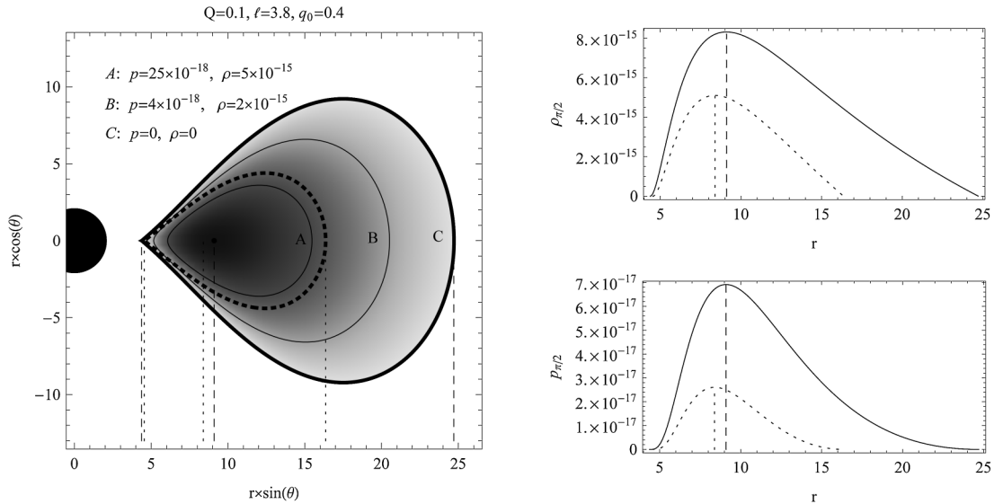
FIG. 4. Profiles of the pressure p(r, \theta) and rest-mass density \rho(r, \theta) for a positively charged torus ( q_0 = 0.4, \ell = 3.8 ) in a Reissner-Nordström spacetime with Q = 0.1 , shown in terms of poloidal sections through the isobaric and isodensity surfaces (left), and in terms of their equatorial profiles p_{\pi/2}(r) and \rho_{\pi/2}(r) (right). The torus terminates at r_{\text{in}} = r_{\text{cusp}} \doteq 4.378 and r_{\text{out}} \doteq 24.72 , and its center is located at r_{\text{cent}} \doteq 9.098 . The dashed curves represent the zero-pressure surface for the equivalent uncharged case (left panel) and the profiles of density and pressure for the uncharged case (right panels). The isobaric and isodensity surfaces coincide (A, B and C), with the values of pressure and density on them being related by the equation of state.
