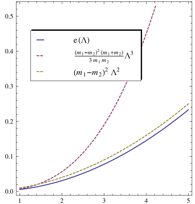
FIG. 2 (color online). The energy density as a function of the cutoff \Lambda , with the values: m_1 = 1 , m_2 = 0.9 , in arbitrary units (sufficient for our purpose here, which is to demonstrate the dependence on \Lambda only) is plotted. The two plots correspond to two different cutoff regimes: the diagram on the left, shows the behavior of e(\Lambda) for small \Lambda . It approaches zero as e(\Lambda) \sim \Lambda^3 for \Lambda \rightarrow 0 ; the plot on the right depicts the behavior of the energy density for large \Lambda , where we have e(\Lambda) \sim \Lambda^2 . As a typical scale of the theory, with respect to which we define the low and high cutoff scale, we take m_1 \approx m_2 = 1 .
