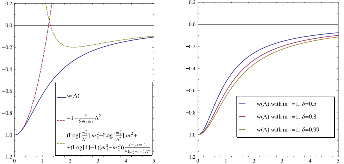
FIG. 4 (color online). The equation of state w as a function of the cutoff is plotted; The plot on the left corresponds to m_1 = 1 , m_2 = 0.9 . In the plot on the right we depict a set of three curves, each of them corresponding to different values of the mass-difference parameter \delta : m_2 \equiv m + \delta and m_1 \equiv m , with m = 1 and \delta = 0.5, 0.8, 0.99 .
