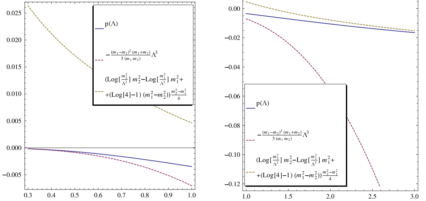
FIG. 3 (color online). The pressure as a function of the cutoff \Lambda , with the values \sin\theta = 2\pi^2 , m_1 = 1 , m_2 = 0.9 is plotted. Again, on the left we have the behavior of p(\Lambda) for small \Lambda (compared with m_2 \approx m_1 = 1 ), where p(\Lambda) \sim \Lambda^3 , and on the right for large \Lambda , where p(\Lambda) \sim \log(\Lambda) .
