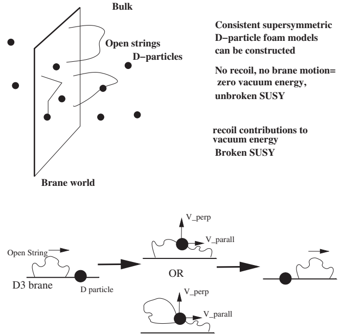
FIG. 1. Upper: schematic representation of a generic D-particle space-time foam model, in which matter particles are treated as open strings propagating on a D3-brane, and the higher-dimensional bulk space-time is punctured by D-particle defects. Lower: details of the process whereby an open-string state propagating on the D3-brane is captured by a D-particle defect, which then recoils. This process involves an intermediate composite state that persists for a period \delta t \sim \alpha' E , where E is the energy of the incident string state, which distorts the surrounding space-time during the scattering, leading to an effective refractive index but not birefringence. The components of the recoil velocity perpendicular to the D3 braneworld lead to vacuum energy contributions and thus target-space supersymmetry-breaking.
