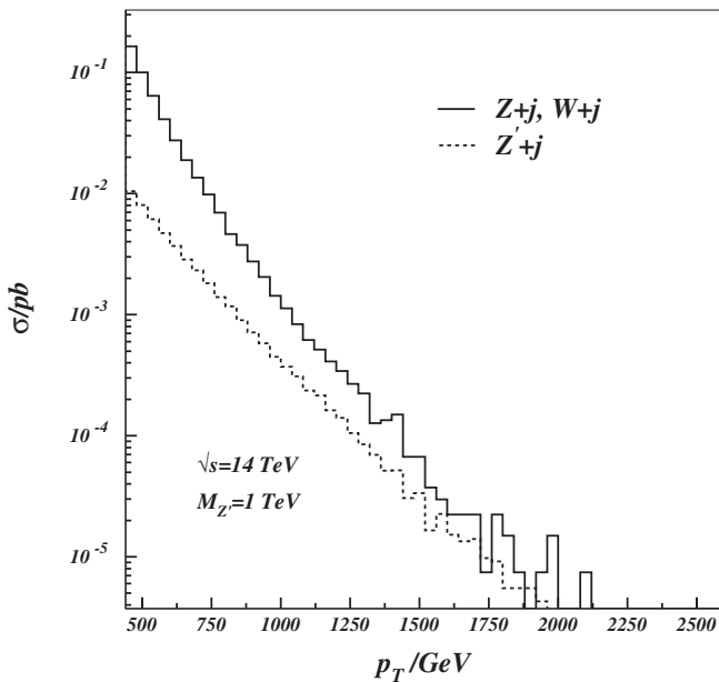
FIG. 5. Monojet p_T distributions for a 1-TeV Z' signal and the SM background at \sqrt{s} = 14 TeV. A cut has been placed requiring p_T > 440 GeV, which gives S/B = 10\% .
