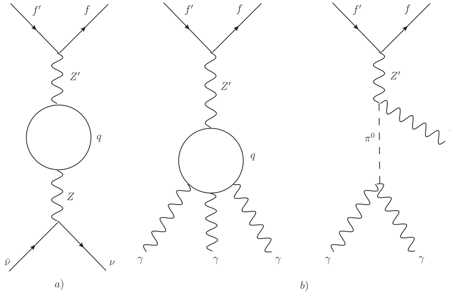
FIG. 3. Diagrams contributing to f' decay in the case of vector couplings to the Z' . (a) f' \rightarrow f\nu\bar{\nu} via Z' - Z mixing. (b) Example diagrams contributing to f' \rightarrow f\gamma\gamma\gamma .
