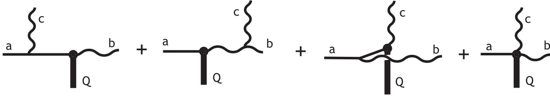
FIG. 1. Feynman diagrams for the computation of the Fg \rightarrow Fgg splitting functions [8].
