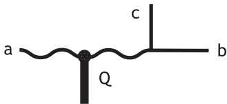
FIG. 2. The single Feynman diagram for the computation of the gg \rightarrow gF\bar{F} splitting function [8].
