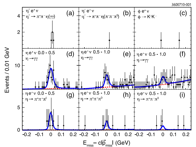
FIG. 1 (color online). Tagged analysis U distributions in data (points) for D^+ \rightarrow \eta' e^+ \nu_e (a), (b), D^+ \rightarrow \phi e^+ \nu_e with \phi \rightarrow K^+ K^- (c), and D^+ \rightarrow \eta e^+ \nu_e with \eta \rightarrow \gamma\gamma (d)–(f) and \eta \rightarrow \pi^+ \pi^- \pi^0 (g)–(i), in the three q^2 intervals. The total (solid line) and background (dashed line) distributions from the fits are also shown.
