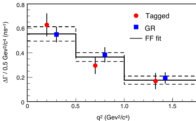
FIG. 6 (color online). The partial rates from the tagged (circles) and GR (squares) analyses, and the form factor (FF) fit (histogram). The dashed lines indicate the total uncertainty on the fit rates.
