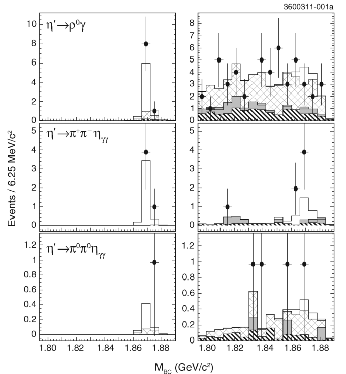
FIG. 3. M_{BC} distributions (GR analysis) for data (points) and signal (unshaded), D\bar{D} (cross-hatch), continuum (grey), and fake e^\pm (45° hatch) fit components for both the HQ (left) and non-HQ (right) subsamples in the \eta' \rightarrow \rho \gamma (top), \eta' \rightarrow \pi^+ \pi^- \eta \gamma \gamma (middle), and \eta' \rightarrow \pi^0 \pi^0 \eta \gamma \gamma (bottom) submodes.
