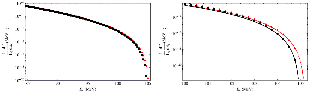
FIG. 1 (color online). End-point region of the electron spectrum for aluminum. The squares correspond to the spectrum with recoil effects, Eq. (18). For comparison, we show the spectrum neglecting recoil, Eq. (10), as the triangles. The right plot is a zoom for E_e > 100 MeV, the solid (dashed) line on this plot corresponds to the Taylor expansion around the end-point with (without) recoil.
