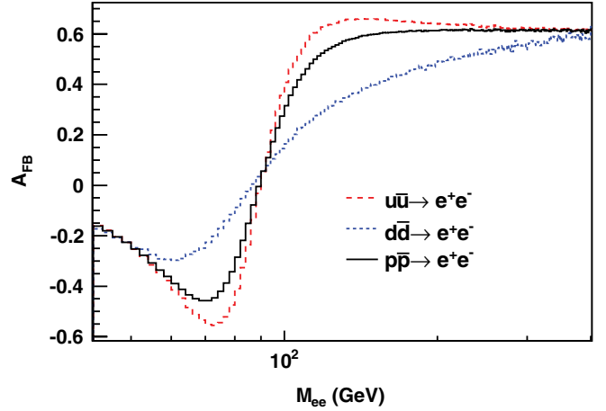
FIG. 2 (color online). The SM LO A_{\text{FB}} prediction as a function of the dielectron invariant mass for u\bar{u} \rightarrow e^+e^- , d\bar{d} \rightarrow e^+e^- , and p\bar{p} \rightarrow e^+e^- [4].
