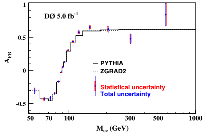
FIG. 7 (color online). Comparison between the unfolded A_{\text{FB}} (points) and the PYTHIA (solid curve) and ZGRAD2 (dashed line) predictions. The boxes and vertical lines show the statistical and total uncertainties, respectively.
