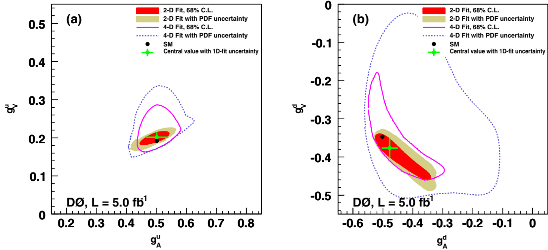
FIG. 8 (color online). The 68% C.L. contours of (a) g_V^u and g_A^u , and (b) g_V^d and g_A^d from a two-dimensional and a four-dimensional \chi^2 fit with statistical and systematic uncertainties. The outer regions are determined by the theoretical PDF uncertainty. The two-dimensional correlation contours correspond to \Delta\chi^2 = 2.3 for different g_A and g_V parameters, as obtained from two-parameter (shaded regions) and four-parameter (solid and dashed curves) fits. The value 2.3 corresponds to the 68% C.L. region in two dimensions. In the case of four-parameter fit, the curve is a projection onto the two-dimensional plane of the envelope of the four-dimensional \Delta\chi^2 = 4.72 surface. The crosses indicate the best two-dimensional fit values, and the uncertainties correspond to the one-dimensional limits.
