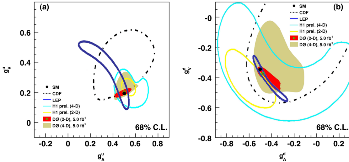
FIG. 9 (color online). The 68% C.L. contours of (a) g_V^u and g_A^u , and (b) g_V^d and g_A^d measured by DØ compared with other experiments. The LEP and CDF Collaborations performed fits with four free parameters to determine these couplings, while we and the H1 Collaboration performed both two and four free parameters fits. The LEP results have another solution (not shown) which is excluded by the H1, CDF, and DØ results.
