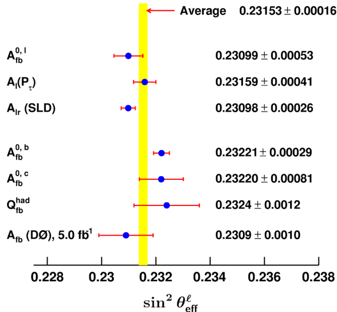
FIG. 6 (color online). Comparison of measured \sin^2\theta_{\text{eff}}^\ell with results from other experiments. The average is a combination of A_{\text{FB}}^{0,\ell} , A_l(P_\tau) , A_{lr}(\text{SLD}) , A_{\text{FB}}^{0,b} , A_{\text{FB}}^{0,c} , and Q_{\text{FB}}^{\text{had}} measurements from the LEP and SLD Collaborations.
