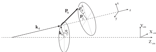
FIG. 2. Kinematics of the fragmentation process.
