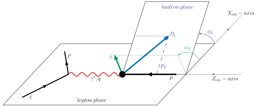
FIG. 1 (color online). Kinematical configuration and conventions for SIDIS processes. The initial and final lepton momenta define the (X-Z)_{cm} plane.
