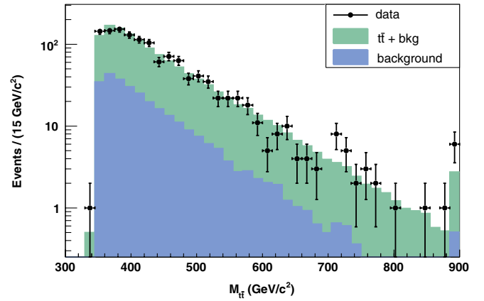
FIG. 9 (color online). Event distribution as a function of the total invariant mass M_{t\bar{t}} .
