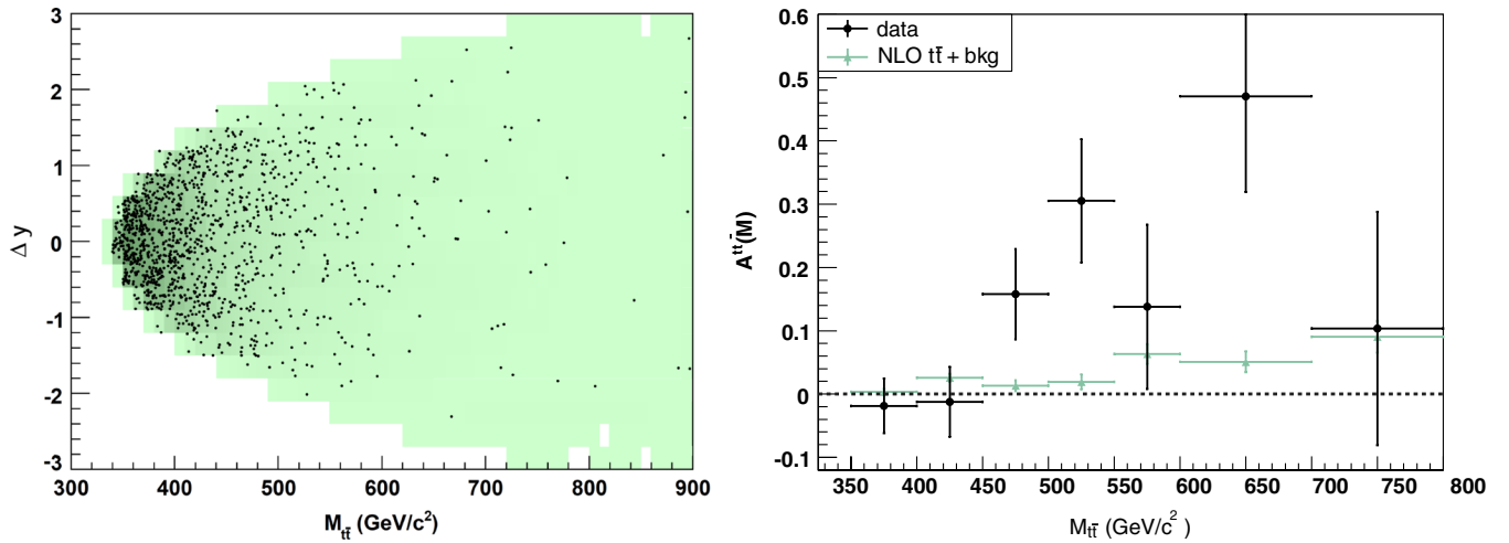
FIG. 10 (color online). Left: The \Delta y - M_{t\bar{t}} plane. Each dot represents one event, while the intensity of the shading shows approximately the event probability in the standard PYTHIA based prediction. Right: The t\bar{t} frame asymmetry in the data in bins of invariant mass M_{t\bar{t}} , compared to the prediction of MC@NLO t\bar{t} + backgrounds. The last bin includes all events with M_{t\bar{t}} \geq 700 \text{GeV}/c^2 .
