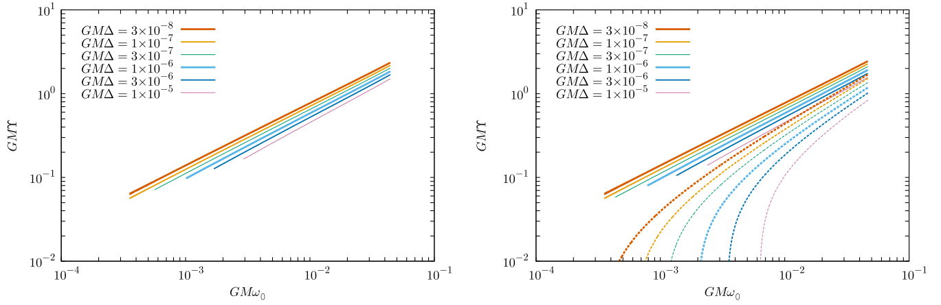
FIG. 1 (color online). Region of parameter space in which f(R) theories can be distinguished from GR when the central BH has spin a = 0 (left panel) or a = 0.5 (right panel). Each curve corresponds to a particular specification of the detectability criterion given in (129) in the text, as identified in the key. Dashed lines correspond to measurements of the vertical epicyclic frequency, while solid lines represent measurements of the radial epicyclic frequency. The region below the curve could be distinguishable in a LISA observation with that detectability value.
