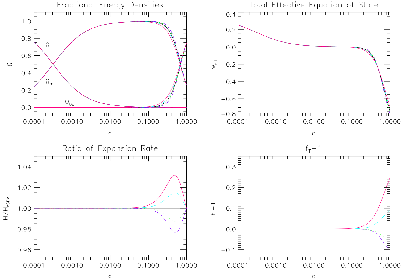
FIG. 1 (color online). The background evolution for the f(T) gravity model with f(T) = T - \mu^{2(1+n)}/(-T)^n . Upper-left Panel : the fractional energy densities for matter ( \Omega_m ), radiation ( \Omega_r ) and the effective dark energy ( \Omega_{\text{DE}} = 1 - \Omega_m - \Omega_r ), as functions of the cosmic scale factor a , which is normalized to 1 today. Upper-right Panel : the total effective equation of state w_{\text{eff}} = -1 - \frac{2\dot{H}}{3H^2} , as a function of a . Lower-left Panel : the ratio between the Hubble expansion rates for the f(T) gravity model and for the \Lambda CDM paradigm, as a function of a . Lower-right Panel : f_T - 1 as a function of a . Here, results are shown for n = 0 (black solid curve), 0.1 (green dotted curve), -0.1 (cyan dashed curve), 0.2 (purple dash-dotted curve) and -0.2 (pink dash-triple-dotted curve). Note that n = 0 corresponds to the \Lambda CDM paradigm. The relevant physical parameters are \Omega_m = 0.257 , \Omega_r = 8.0331 \times 10^{-5} and H_0 = 71.9 km/s/Mpc.
