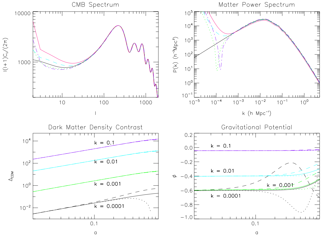
FIG. 3 (color online). The power spectra for the large-scale structure of the f(T) gravity model with f(T) = T - \mu^{2(1+n)}/(-T)^n . Upper-left Panel : the CMB spectrum for different values of n = 0 (black solid curve), 0.1 (green dotted curve), -0.1 (cyan dashed curve), 0.2 (purple dash-dotted curve) and -0.2 (pink dash-triple-dotted curve). Upper-right Panel : the same as the upper-left panel, but for the matter power spectrum at redshift 0 (today). Lower-left Panel : the late-time evolution of the dark matter density contrast \Delta_{\text{CDM}} on different scales (as indicated besides the curves); three values of n have been considered -n = 0.0 (solid curves), 0.1 (dotted curves) and -0.1 (dashed curves). Lower-right Panel : the same as the lower-left panel, but for the late-time evolution of the gravitational potential \phi on different scales. The physical parameters are the same as listed in the caption of Fig. 1, and three species of massless neutrinos are used.
