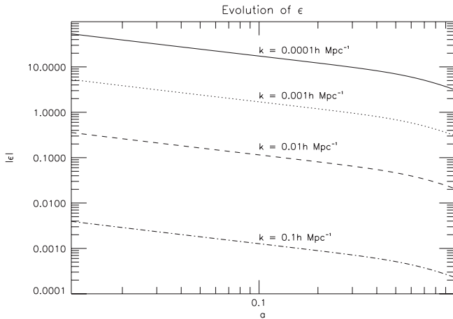
FIG. 2. The time evolution of frame-independent quantity \epsilon \equiv \varkappa + \sigma , with the scale factor, a(t) , for the model with f(T) = T - \mu^{2(1+n)}/(-T)^n and n = 0.1 , on different length scales, characterized, respectively, by k/(h \text{ Mpc}^{-1}) = 10^{-4} (solid curve), 10^{-3} (dotted curve), 10^{-2} (dashed curve) and 10^{-1} (dash-dotted curve).
