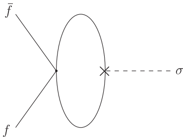
FIG. 1. Yukawa coupling between the SM fermions f and the scalar bound state \sigma in the framework of the ETC. The technifermion loop generates the mass of f and also intermediates between f and \sigma .
