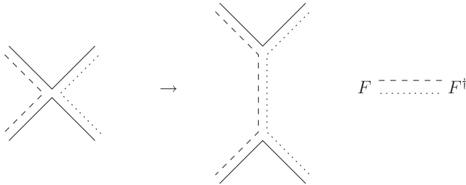
FIG. 3. F integrated in.
