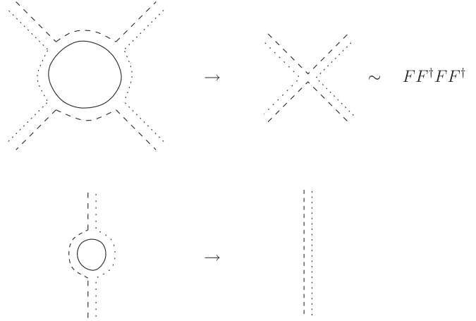
FIG. 4. C, D integrated out; note that you can have any even-valency (FF^\dagger)^p of F, F^\dagger vertices.
