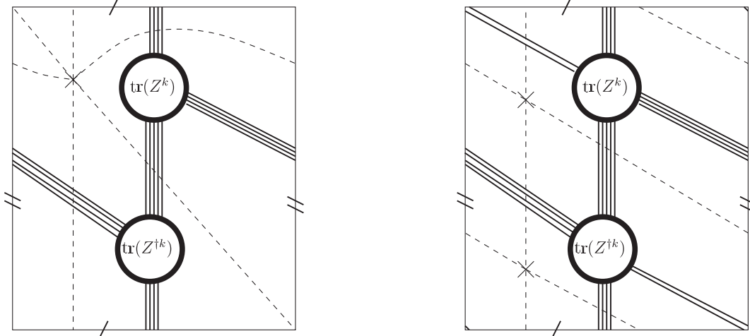
FIG. 9. The two different bunchings of propagators with no crossing for the Z model two-point function on the torus: three bunchings from \Sigma_{[3]} on the left and four bunchings from \Sigma_{[2,2]} on the right. The dual graphs are drawn with dashed lines. The left dual graph can be considered as a degenerate case of the right graph when the two vertices of the dual graph on the right collide.
