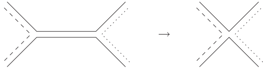
FIG. 2. Z integrated out.
