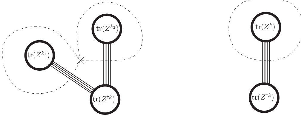
FIG. 8. Z model three-point function and two-point function on the sphere with bunched propagators. The dual graph is drawn with a dashed line.
