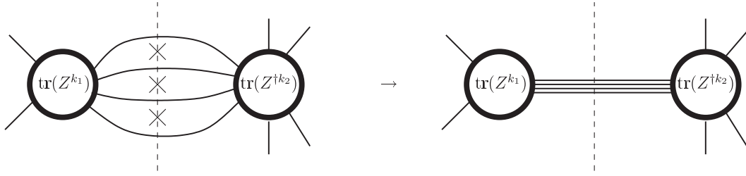
FIG. 7. Replacement of 2-valent vertices of the F model with plain \text{tr}(FF^\dagger) quadratic term (dashed lines), dual to faces bounded by parallel propagators in the Z model (thin solid lines), by the propagator of the proper F model (23), which is dual to the parallel propagators of the Z model bunched into an edge of the skeleton graph. [All propagators are drawn in a single-line notation here for ease of reading.]
