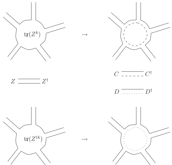
FIG. 1. C, D integrated in.
