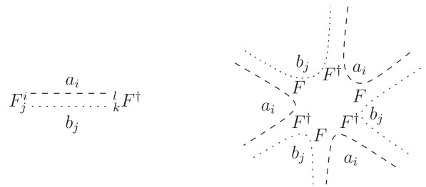
FIG. 5. Associations of A with dashed faces and B with dotted faces. On the left is the propagator and associated a_i, b_j . On the right is an example 6-valent vertex \text{tr}[(A^{-1} F B^{-1} F^\dagger)^3] , also with associated a_i, b_j .
