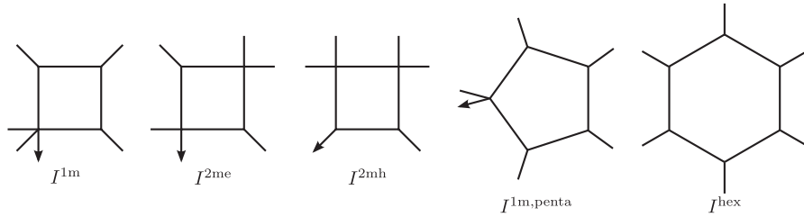
FIG. 1. The integrals contributing to the six-point one-loop MHV and NMHV amplitudes. An arrow marks the leg with momentum k_1 ; the remaining momenta follow clockwise. The one-mass box I^{1m} and two-mass easy I^{2me} integrals contribute to the MHV amplitude and the one-mass box I^{1m} and two-mass hard I^{2mh} integrals contribute to the NMHV amplitude. The one-mass pentagon I^{1m,penta} and the hexagon I^{hex} have numerator factors of \mu^2 [the square of the (-2\epsilon) -dimensional components of the loop momentum], and hence are finite. They contribute to both the MHV and NMHV amplitudes only at \mathcal{O}(\epsilon) and higher ( I^{hex} contributes to the even parts while I^{1m,penta} contributes to the odd parts).
