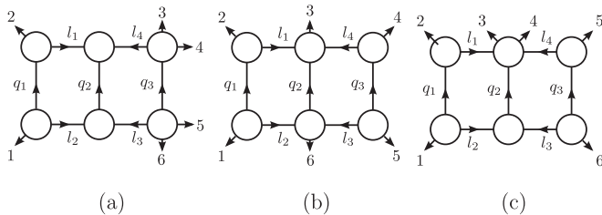
FIG. 6. Next-to-maximal cuts that detect the integrals not easily isolated by the iterated two-particle cuts: from left to right, next-to-maximal cuts for the hexabox, flying-squirrel, and rabbit-ears cuts of Figs. 2(c)–2(e), respectively.
