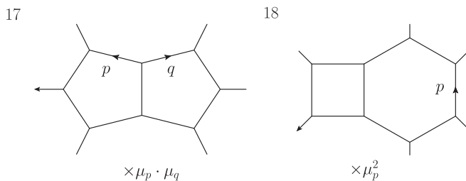
FIG. 8. \mu -integrals entering the two-loop six-point amplitudes. The arrow on the external line indicates leg number 1.
