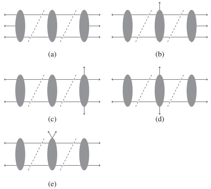
FIG. 2. Generalized cuts required to determine the two-loop NMHV amplitude: (a) the double-pentagon cut, (b) the turtle cut, (c) the “hexabox” cut, (d) the flying-squirrel cut, and (e) the “rabbit-ears” cut. Unlike the MHV calculation, all cyclic permutations of the external legs must be considered.
