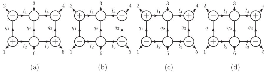
FIG. 7. The four possible assignments of internal helicities for the next-to-maximal flying-squirrel cut of Fig. 6(b). The “ \ominus ” vertices denote three-point \overline{\text{MHV}} amplitudes while the “ \oplus ” vertices denote three-point MHV amplitudes.
