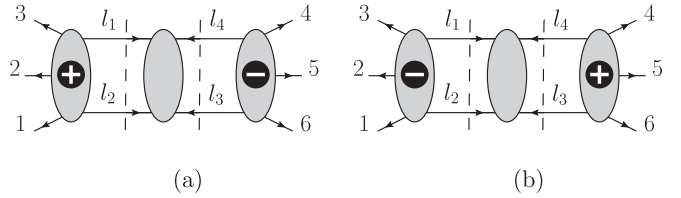
FIG. 5. The two contributions to the double-pentagon supercut (Fig. 2(a)). The circled + and - denote MHV and \overline{\text{MHV}} superamplitudes, respectively. The middle amplitude may be chosen to be either of MHV or of \overline{\text{MHV}} type. Here we choose to present it as an MHV superamplitude.
