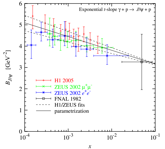
FIG. 2 (color online). The exponential t slope, B_{J/\psi} , of the differential cross section of exclusive J/\psi photoproduction measured in the FNAL E401/E458 [16], HERA H1 [9], and ZEUS [17] experiments, as a function of x = M_{J/\psi}^2/W^2 . (In the H1 and ZEUS results the quoted statistical and systematic uncertainties were added linearly.) The dashed lines represent the published two-dimensional fits to the H1 and ZEUS data [9,17]. The parameter B_g in the exponential two-gluon form factor Eq. (5) is related to the measured J/\psi slope by Eq. (8). Our parametrization Eqs. (9)–(12) is shown by the solid line.
