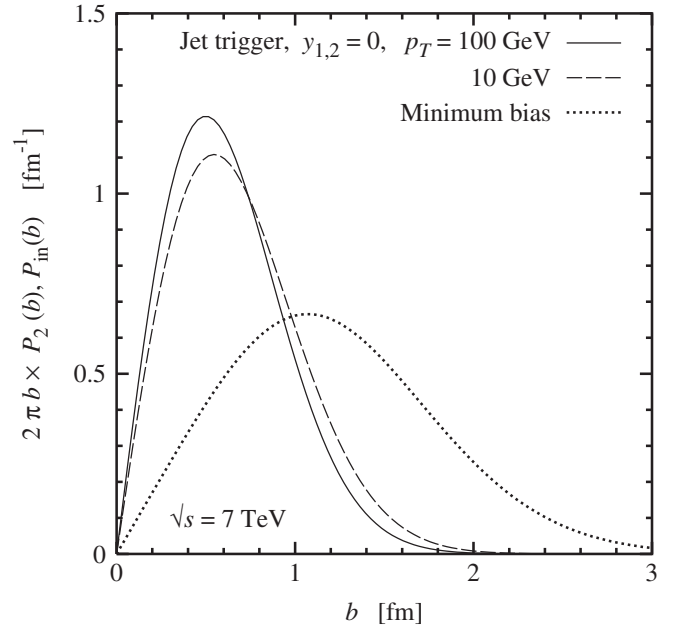
FIG. 4. Impact parameter distributions of inelastic pp collisions at \sqrt{s} = 7 \text{ TeV} . Solid (dashed) line : Distribution of events with a dijet trigger at zero rapidity, y_{1,2} = 0 , cf. Eq. (19), for p_T = 100 (10) \text{ GeV} . Dotted line : Distribution of minimum-bias inelastic events, cf. Eq. (20).
