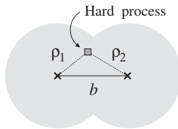
FIG. 3. Overlap integral of the transverse spatial gluon distributions, defining the dependence of the cross section for an inclusive hard gg \rightarrow gg process on the pp impact parameter b , cf. Eqs. (13) and (18). Shown is the transverse view; the momenta of the colliding nucleons point into and out of the plane, respectively.
