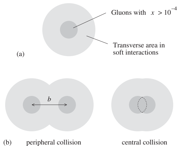
FIG. 1. (a) The two-scale picture of transverse nucleon structure at high energies. The drawing shows the transverse view; the fast nucleon's momentum points in the direction perpendicular to the plane. (b) Implications of the two-scale picture for pp collisions. Peripheral collisions constitute the dominant part of the overall inelastic cross section. Hard processes happen predominantly in central collisions, where the areas occupied by large- x partons overlap. Here the momenta of the colliding nucleons point into and out of the plane, respectively.
