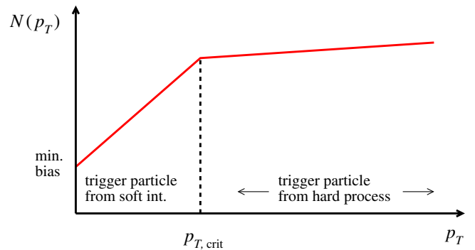
FIG. 6 (color online). Schematic illustration of the expected dependence of the transverse multiplicity, N(p_T) , on the p_T of the trigger.
