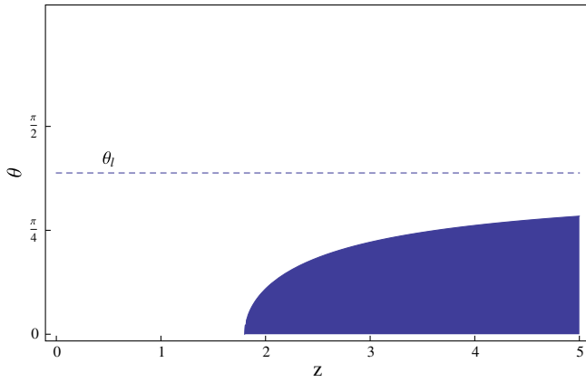
FIG. 3 (color online). Summary of the observable prediction of our model. Assuming the wall is at a redshift z_* \sim 1.8 at its closest position to us in a direction \mathbf{n}_* , then the fine-structure constant is a function of \cos\theta = \mathbf{n}_* \cdot \mathbf{n} and z . The dark (blue) region corresponds to \alpha = \alpha_- and the upper region to \alpha = \alpha_+ . The fact that our observable universe has a finite radius implies that we shall detect no variation for angles larger than \theta_l .
