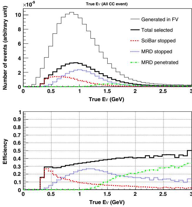
FIG. 8 (color online). (Top panel) Number of CC events in the SciBar FV as a function of true E_\nu , predicted by the NEUT-based simulation. The number of selected events in each subsample is also shown. (Bottom panel) Detection efficiency as a function of true neutrino energy for each subsample.
