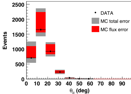
FIG. 7 (color online). Distribution of the reconstructed angle of the muon candidate in the MRD-penetrated sample. The MC prediction is based on NEUT and absolutely normalized by the number of POT. The total and flux systematic errors on the MC predictions are shown separately.
