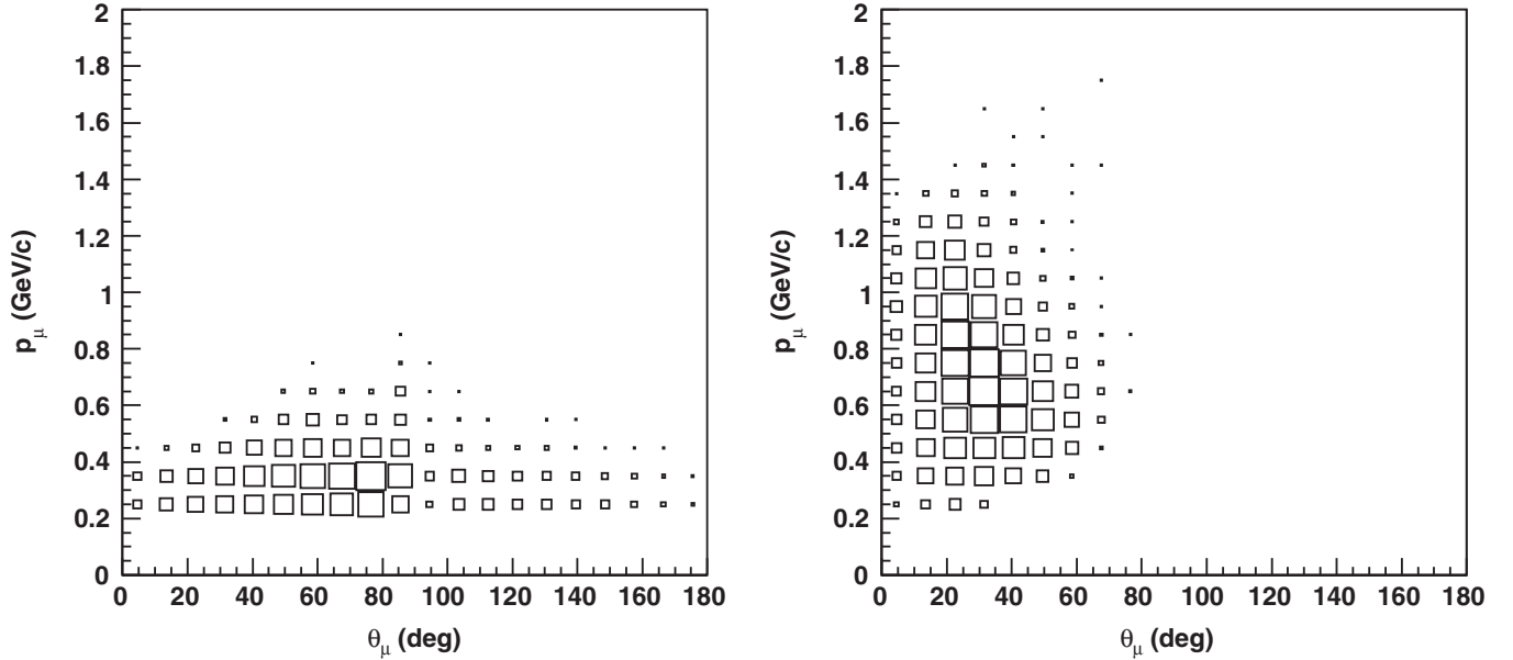
FIG. 10. Data distributions of p_{\mu} vs \theta_{\mu} for the SciBar-stopped (left panel) and MRD-stopped (right panel) samples. The size of the boxes is proportional to the number of entries.
