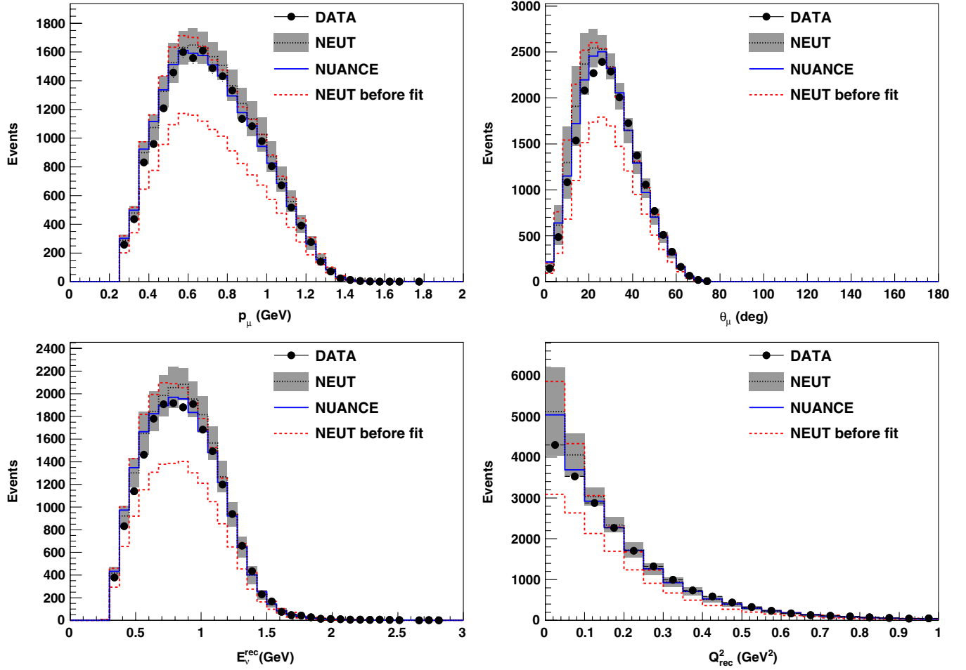
FIG. 14 (color online). Top panels: Reconstructed p_\mu (left) and \theta_\mu (right) of the MRD-stopped sample. Bottom panels: E_\nu^{\text{rec}} (left) and Q_{\text{rec}}^2 (right) of the MRD-stopped sample. The NEUT and NUANCE predictions after the fit are shown, and the predictions are absolutely normalized by the number of POT. The filled regions show the systematic uncertainties of MC predictions based on NEUT. The area within the dashed lines shows the NEUT predictions with their systematic uncertainties before the fit. The systematic uncertainty for the NUANCE prediction is similar to that of the NEUT prediction and is not shown.
