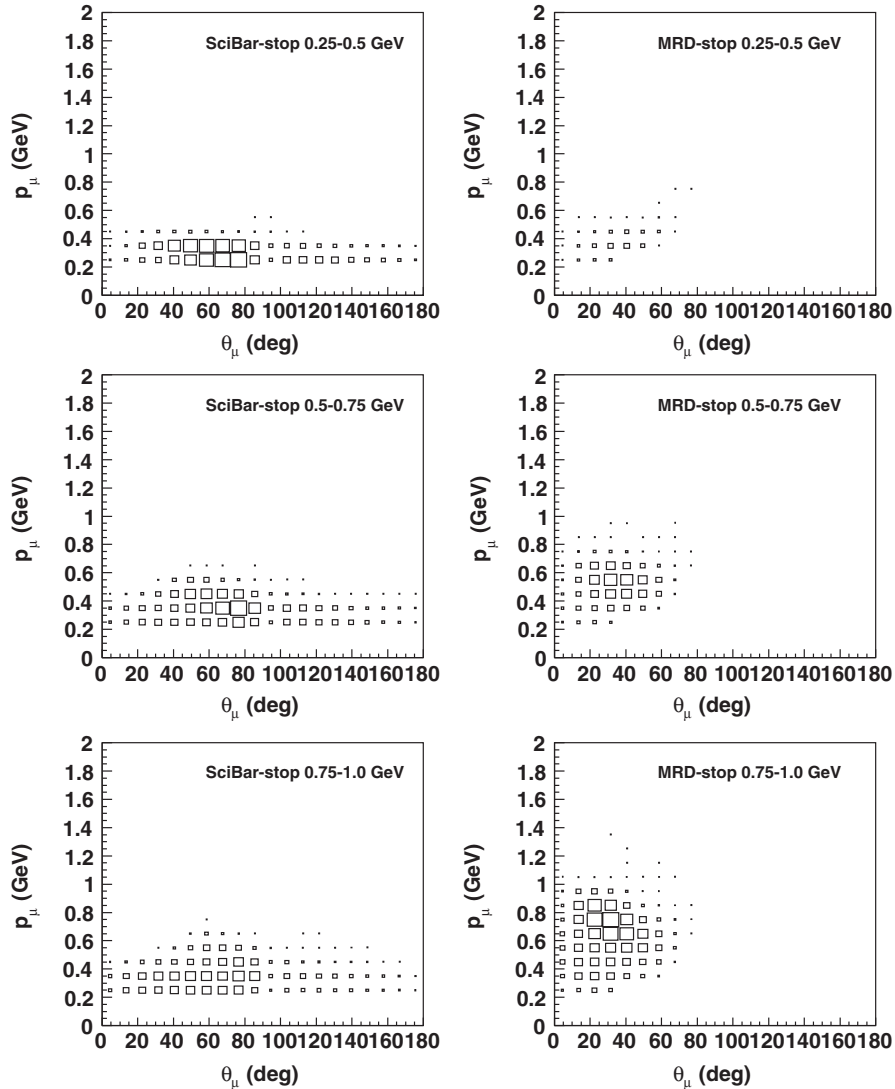
FIG. 11. The MC templates of p_\mu vs \theta_\mu for the SciBar-stopped and MRD-stopped samples for the three lowest E_\nu regions. The normalization factors are common between the SciBar-stopped and MRD-stopped samples.
