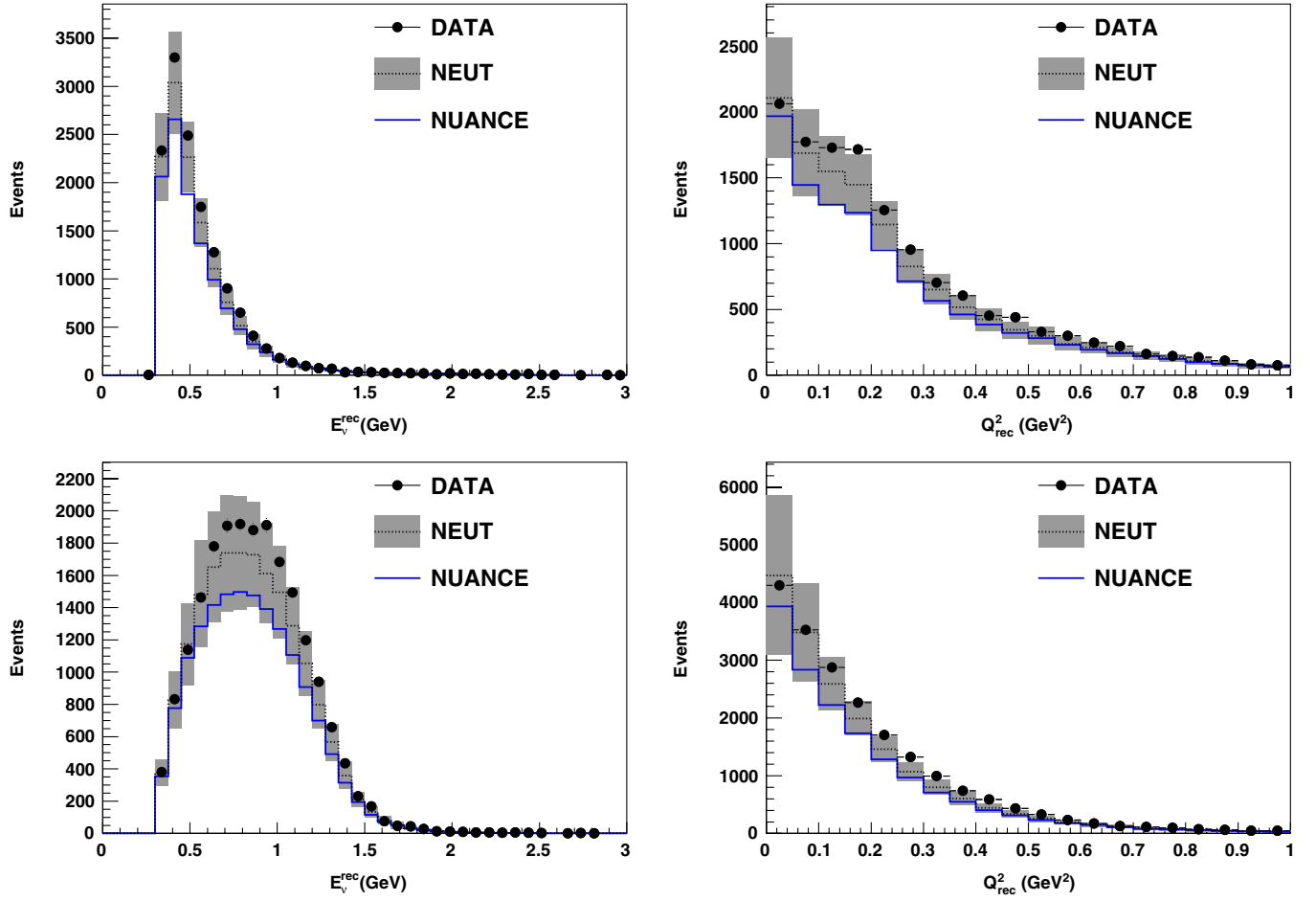
FIG. 9 (color online). Top panels: E_{\nu}^{\text{rec}} (left) and Q_{\text{rec}}^2 (right) of the SciBar-stopped sample. Bottom panels: E_{\nu}^{\text{rec}} (left) and Q_{\text{rec}}^2 (right) of the MRD-stopped sample. The NEUT and NUANCE predictions are absolutely normalized by the number of POT. The filled regions show the systematic uncertainties on the MC predictions based on NEUT. The systematic uncertainty for the NUANCE prediction is similar to that of the NEUT prediction and is not shown.
