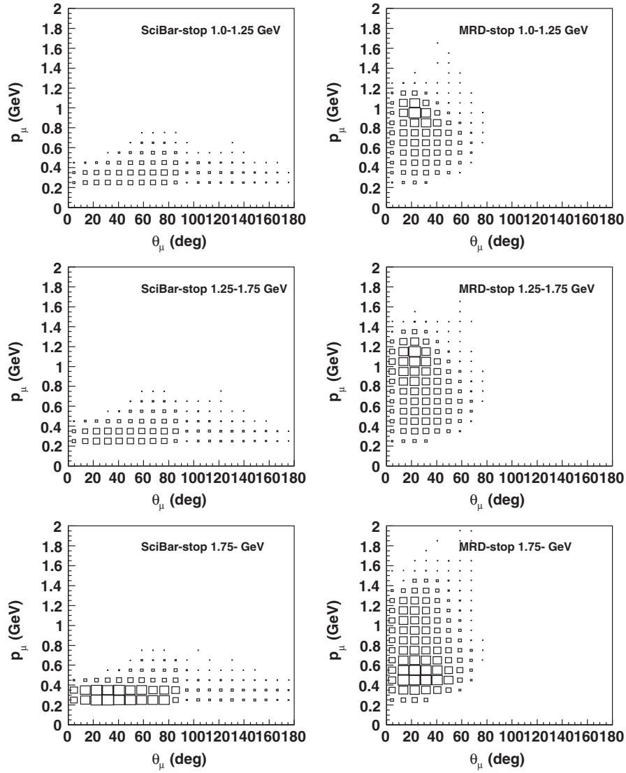
FIG. 12. The MC templates of p_\mu vs \theta_\mu for the SciBar-stopped and MRD-stopped sample for the three highest E_\nu regions. The normalization factors are common between the SciBar-stopped and MRD-stopped samples.
