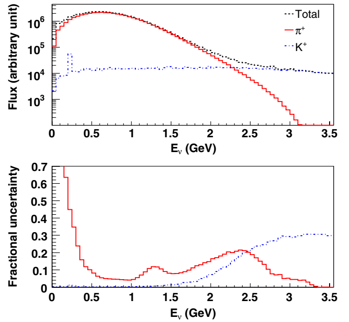
FIG. 2 (color online). (Top panel) \nu_\mu flux prediction at the SciBooNE detector as a function of neutrino energy E_\nu . The total flux and contributions from \pi^+ and K^+ decays are shown. (Bottom panel) Fractional uncertainty of the \nu_\mu flux prediction due to \pi^+ and K^+ production from the p-Be interaction. Additional uncertainties from POT, hadron interactions in the target, and the horn magnetic field are not shown.
