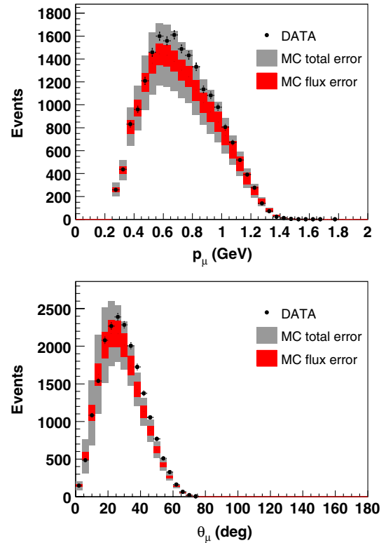
FIG. 6 (color online). Distributions of the reconstructed momentum (top panel) and angle (bottom panel) of the muon candidate in the MRD-stopped sample. The MC prediction is based on NEUT and absolutely normalized by the number of POT. The total and flux systematic errors on the MC predictions are shown separately. The dominant source of the total error is the cross-section uncertainty.
