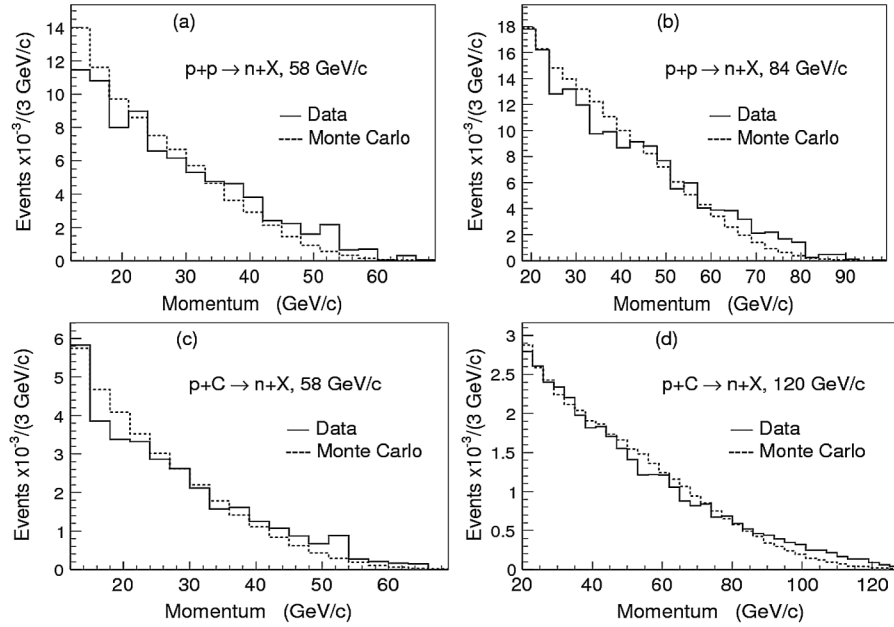
FIG. 12. Comparison of data (solid) with fully reconstructed Monte Carlo (dashed) neutron candidate events. The Monte Carlo events have been normalized to have an equal number of total events and, hence, only the shapes are to be compared in this plot. The agreement in shapes indicates that all the reconstruction and resolution effects have been properly simulated in the Monte Carlo.
