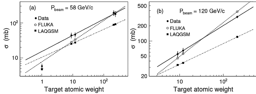
FIG. 17. Comparison of the A dependence of MIPP cross sections with those from Monte Carlos. The lines are fits to the data. The cross sections are for producing neutrons with momentum greater than the threshold and within an angular range of 20.4 mrad. The errors are combined statistical and systematic uncertainties. Note that the hydrogen data point is not included in the fit. The cross sections are not corrected for geometric acceptance.
