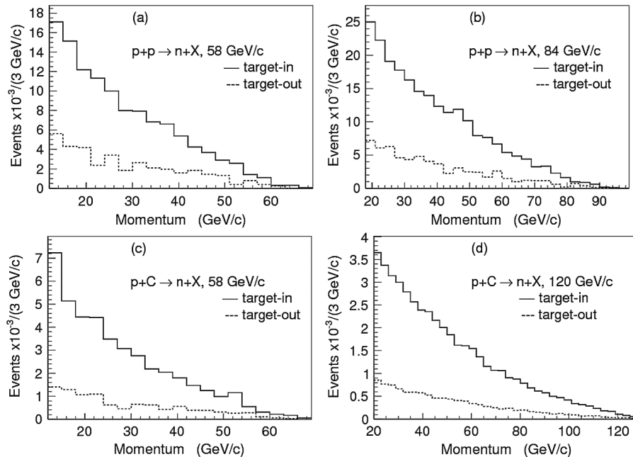
FIG. 8. Raw momentum spectra of neutron candidates before acceptance, trigger, and background corrections. Plots on the top are from the hydrogen target and those on the bottom from the carbon target.
