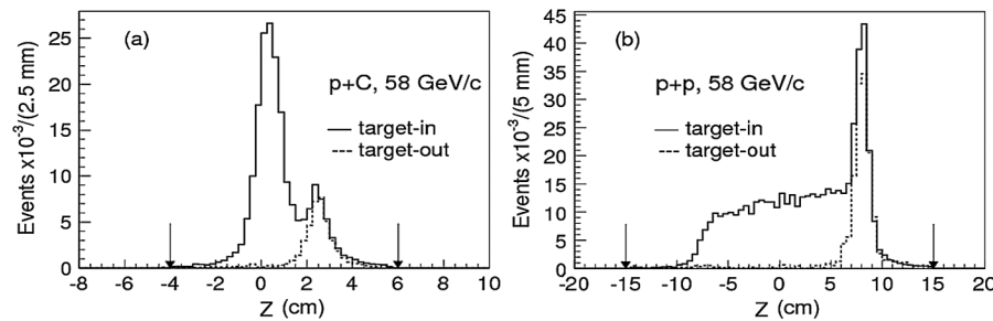
FIG. 5. Longitudinal positions of reconstructed vertices from carbon target (left) and hydrogen target (right). The arrows indicate the location of the selection cuts. The carbon target was 1 cm thick and 5.08 cm in diameter, while the hydrogen target was 14 cm thick and 3.8 cm in diameter.
