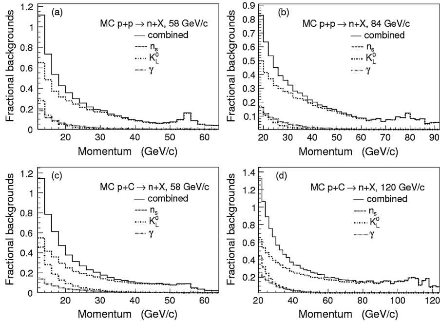
FIG. 11. Typical momentum dependence of backgrounds predicted by the Monte Carlo as a fraction of the predicted neutron production cross section.
