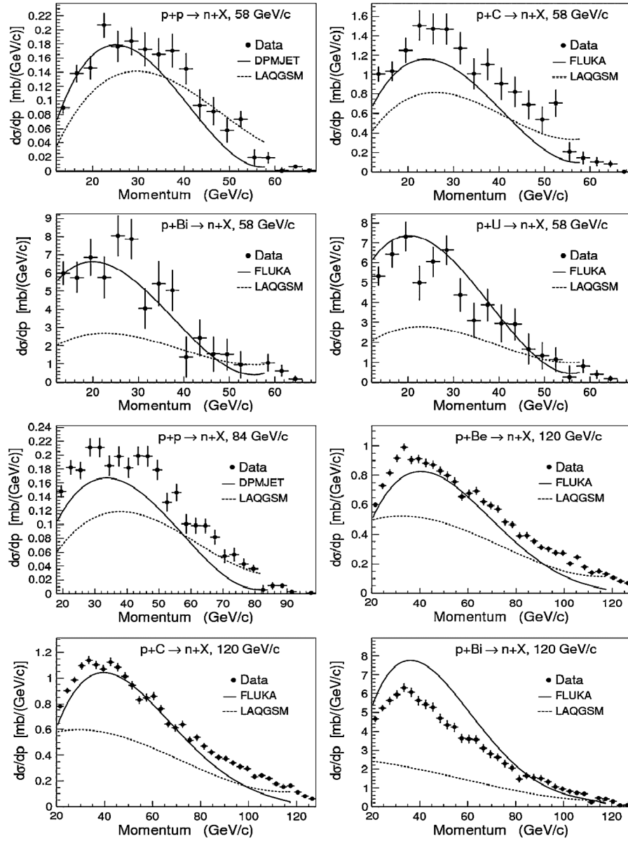
FIG. 16. Measured cross sections from this experiment compared with neutron spectra generated by the DPMJET/FLUKA and LAQGSM Monte Carlos. Data and Monte Carlos are not corrected for geometric acceptance. The error bars are statistical only.
