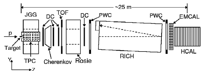
FIG. 1. Experimental layout schematic.
