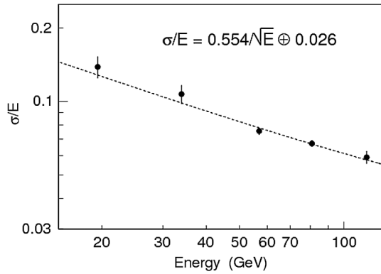
FIG. 3. The fractional energy resolution of the calorimeters as a function of the proton beam energy. The curve represents the fit to \sigma/E = a/\sqrt{E} \oplus b , where E is in GeV. “ \oplus ” indicates addition in quadrature.
