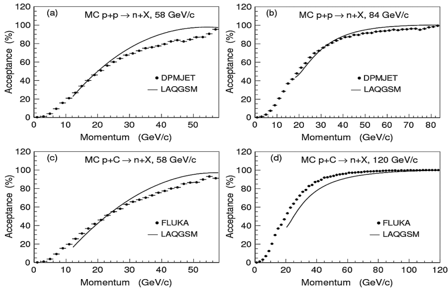
FIG. 15. Geometric acceptance of the calorimeter for neutrons from hydrogen (top) and carbon (bottom) based on DPMJET/FLUKA and LAQGSM models.
