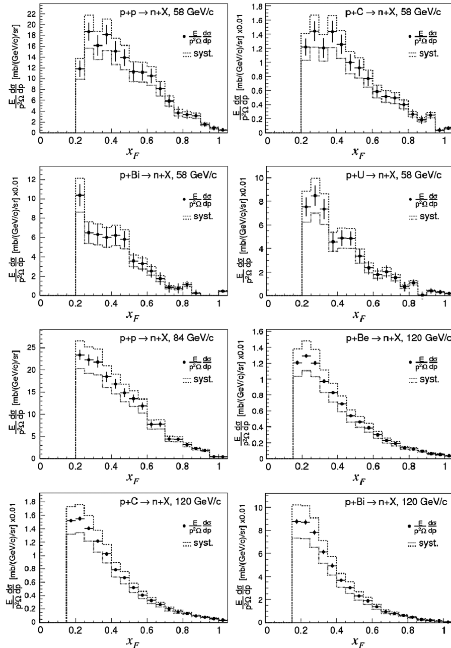
FIG. 18. Lorentz-invariant cross sections as a function of x_F for producing neutrons with momentum greater than threshold within the solid angle of the calorimeter.
