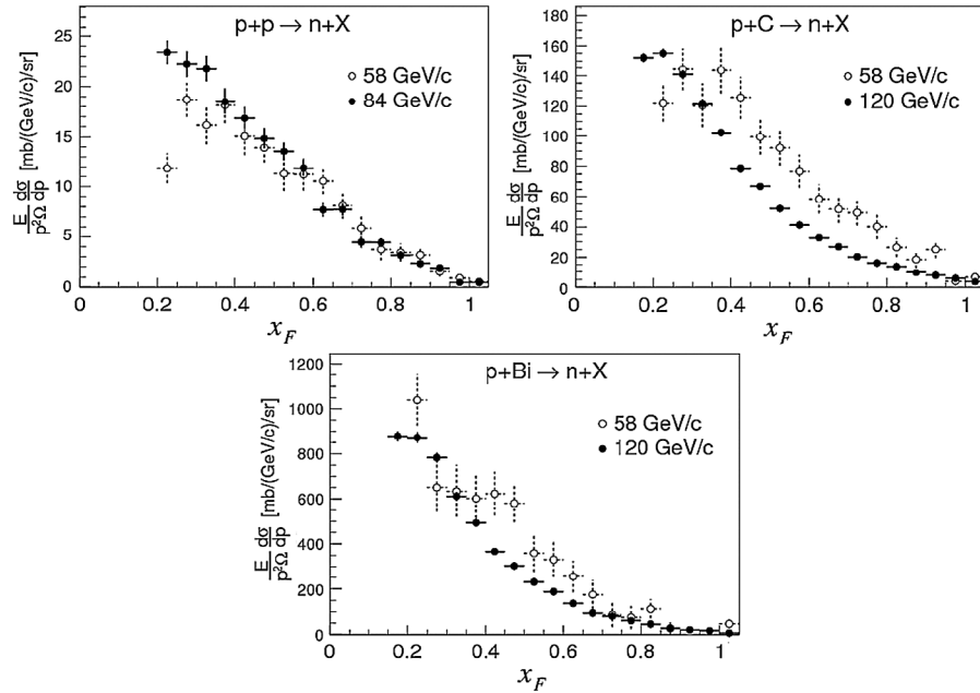
FIG. 19. Lorentz-invariant cross sections as a function of x_F for hydrogen, carbon, and bismuth targets at different incident beam momenta. Errors are statistical only.
