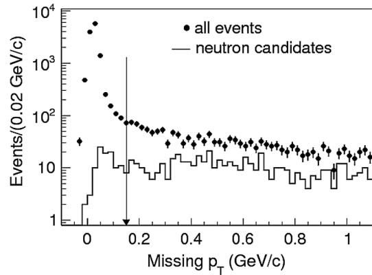
FIG. 6. The difference in transverse momentum between the incident beam particle and the outgoing secondary tracks. The arrow indicates the location of the cut. The peak at 0 represents straight-through beam tracks that were rejected by the cut.
