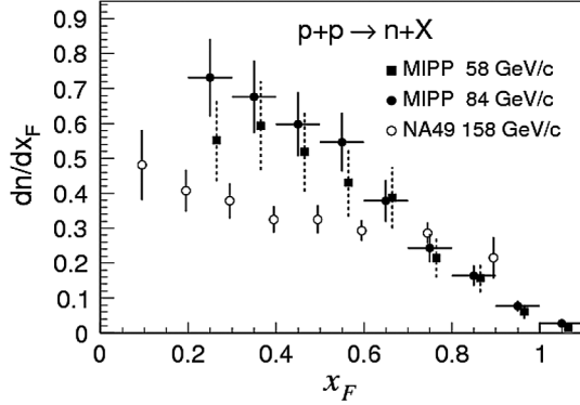
FIG. 21. Comparison of our results (solid points) for 58 and 84 GeV/c incident protons with those from NA49 (open circles). The errors in our data are combined statistical and systematic uncertainties.
