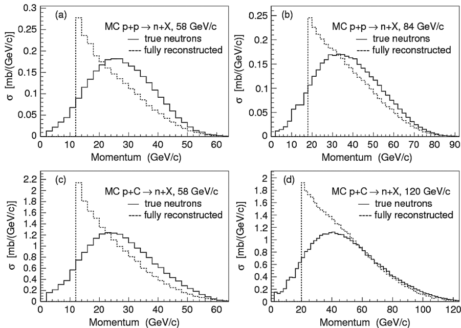
FIG. 13. True neutron spectra generated by Monte Carlo (black) compared with reconstructed neutron candidates from the full Monte Carlo sample (dashed).
