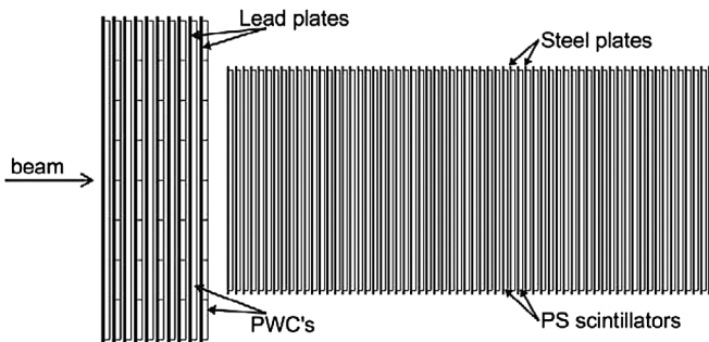
FIG. 2. Schematic of calorimeters (not to scale).
