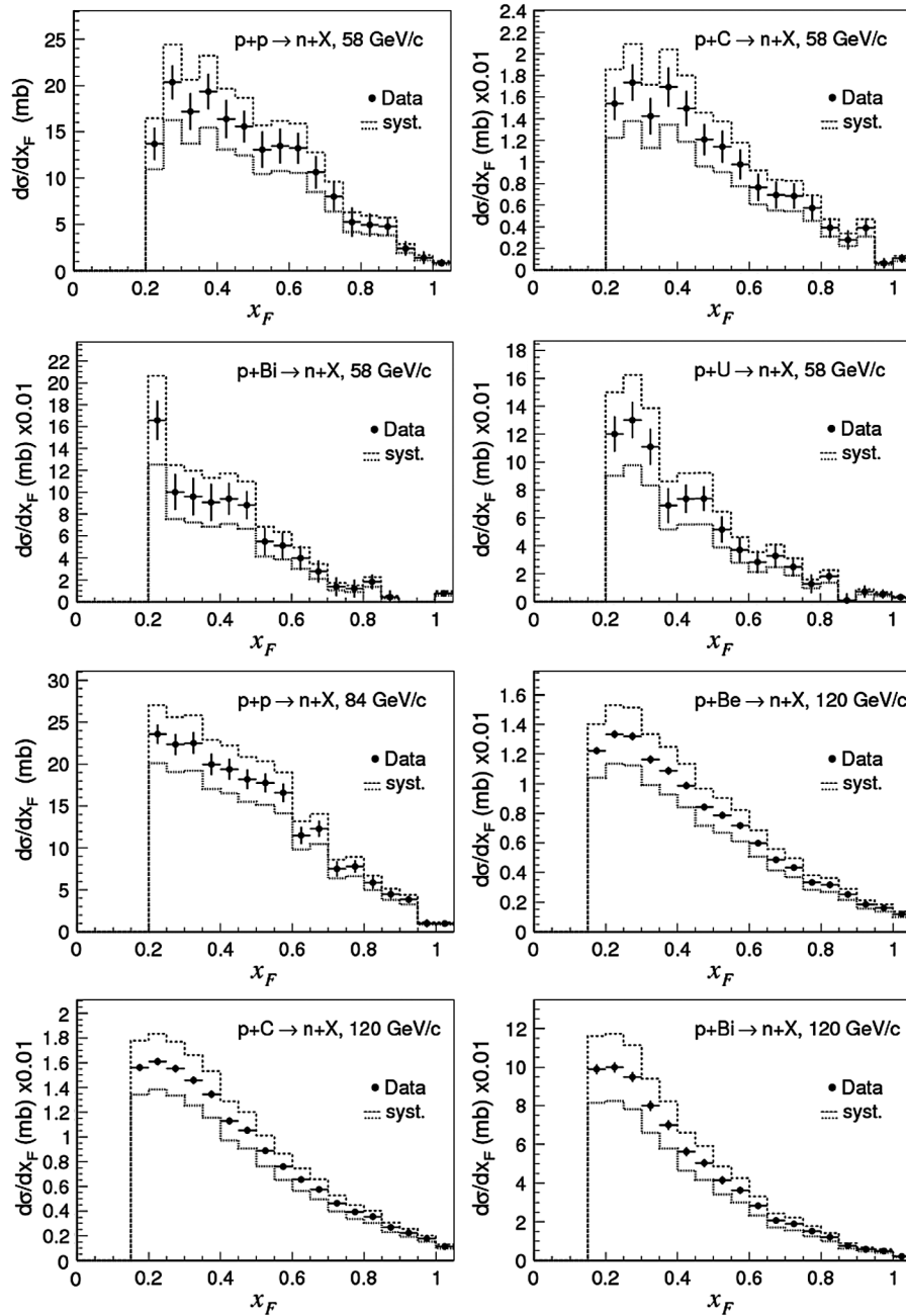
FIG. 20. Total inclusive cross sections as a function of x_F for producing neutrons with momentum greater than the threshold with estimated systematic uncertainties. The difference between these plots and the ones in Fig. 16 is that here we have corrected for the geometric acceptance of the calorimeter.
