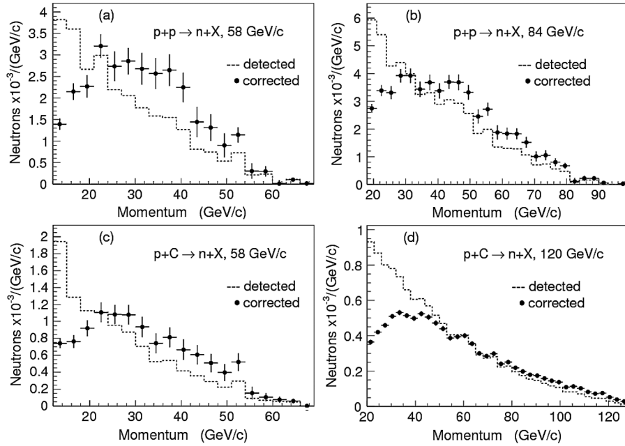
FIG. 14. Neutron spectra from MIPP data after correction. The correction, as described earlier in the section, includes backgrounds, neutron losses, and efficiencies for triggering and selection. The uncertainties are statistical.
