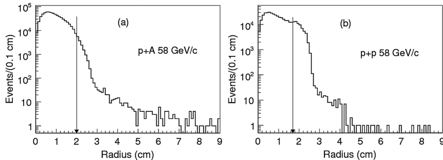
FIG. 4. Radial positions of 58 GeV/c incident protons on solid target (left) and hydrogen target (right), based on beam triggers. The arrows indicate the location of the selection cuts. The profile for the hydrogen target is broader because of additional material just upstream of the target.
