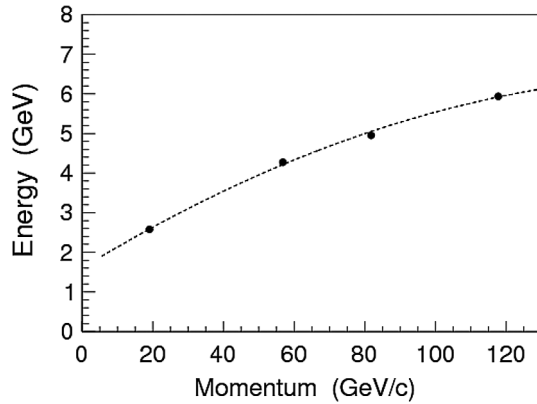
FIG. 7. Average energy loss of protons in the EMCAL. The energy loss of neutrons in the EMCAL was assumed to be similar to that of protons.
