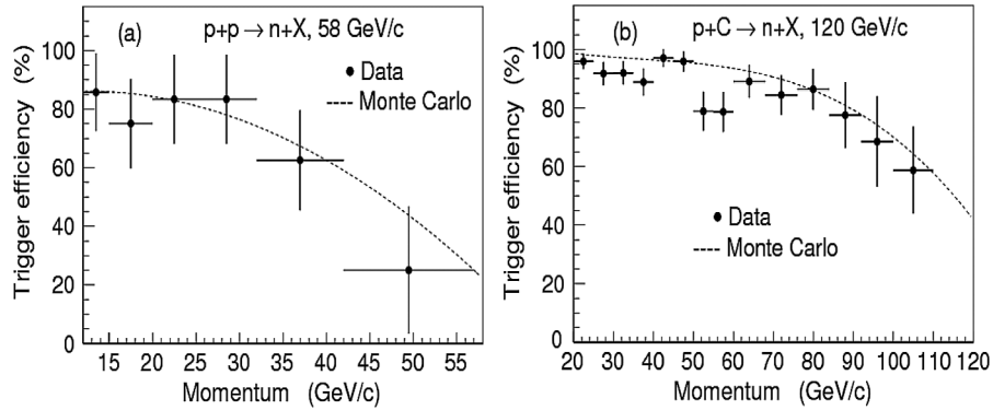
FIG. 9. The SCINT trigger efficiency as a function of neutron momentum for data (solid points) and Monte Carlo (dashed curve). Note that the horizontal axis minimum is at the neutron selection threshold and not at 0.
