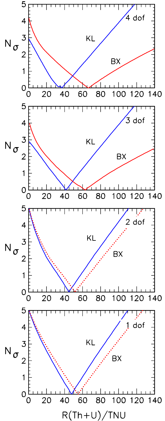
FIG. 6 (color online). KamLAND and Borexino analysis: constraints on the total rate R(\text{Th} + \text{U}) in terms of standard deviations N_\sigma .
