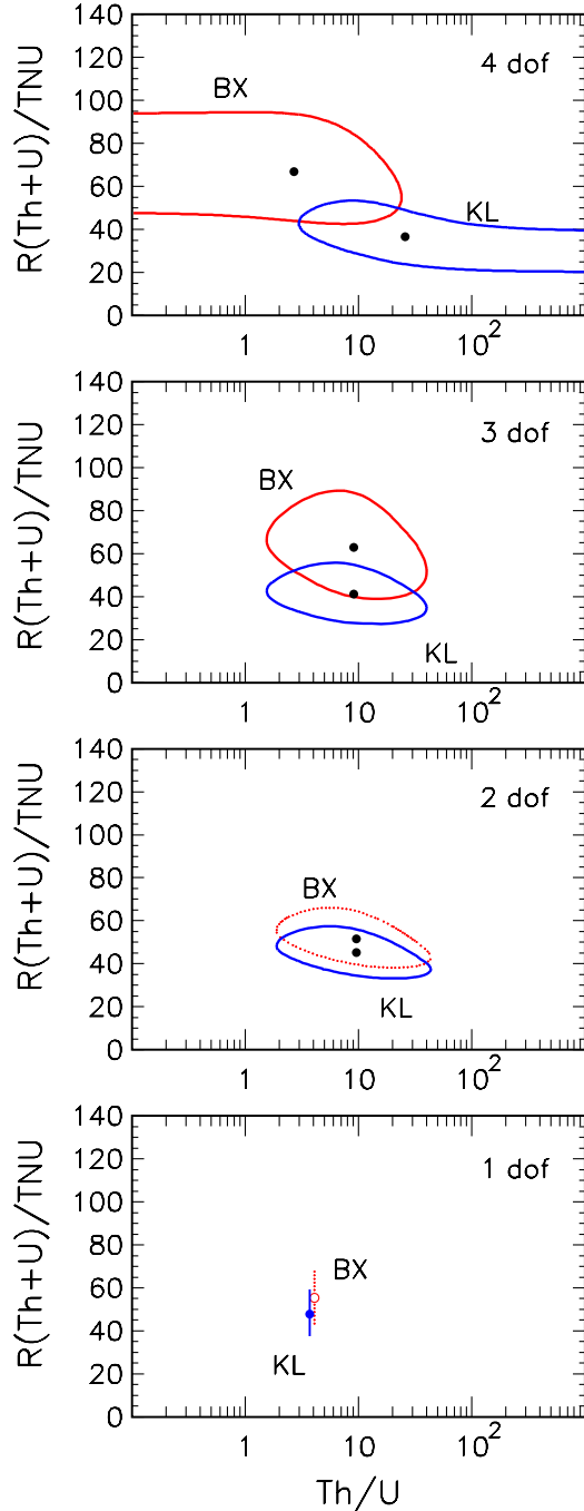
FIG. 4 (color online). KamLAND (KL) and Borexino (BX) geoneutrino analysis in the plane charted by the total rate R(\text{Th} + \text{U}) and by the mass abundance ratio \text{Th}/\text{U} . The curves represent 1\sigma contours ( \Delta\chi^2 = 1 ) around the best-fit points (thick dots). From top to bottom, the degrees of freedom decrease from N_D = 4 to N_D = 1 , as reported in Table I.
