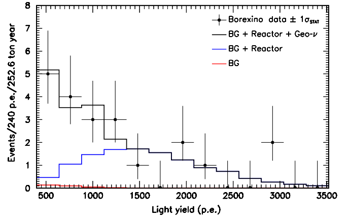
FIG. 3 (color online). Borexino event spectrum as a function of the light yield for positron events (p.e.). Data points and background (BG) estimates are taken from [6]. The histogram represents our best-fit spectrum, with cumulative contributions from background, plus reactor, plus geoneutrino events.
