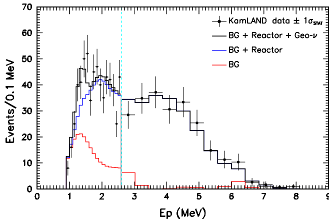
FIG. 2 (color online). KamLAND event spectrum as a function of the observed prompt energy E_p . Data points and background (BG) estimates are taken from [5,25]; note the narrower binning in the geoneutrino energy range E_p < 2.6 MeV [25]. The histogram represents our best-fit spectrum, with cumulative contributions from background, plus reactor, plus geoneutrino events.
