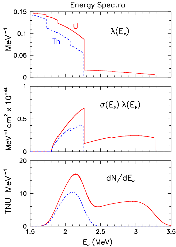
FIG. 1 (color online). Geoneutrino spectra computed in this work, as a function of the neutrino energy E_\nu . Upper panel: spectra from U and Th decay chains (solid and dashed curves, respectively). Middle panel: spectra multiplied by the cross section for inverse beta decay. Lower panel: observable event spectra, including typical energy resolution effects. The results refer to a \bar{\nu}_e flux of 10^6/\text{cm}^2/\text{s} (all panels), and to 10^{32} target protons (lower panel).
