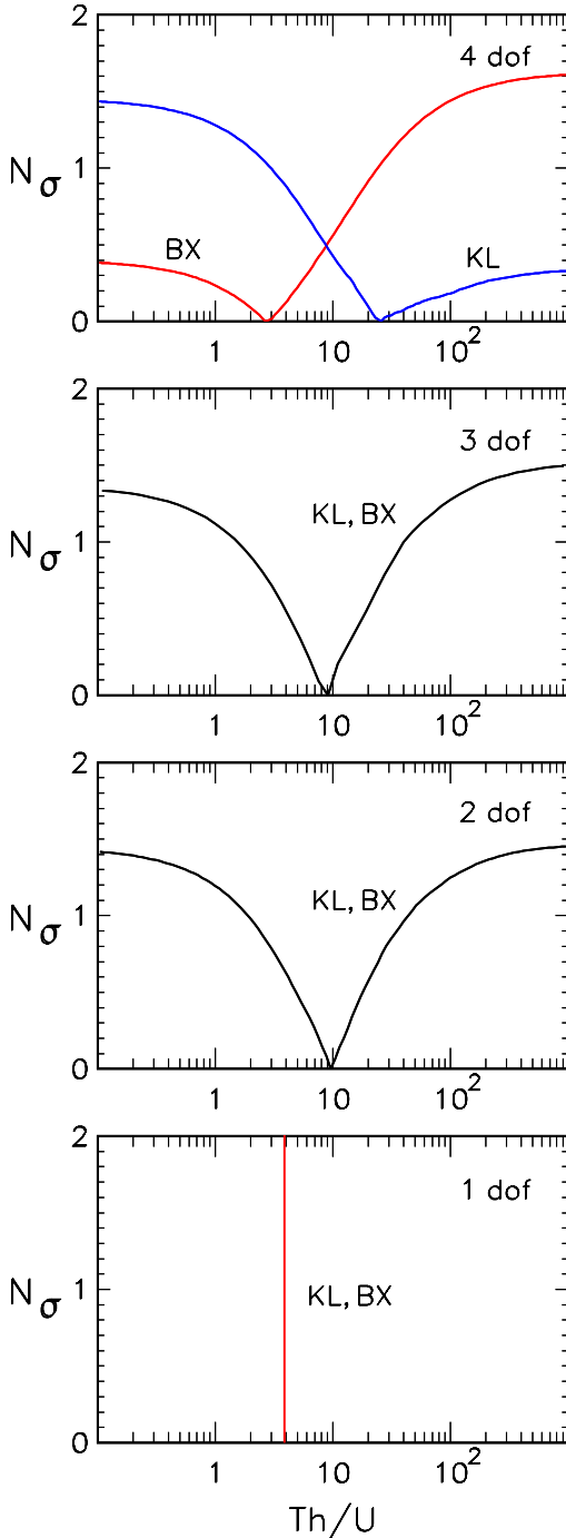
FIG. 5 (color online). KamLAND and Borexino analysis: constraints on the Th/U ratio in terms of standard deviations, N_\sigma = \sqrt{\Delta\chi^2} .
