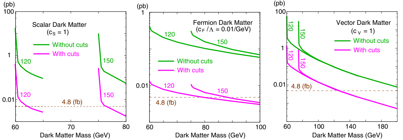
FIG. 3 (color online). Cross section of the dark matter signal at the LHC with and without kinematical cuts in Eq. (20). The parameter m_h and c_{DM} are fixed as shown in these figures.
