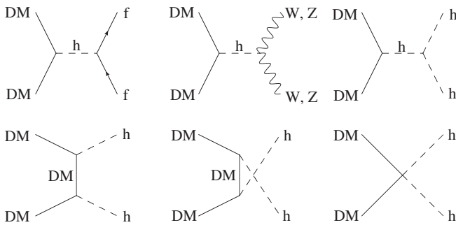
FIG. 1. Feynman diagrams for dark matter annihilation.
