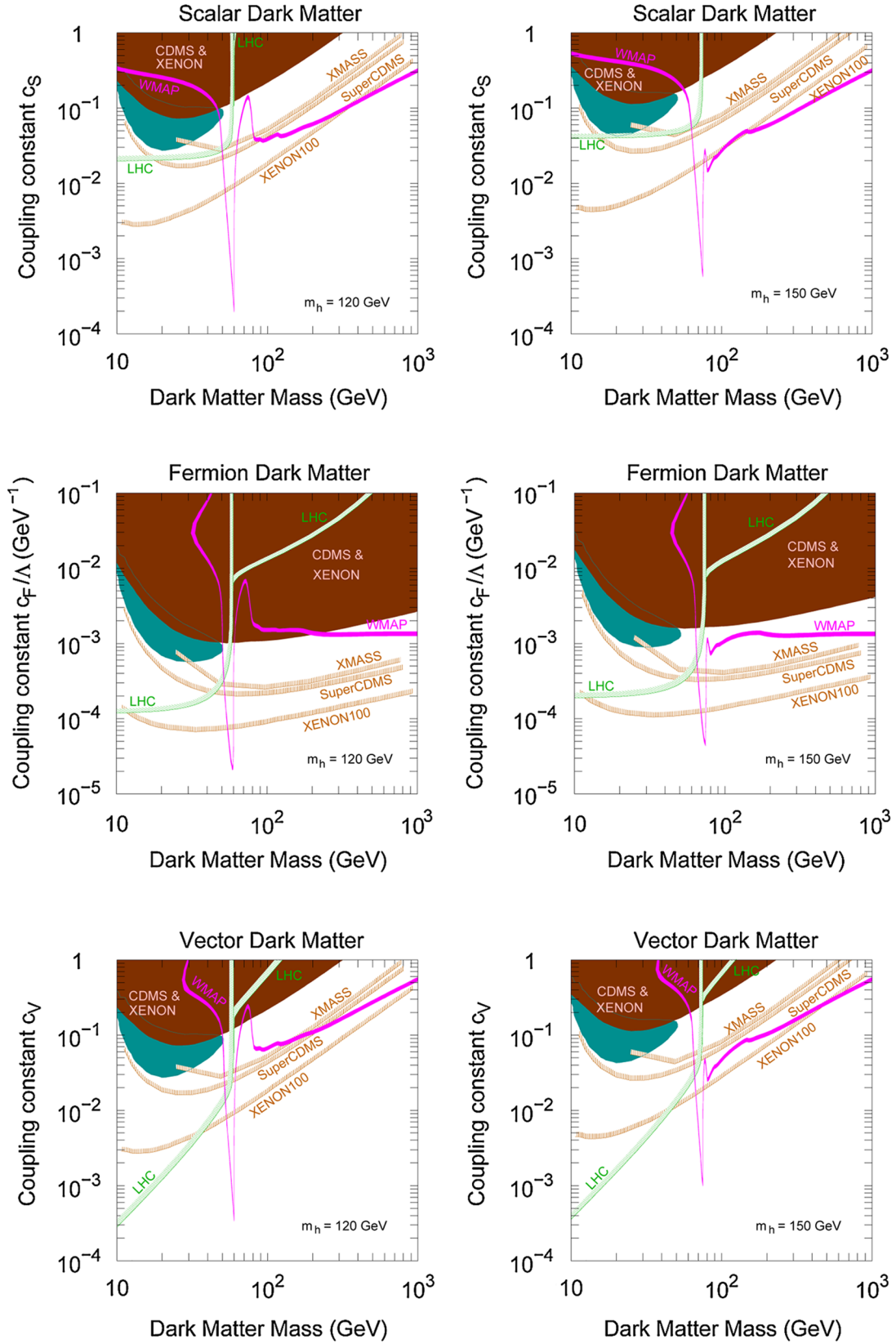
FIG. 2 (color online). Constraints on the nightmare scenario from WMAP, Xenon100 first data, and CDMS-II experiments. Higgs mass is fixed to be 120 GeV in left three figures, while 150 GeV in right three figures. Expected sensitivities to detect the signal of the dark matter at XMASS, SuperCDMS, Xenon100, and LHC experiments are also shown in these figures. See the text for the detail of the region painted by dark cyan (light gray).
