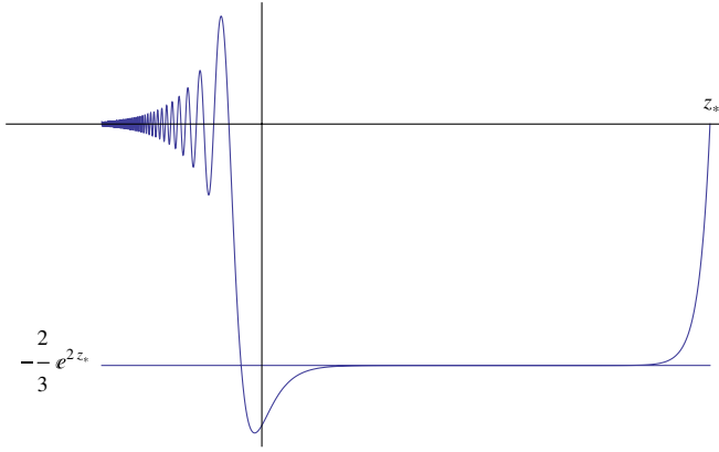
FIG. 2 (color online). The function e^z \tilde{I}(-e^{-z}, -e^{-z_*}) on a linear scale. The axes cross at the point \{0, 0\} . For 0 < z < z_* the function is well approximated by -\frac{2}{3}e^{2z_*} . The frequency of oscillation for z < 0 does not vary much as z_* increases—only the amplitude changes. The plot above was generated using z_* = 15 .
