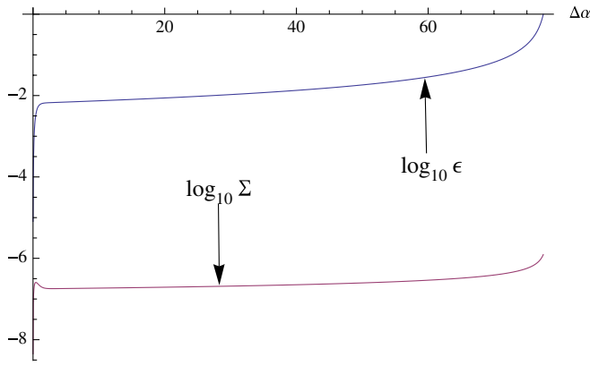
FIG. 1 (color online). Log plot of \Sigma and \epsilon as a function of e -foldings ( \Delta\alpha = \alpha - \alpha_0 ) during inflation. The plot was generated with the potential V = \frac{1}{2}m^2\phi^2 and coupling function f(\phi) = \exp[\frac{\kappa^2\phi^2}{2}] . The initial conditions were \phi_0 = 17.5/\kappa , \phi'_0 = 0 , \alpha_0 = -75 , \beta_0 = 0 , and \beta'_0 = 0 . The constants m and p_A were chosen so that initially \rho_A/\rho_\phi \approx 10^{-6} . Notice that \Sigma very quickly settles to a value that is somewhat smaller than the square of the slow-roll parameter \epsilon .
