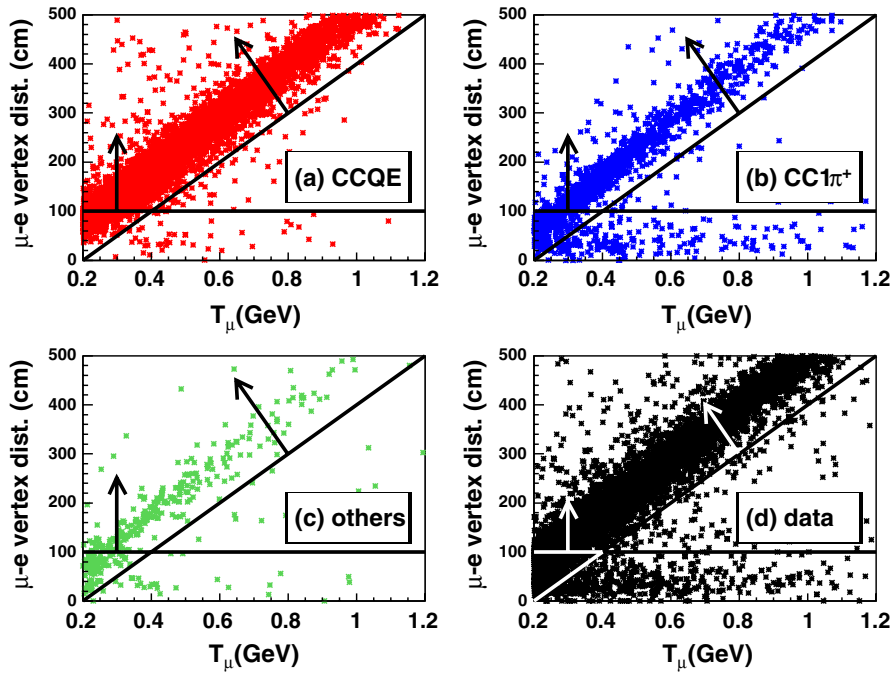
FIG. 6 (color online). Scatter plots of muon-electron vertex distance as a function of reconstructed muon kinetic energy for MC samples: (a) CCQE, (b) CC1\pi^+ , and (c) other channels. The distribution of data is shown in (d). These are events with 2-subevents and with cuts 1–6 applied. The lines with arrows indicate the region selected by the muon-electron vertex distance cut.
