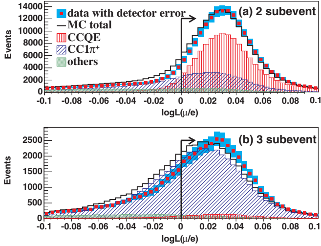
FIG. 5 (color online). Distributions of the \mu/e log-likelihood ratio for the (a) 2 and (b) 3 subevent samples. Data and Monte Carlo simulation (MC) are shown along with the individual MC contributions from CCQE, CC1\pi^+ , and other channels. The lines with arrows indicate events selected by the muon-electron likelihood ratio cut.
