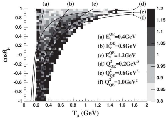
FIG. 11. Ratio of \nu_\mu CCQE data to simulation as a function of reconstructed muon kinetic energy and angle. The simulation includes adjustment of the CC1\pi^+ backgrounds based on MiniBooNE data but is that prior to any CCQE model tuning (it assumes M_A = 1.03 GeV, \kappa = 1 ). The prediction has been normalized to the data. If the simulation modeled the data perfectly, this ratio would be unity. Contours of constant E_\nu and Q^2 are overlaid, and only bins with >20 events in the data are plotted.
