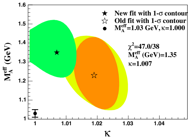
FIG. 9 (color online). The 1\sigma contour plot for the M_A^{\text{eff}} - \kappa fit. The filled star shows the best fit point and 1\sigma contour extracted from this work. The open star indicates the best fit point and 1\sigma contour from the previous work [11]. Two error ellipses are shown for the previous work, the larger reflects the total uncertainty ultimately included in Ref. [11]. The circle indicates the world-average value for M_A [9].
