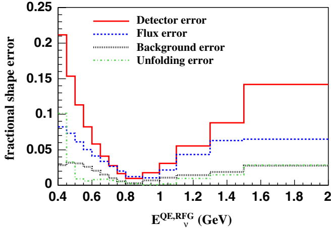
FIG. 16 (color online). Fractional shape error on the MiniBooNE \nu_\mu CCQE flux-unfolded cross section separated into major components. The overall normalization error of 10.7% is not shown.
