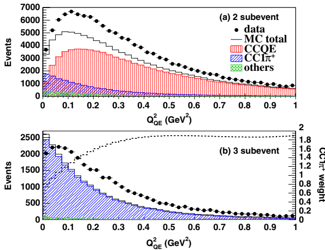
FIG. 7 (color online). Distribution of events in Q_{QE}^2 for the (a) 2 and (b) 3 subevent samples before the application of the CC1 \pi^+ background correction. Data and MC samples are shown along with the individual MC contributions from CCQE, CC1 \pi^+ , and other channels. In (b), the dashed line shows the CC1 \pi^+ reweighting function (with the y-axis scale on the right) as determined from the background fit procedure.
