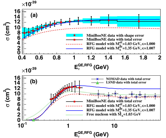
FIG. 15 (color online). Flux-unfolded MiniBooNE \nu_\mu CCQE cross section per neutron as a function of neutrino energy. In (a), shape errors are shown as shaded boxes along with the total errors as bars. In (b), a larger energy range is shown along with results from the LSND [56] and NOMAD [10] experiments. Also shown are predictions from the NUANCE simulation for an RFG model with two different parameter variations and for scattering from free nucleons with the world-average M_A value. Numerical values are provided in Table X in the appendix.
