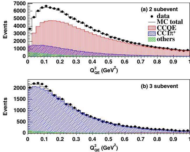
FIG. 8 (color online). Distribution of events in Q_{QE}^2 for the (a) 2 and (b) 3 subevent samples after the application of the data-based CC1\pi^+ background constraint and the new CCQE model parameters M_A^{\text{eff}} and \kappa as determined from the CCQE fit procedure described in the text.
