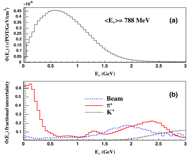
FIG. 2 (color online). Predicted \nu_\mu flux at the MiniBooNE detector (a) along with the fractional uncertainties grouped into various contributions (b). The integrated flux is 5.16 \times 10^{-10} \nu_\mu/\text{POT}/\text{cm}^2 ( 0 < E_\nu < 3 GeV) with a mean energy of 788 MeV. Numerical values corresponding to the top plot are provided in Table V in the appendix.
