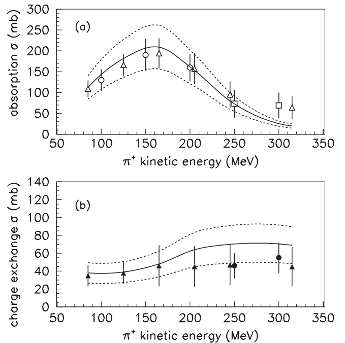
FIG. 3. A comparison of relevant data [25] with the NUANCE model (solid lines) for intranuclear pion (a) absorption and (b) charge exchange as a function of pion kinetic energy. The dotted lines show the 25% (30%) systematic error bands assumed for the pion absorption (charge-exchange) cross sections.
