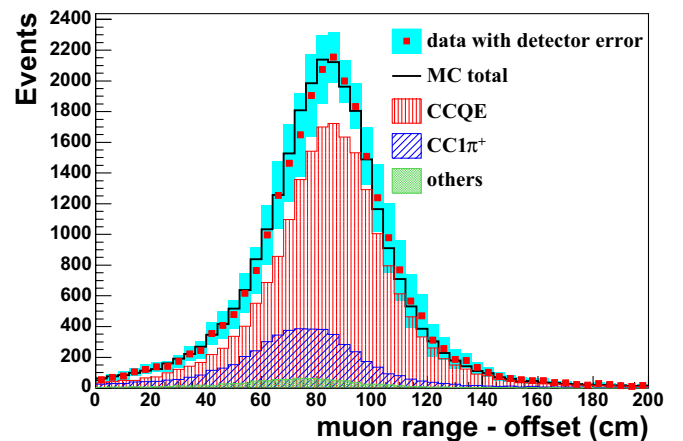
FIG. 10 (color online). Distributions, for both data and simulation, of the measured muon range for muons with 400 < T_\mu < 500 MeV. The subtracted offset, (500 \times T_\mu(\text{GeV}) - 100) cm, corresponds to the solid diagonal line in Fig. 6.
