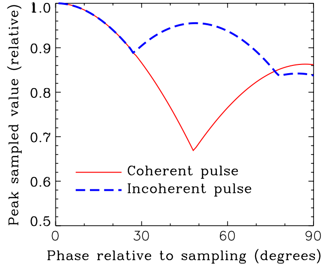
FIG. 6 (color online). (color online) Maximum sampled value as a fraction of the true pulse height as a function of the arbitrary phase offset for sampling rate of 2.048 Gs/s and two extreme lunar Cherenkov pulse types.
