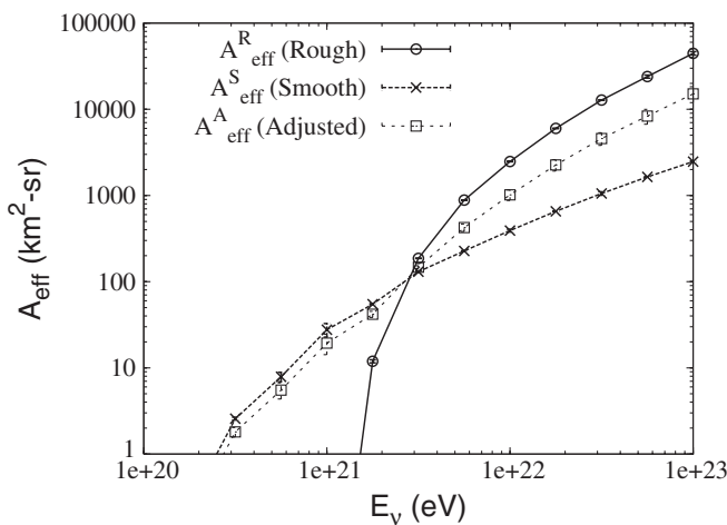
FIG. 17. Effective apertures of a fictitious experiment, calculated using large-scale roughness only ( A_{\text{eff}}^S ), our small-scale roughness approximation ( A_{\text{eff}}^R ), and an adjusted aperture which is a linear combination of them both ( A_{\text{eff}}^A —see Sec. B 2).
