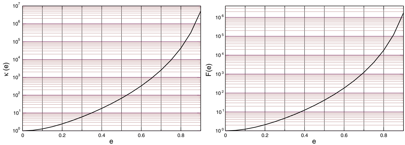
FIG. 6 (color online). Enhancement functions \kappa(e) and F(e) in the evolution of n at 3PN order.
