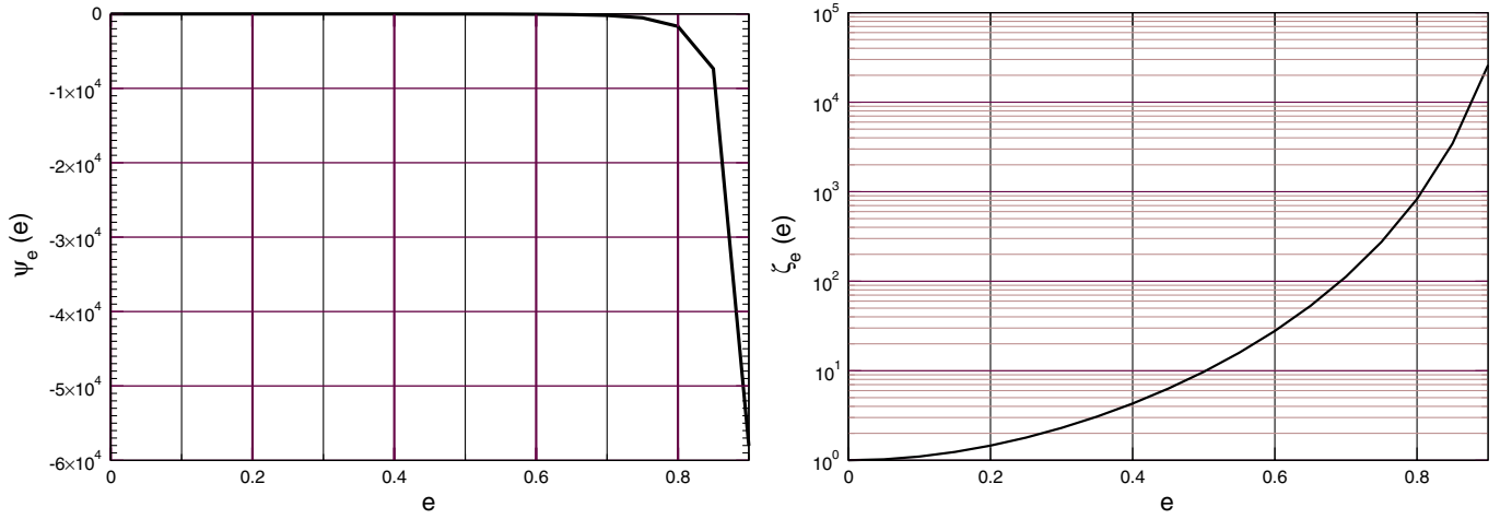
FIG. 7 (color online). Enhancement functions \psi_e(e) and \zeta_e(e) in the evolution of e_t at 2.5PN order. Note the similarity of \psi_e(e) with \tilde{\psi}(e) in Fig. 2.
