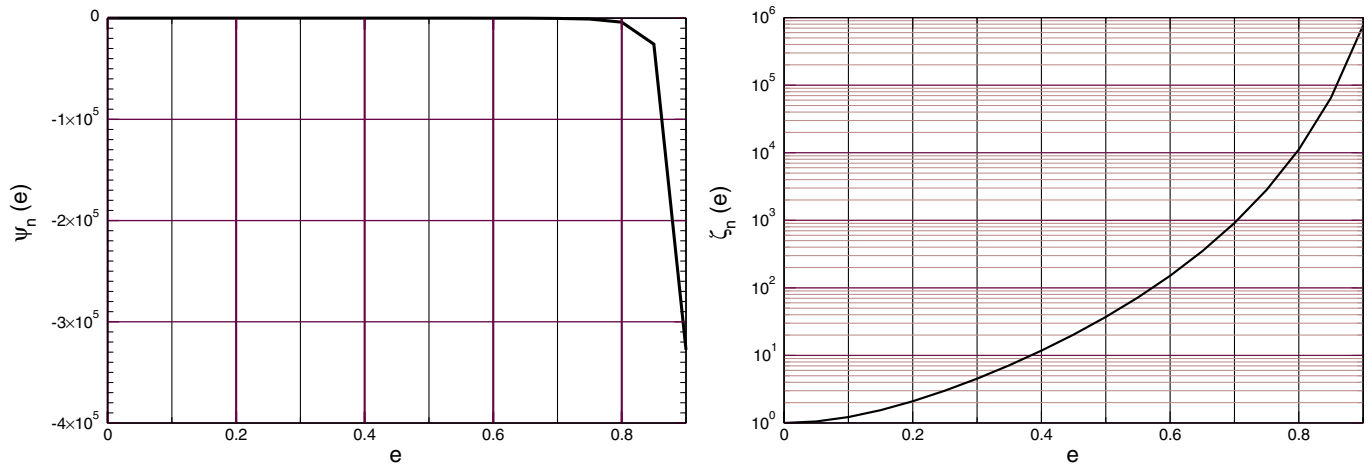
FIG. 5 (color online). Enhancement functions \psi_n(e) and \zeta_n(e) in the evolution of n at 2.5PN order. Note the similarity of \psi_n(e) with \tilde{\psi}(e) in Fig. 2.
