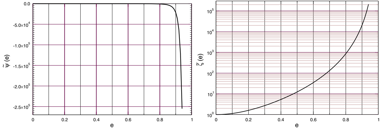
FIG. 2 (color online). Enhancement functions \tilde{\psi}(e) and \tilde{\zeta}(e) in the angular-momentum flux at 2.5PN order.
