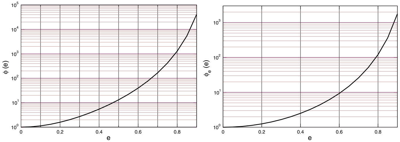
FIG. 4 (color online). Enhancement functions \varphi(e) and \varphi_e(e) in the evolutions of n and e_t at 1.5PN order.
