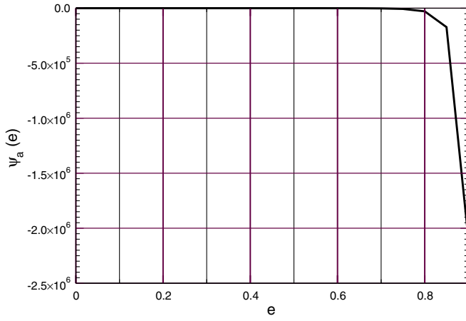
FIG. 10 (color online). Enhancement function \psi_a(e) in the evolution of a_r at 2.5PN order. The other function \zeta_a(e) at 2.5PN order is the same as \zeta_n(e) and hence is not plotted. Similarly at 3PN order it involves the same functions \kappa(e) and F(e) as for n . Note the similarity of \psi_a(e) with \tilde{\psi}(e) in Fig. 2.
