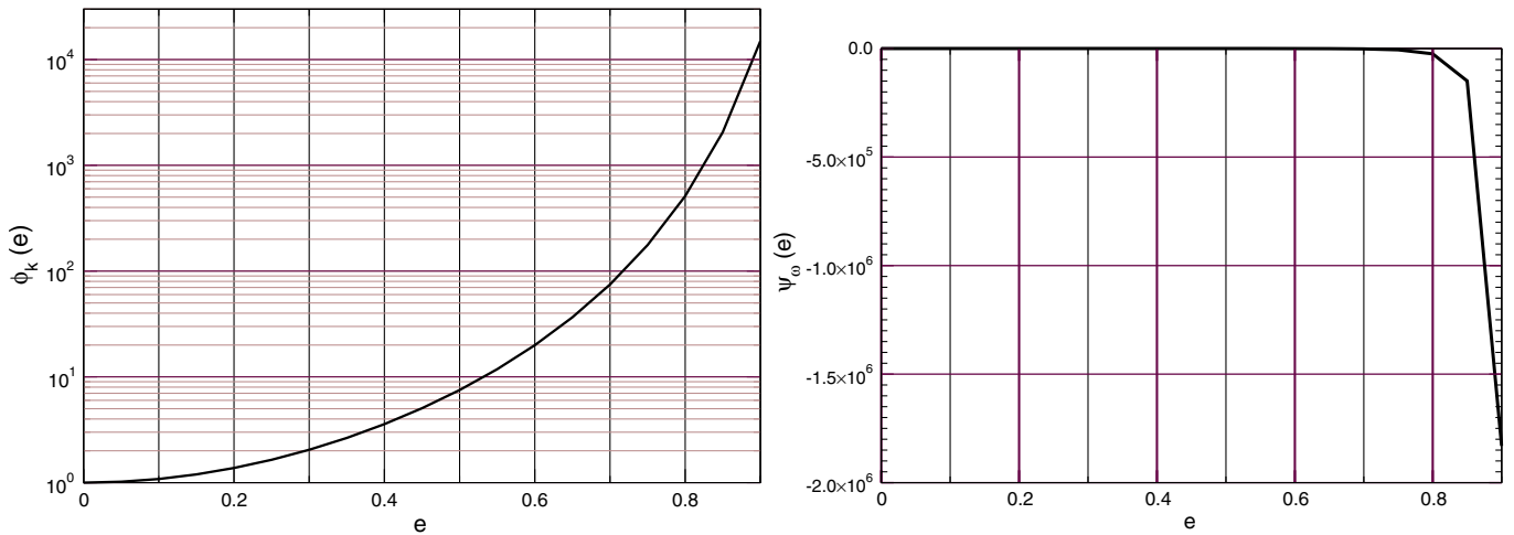
FIG. 9 (color online). Enhancement functions \phi_k(e) and \psi_\omega(e) in the evolution of k and \omega at 1.5PN and 2.5PN orders. Note the similarity of \psi_\omega(e) with \tilde{\psi}(e) in Fig. 2.
