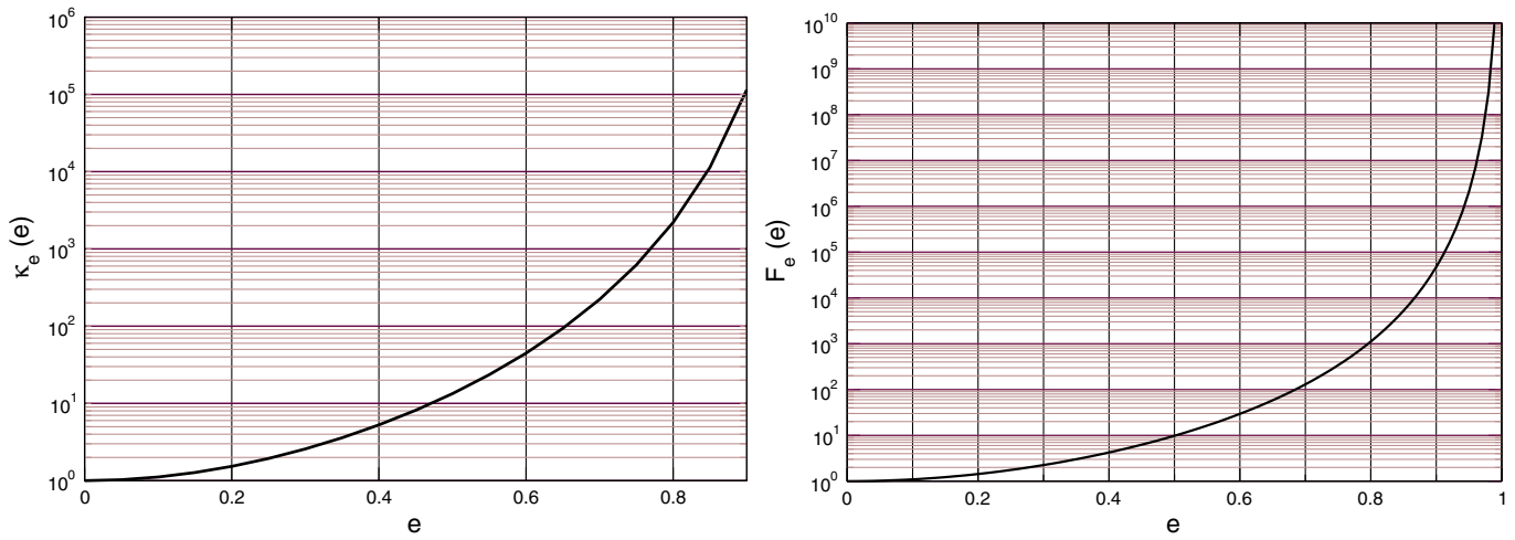
FIG. 8 (color online). Enhancement functions \kappa_e(e) and F_e(e) in the evolution of e_t at 3PN order.
