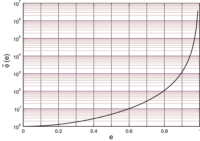
FIG. 1 (color online). Enhancement function \tilde{\varphi}(e) in the angular-momentum flux at 1.5PN order.
