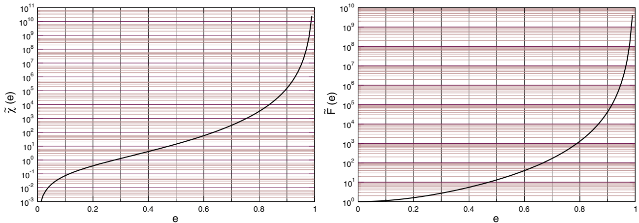
FIG. 3 (color online). Enhancement functions \tilde{\chi}(e) and \tilde{F}(e) in the angular-momentum flux at 3PN order.
