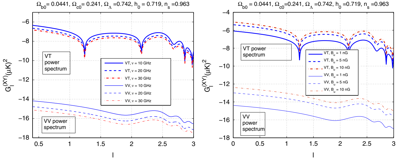
FIG. 1 (color online). In the plot at the left the VT and the VV angular power spectra are reported for a fixed value of B_u (i.e., 1 nG) but for different values of the comoving frequency. In the plot at the right the comoving frequency is fixed to 10 GHz but the magnetic field strength increases. The thin lines denote the VV correlations while the thick lines denote the VT correlations. In the plots, on both axes, the common logarithm of the corresponding quantity is reported.
