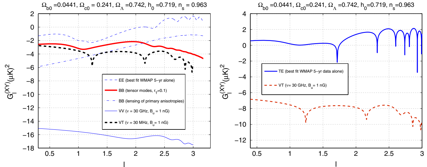
FIG. 2 (color online). The V -mode power spectra are compared with the linear polarizations. As in Fig. 1 on both axes the common logarithm of the indicated quantity is reported.
