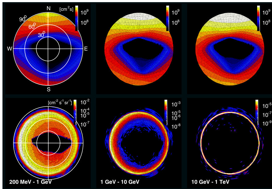
FIG. 1 (color online). Two-dimensional maps of exposure (top row) and intensity (bottom row) for three different energy bands. The coordinate system in these maps is a polar representation such that the nadir direction (i.e., looking down towards the center of the Earth) with \Theta_{\text{nadir}} = 0^\circ is at the center of the plot. \Theta_{\text{nadir}} is increasing in radial direction with the edge of the plot towards the horizon at \Theta_{\text{nadir}} = 90^\circ . The north pole is to the top and west is to the left. The exposure maps are given in units of \text{cm}^2 \text{s} , the intensity maps in units of \text{cm}^{-2} \text{s}^{-1} \text{sr}^{-1} .
