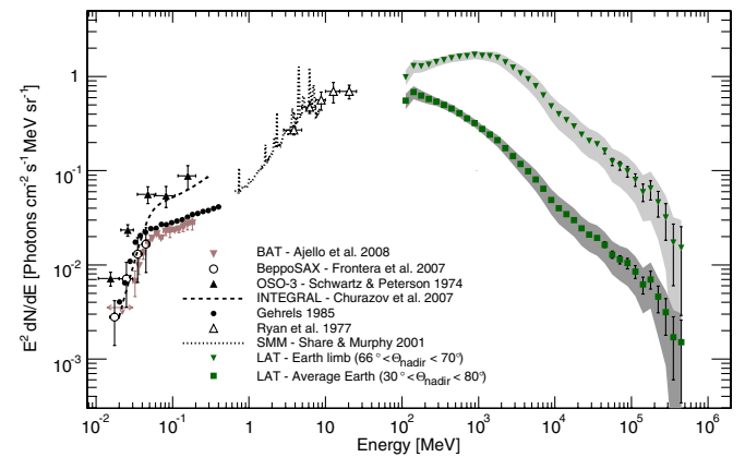
FIG. 7 (color online). Energy intensity for the Earth-originating \gamma rays from keV to 500 GeV energies. The measurements from different instruments are not readily comparable since they have been taken in different points in the solar cycle and are also integrated over different areas of the Earth. Data points are taken from Ryan et al. , Share and Murphy [12], Ajello et al. [26], Frontera et al. [27], Schwartz and Peterson [28], Churazov et al. [29], Gehrels [30].
