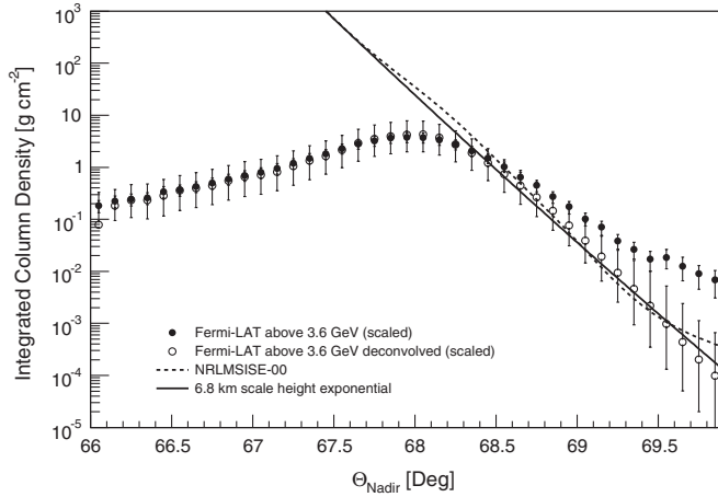
FIG. 5. Comparison between the integrated column density with the LAT-detected gamma-ray intensity as a function of nadir angle for events above 3.6 GeV. Two different model atmospheric profiles have been used: a simple barometric atmosphere with scale height of 6.8 km [22] shown as a solid line and a more realistic atmospheric model from [23]. Shown are the measured gamma-ray intensity (solid circles) and the gamma-ray intensity deconvolved by the PSF of the median energy (4.7 GeV) of this data set (open circles). A good correspondence between the \gamma -ray intensity and the column density can be seen at angles \Theta_{\text{Nadir}} \gtrsim 68.3^\circ . For these angles the atmosphere is thin enough (column density < 10 \text{ g cm}^{-2} ) so that no significant attenuation occurs and the \gamma rays are directly related to the amount of target material for the incoming cosmic rays. The absolute level of the \gamma -ray intensity has been scaled to match the column density for the barometric atmosphere model.
