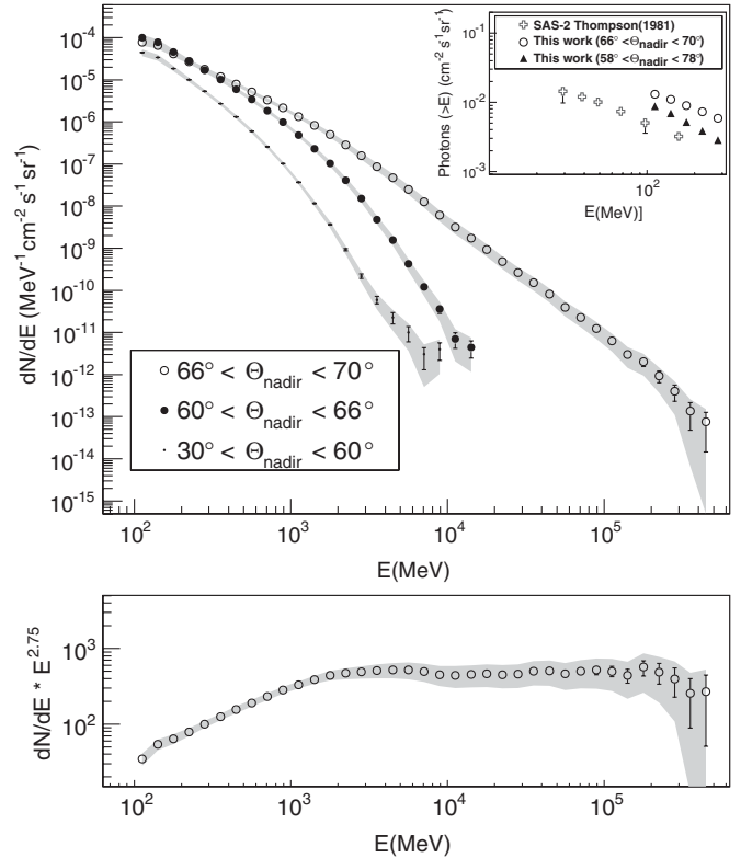
FIG. 2. The top panel shows the differential energy spectrum for the \gamma rays produced in the Earth's atmosphere taken in different \Theta_{\text{nadir}} bands. The spectrum of the limb (open circles) shows a power-law behavior. Also shown are \gamma -ray spectra for the inner parts of the Earth's disk (filled circles and points). Indicated are both statistical and systematic errors (grey band), the latter derived from studies of the Vela pulsar. The inset shows a comparison to previous data by the SAS-2 satellite [13]. To allow for a direct comparison, the limb spectrum is also shown for a larger integration region ( 58^\circ < \Theta_{\text{nadir}} < 78^\circ ) corresponding to the SAS-2 measurement. The bottom panel shows the limb spectrum multiplied by energy to the power 2.75.
