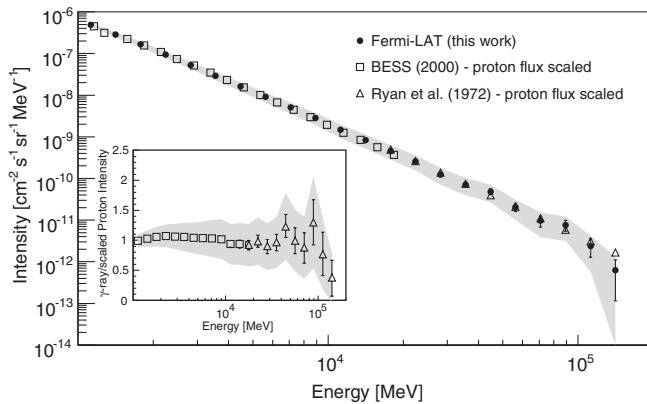
FIG. 6. A comparison of the measured gamma-ray intensity for the angular interval 68.6^\circ < \Theta_{\text{nadir}} < 69.6^\circ (thin-target case, gamma-ray attenuation is insignificant) with the scaled cosmic-ray proton intensity (see text for details). The inset shows the ratio between the \gamma -ray data and the scaled proton data and shows the general good match between the two measurements. The data have been taken from Sanuki et al. [18] and Ryan, Ormes, and Balasubrahmanyam [17].
