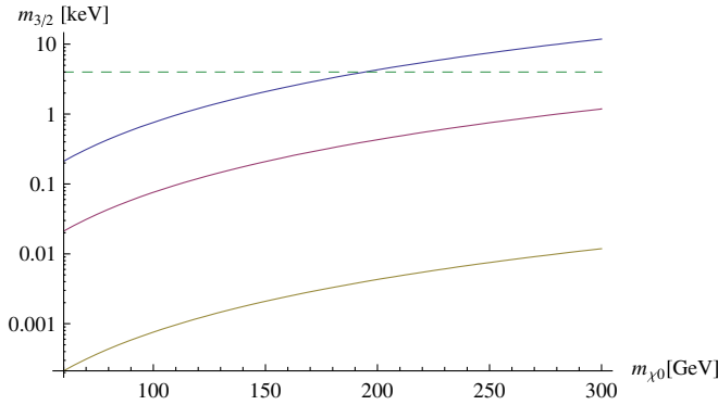
FIG. 7 (color online). Contours of fixed \chi^0 lifetimes in the m_{\chi^0} - m_{3/2} plane as in Eq. (15). The solid curves correspond, from top to bottom, to c\tau_{\chi^0} = 10 m, 10 cm, 10 \mu m. The dashed line indicates the warm dark matter constraint m_{3/2} > 4 keV [26].
