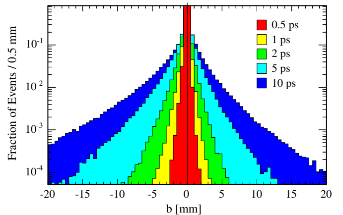
FIG. 4 (color online). The distribution of impact parameters b_i in mm at the LHC in processes Eq. (4) for different stop lifetimes. The curves with b_i > 0 (< 0) refer to the stop in each event with larger (smaller) charm p_T .
