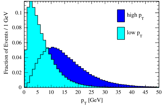
FIG. 5 (color online). The p_T distributions of the charm quarks stemming from the decays of light stops produced in processes Eq. (4) for m_{\tilde{t}} = 100 GeV, m_{\tilde{g}} = 500 and \Delta m = 5 GeV. The light blue (lighter shaded) histogram corresponds to the charm quarks with per event lower p_T .
