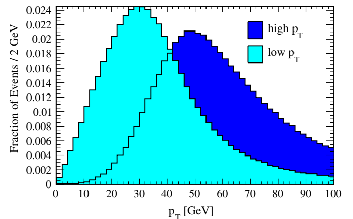
FIG. 8 (color online). The photon p_T distributions stemming from the decays \tilde{t} \rightarrow c\chi^0 \rightarrow c\gamma\tilde{G} of stops produced in pp \rightarrow \tilde{t}\tilde{t}^* at the LHC for m_{\tilde{t}} = 100 GeV. The light blue (lighter shaded) histogram corresponds to the photons with per event lower p_T .
