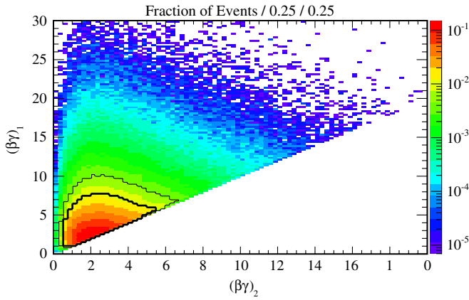
FIG. 1 (color online). The stop boost factors at the LHC in processes Eq. (4) for m_{\tilde{t}} = 100 GeV and m_{\tilde{g}} = 500 GeV. The thick (thin) contour contains 80% (90%) of the events.
