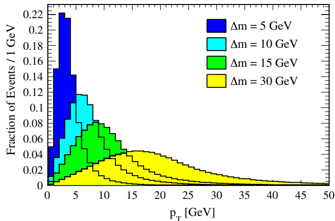
FIG. 9 (color online). The p_T distribution of the lower p_T charm quarks stemming from the decays of light stops produced in pp \rightarrow \tilde{t}\tilde{t}^* at the LHC for m_{\tilde{t}} = 100 GeV and different mass splittings \Delta m .
