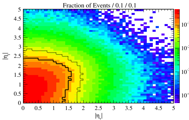
FIG. 2 (color online). The pseudorapidity distribution of the two stops at the LHC in processes Eq. (4) for m_{\tilde{t}} = 100 GeV and m_{\tilde{g}} = 500 GeV. In all shown events both stops satisfy \gamma\beta > 1 . The thick (thin) contour contains 80% (90%) of the events shown.
