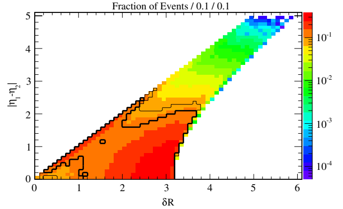
FIG. 3 (color online). The transverse separation |\eta_1 - \eta_2| versus \Delta R of the stops at the LHC in processes Eq. (4) for m_{\tilde{t}} = 100 GeV and m_{\tilde{g}} = 500 GeV. In all shown events the stops satisfy \gamma\beta > 1 and |\eta| < 2.5 . The thick (thin) contour contains 80% (90%) of the events shown.
