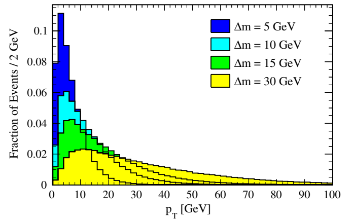
FIG. 6 (color online). The p_T distribution of the lower p_T charm quarks stemming from the decays of light stops produced in processes Eq. (4) for m_{\tilde{t}} = 100 GeV, m_{\tilde{g}} = 500 GeV, and different mass splittings \Delta m .
