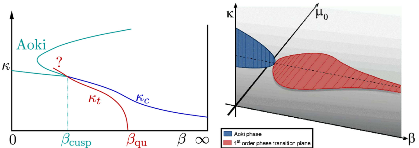
FIG. 1 (color online). Left: Aoki phase and thermal transition \kappa_t(\beta) for untwisted Wilson fermions. \beta_{\text{cusp}} denotes the tip of the Aoki phase and \beta_{\text{qu}} the critical coupling for the deconfinement transition in the quenched limit. Right: Aoki phase and first order bulk transition for twisted mass Wilson fermions at zero temperature [17].
