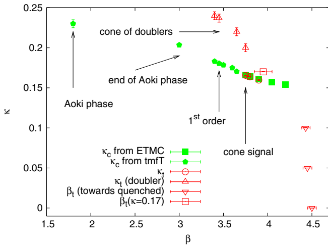
FIG. 15 (color online). Summary of numerically obtained transition points for 0 \leq \mu_0 \leq 0.007 . The data for \kappa_c(\beta) , \beta \geq 3.75 are taken from [24,61].
