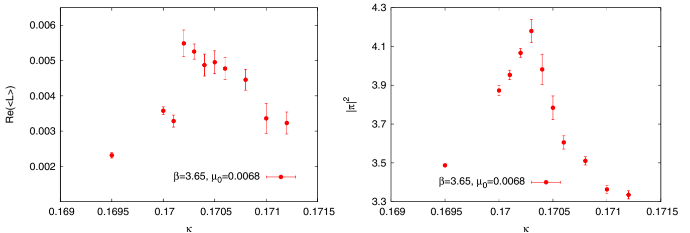
FIG. 5 (color online). Real part of the Polyakov loop (left) and the pion norm (right) around \kappa_c at \beta = 3.65 and \mu_0 = 0.0068 .
