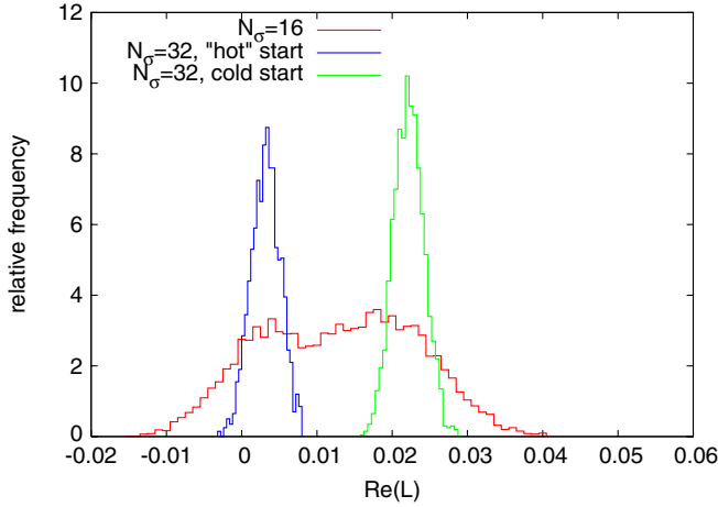
FIG. 12 (color online). Distributions of \text{Re}(L) for \beta = 3.6 , \mu_0 = 0 , and \kappa = 0.22 .
