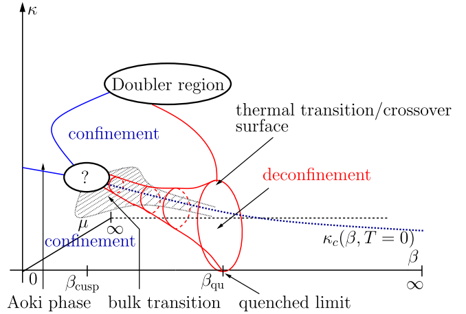
FIG. 2 (color online). Schematic view of Creutz's cone conjecture, derived from [56].
