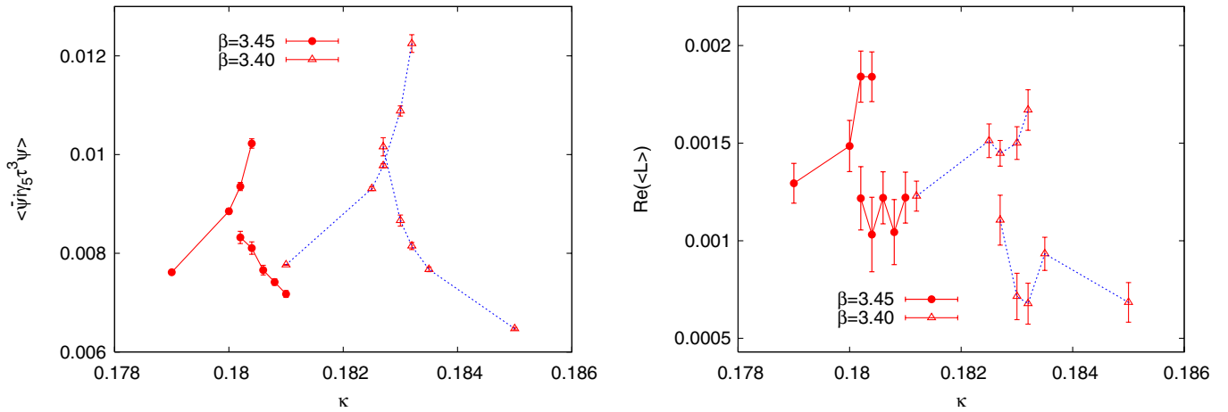
FIG. 4 (color online). Metastability signals in the order parameter \langle \bar{\psi} i \gamma_5 \tau^3 \psi \rangle (left) and the Polyakov loop (right) in the neighborhood of the critical line, \mu_0 \approx 0.0068 . The lines were added for visual guidance.
