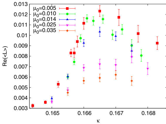
FIG. 13 (color online). Left: Polyakov loop expectation value for different values of \mu_0 . For \mu_0 \geq 0.025 , the transitions are lost. Right: Data points represent the phase boundary at \beta = 3.75 , estimated from the peaks of susceptibilities. The leading order part of Eq. (11) does not fit the data; the NLO formula contains undetermined constants that have been estimated by order of magnitude only. The vertical line marks \kappa_c(\beta = 3.75) , i.e. maximal twist.
