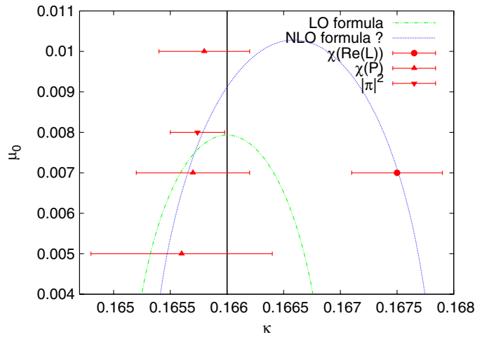
FIG. 13 (color online). Left: Polyakov loop expectation value for different values of \mu_0 . For \mu_0 \geq 0.025 , the transitions are lost. Right: Data points represent the phase boundary at \beta = 3.75 , estimated from the peaks of susceptibilities. The leading order part of Eq. (11) does not fit the data; the NLO formula contains undetermined constants that have been estimated by order of magnitude only. The vertical line marks \kappa_c(\beta = 3.75) , i.e. maximal twist.
