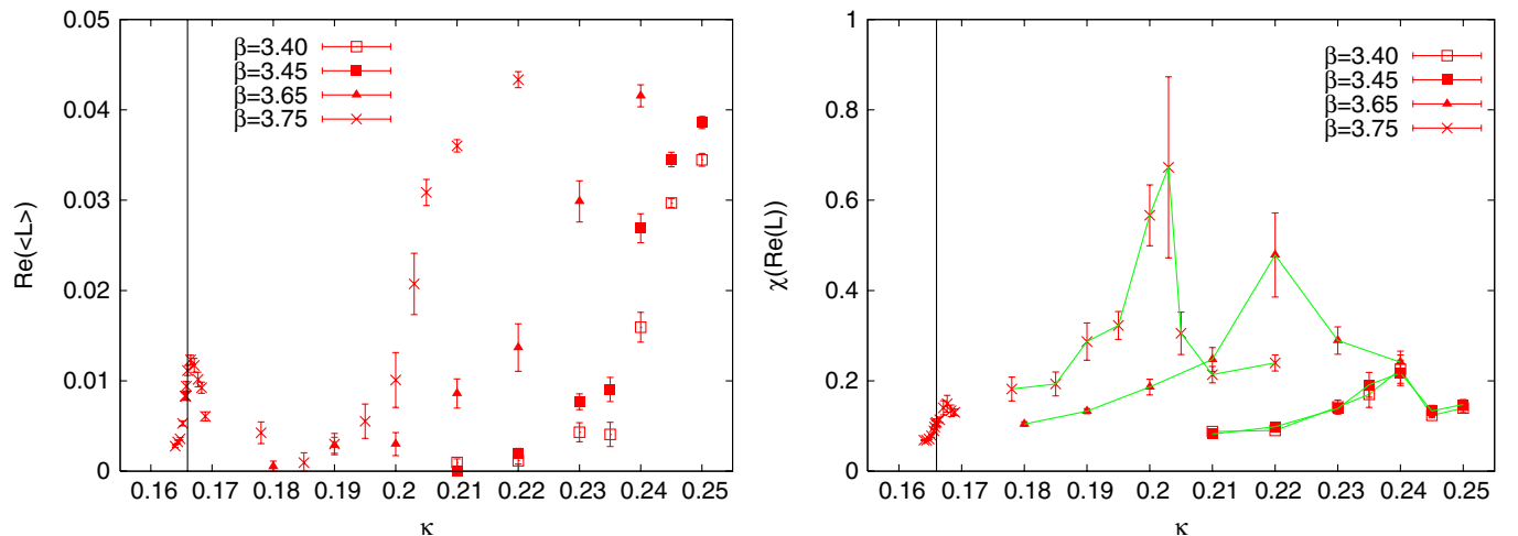
FIG. 11 (color online). Real part of the Polyakov loop (left) and its susceptibility (right) for \beta = 3.4, 3.45, 3.65 with \mu_0 = 0.0068 and \beta = 3.75 with \mu_0 = 0.005 . The vertical line marks \kappa_c(\beta = 3.75) . Lines on the right are added for visual guidance.
