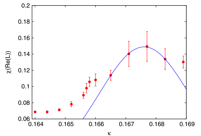
FIG. 14 (color online). Pion norm (left) and Polyakov loop susceptibility (right) showing two subsequent transitions at \beta = 3.75 , \mu_0 = 0.005 .
