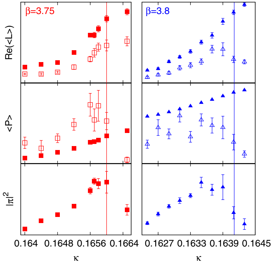
FIG. 9 (color online). Real part of Polyakov loop (top panel), plaquette (middle panel), and pion norm (bottom) near \kappa_c (marked by vertical lines). For the first two observables expectation value (filled points) and susceptibility (open) are shown.
