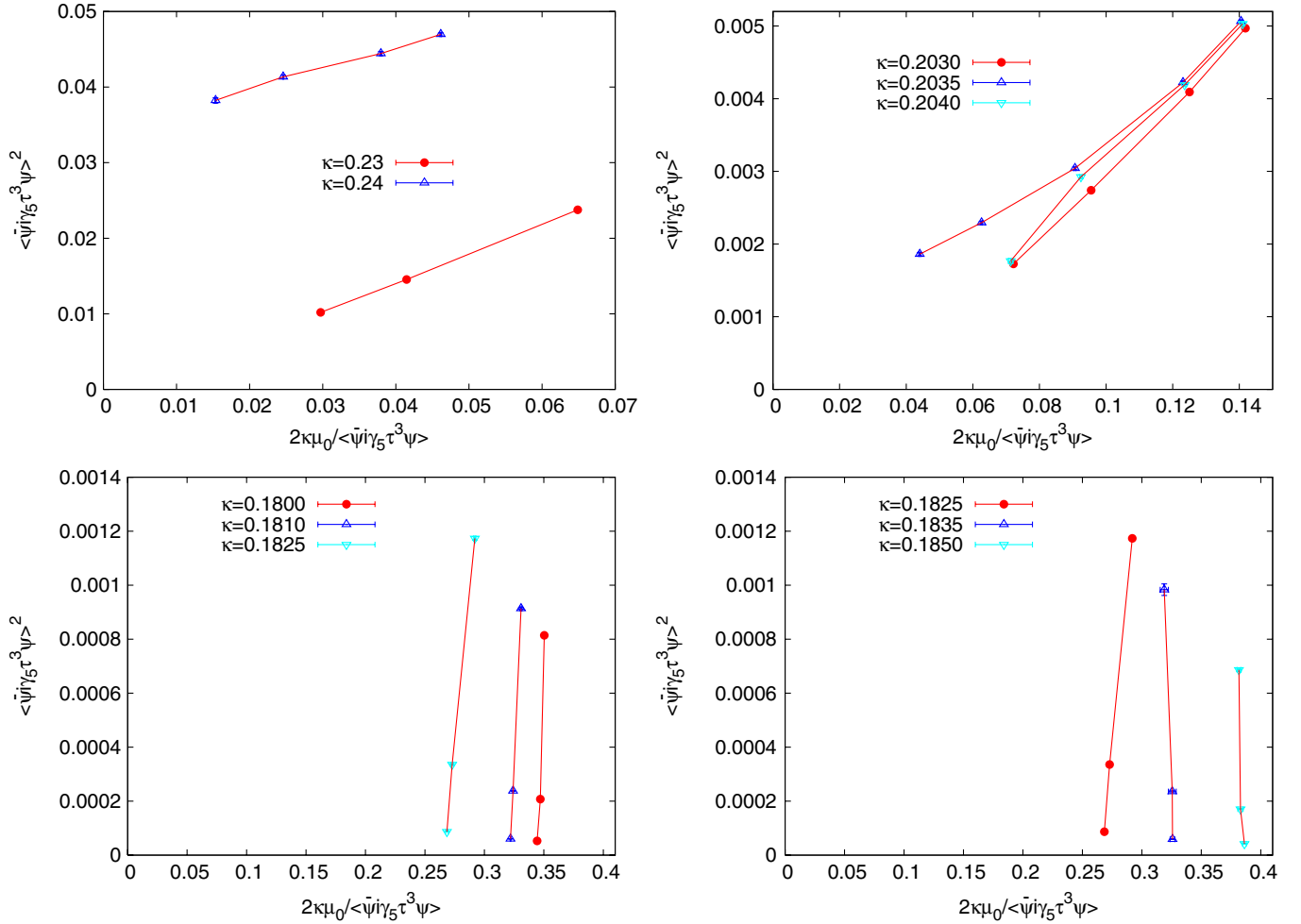
FIG. 3 (color online). Fisher plots for \beta = 1.8 (upper left panel), \beta = 3.0 (upper right panel) and \beta = 3.4 (lower panels) for \kappa < \kappa_c \approx 0.1825 (left) and \kappa > \kappa_c (right).
