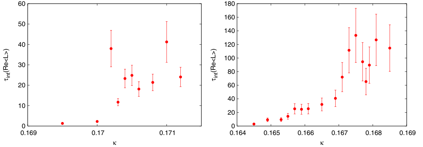
FIG. 6 (color online). Integrated autocorrelation time for \text{Re}(L) as a function of \kappa for \beta = 3.65 , \mu_0 = 0.0068 (left) and \beta = 3.75 , \mu_0 = 0.0070 (right).
