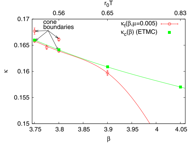
FIG. 16 (color online). The region \beta \geq 3.75 . The lines are splines to guide the eye where the quenched and zero coupling limits have been taken into account.
