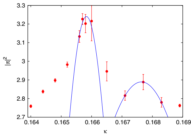
FIG. 14 (color online). Pion norm (left) and Polyakov loop susceptibility (right) showing two subsequent transitions at \beta = 3.75 , \mu_0 = 0.005 .
