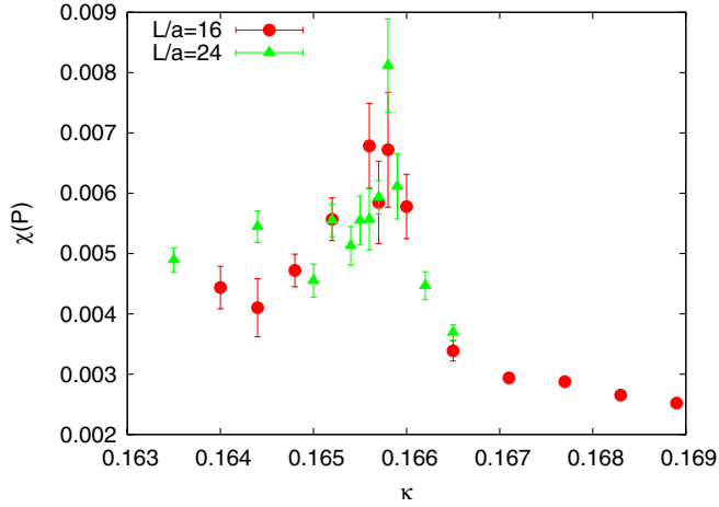
FIG. 10 (color online). Finite size scaling test for the plaquette susceptibility at \beta = 3.75 and \mu_0 = 0.005 .
