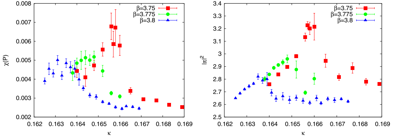
FIG. 8 (color online). Plaquette susceptibility (left) and pion norm (right) for \beta = 3.75, 3.775, 3.8 and \mu_0 = 0.005 .
