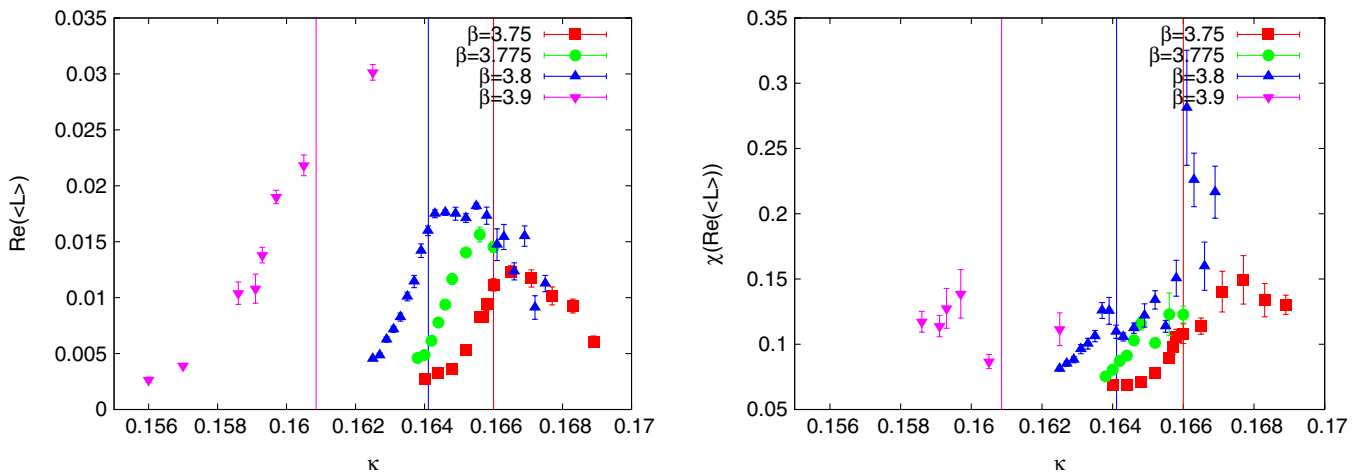
FIG. 7 (color online). The real part of the Polyakov loop (left) and its susceptibility (right) for \beta = 3.75, 3.775, 3.8, 3.9 and \mu_0 = 0.005 . The vertical lines mark \kappa_c(T = 0, \beta) for \beta = 3.9, 3.8, 3.75 from left to right.
