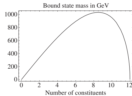
FIG. 1. Mass spectrum of bound states.
