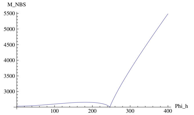
FIG. 3 (color online). Energy or mass of the bound state in GeV in our toy model as a function of the imposed \phi_h value, but with p_f adjusted by minimization. The top-quark Yukawa coupling is chosen to have the phase transition value g_t = 1.191 .
