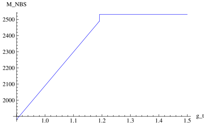
FIG. 2 (color online). Energy or mass of the “bound state” in GeV in our toy model as a function of the top-quark Yukawa coupling g_t .
