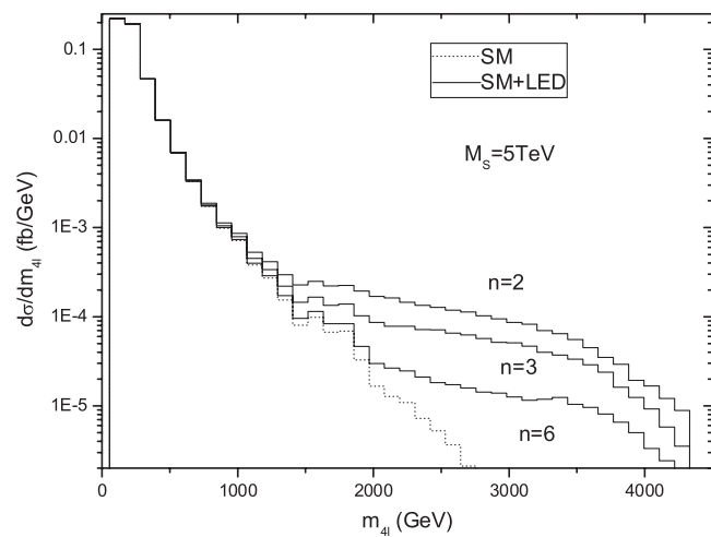
FIG. 3. The invariant mass distributions of the four leptons.
