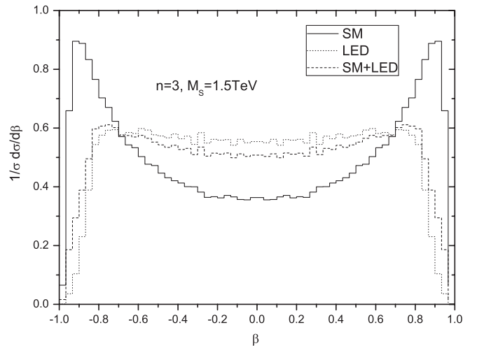
FIG. 5. The normalized velocity distributions of the rest frame of the Z pair.
