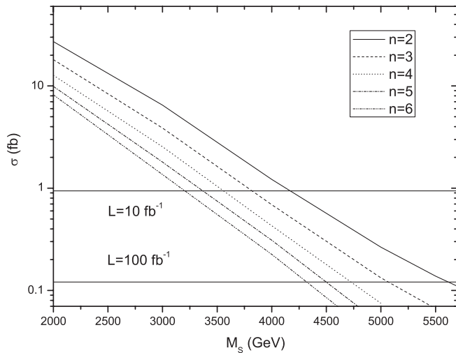
FIG. 7. The total cross sections of the LED signals after all the cuts as functions of M_S . The horizontal lines indicate the cross sections needed for a 3\sigma detection of the signal.
