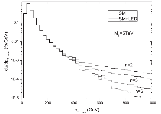
FIG. 4. The transverse momentum distributions of the leading lepton.
