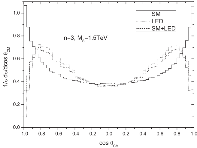
FIG. 6. The normalized polar angle distributions of the reconstructed Z boson in the rest frame of the Z pair.
