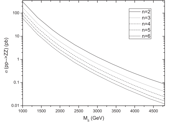
FIG. 2. The total cross sections of the Z boson pair production from LED contributions as functions of M_S at the LHC.
