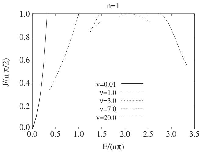
FIG. 6. Angular momentum per vortex number J/n versus energy per vortex number E/n for solutions with n = 1 and several values of \nu .
