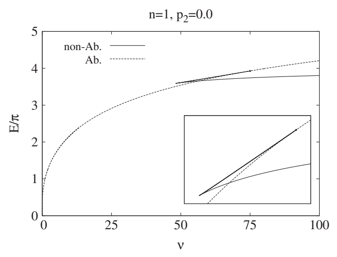
FIG. 8. Energy E versus the Higgs self-coupling parameter \nu for p_2 = 0 solutions with n = 1 . For a range of \nu , the non-Abelian solutions have a lower energy than their Abelian counterparts.
